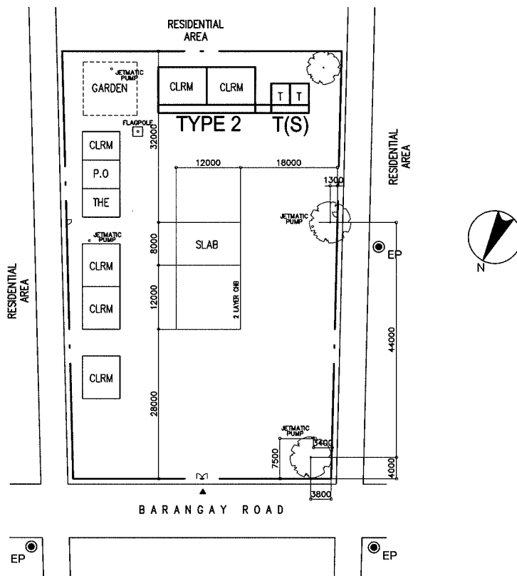
PROPOSED SITE PLAN SCALE 1:1000M
