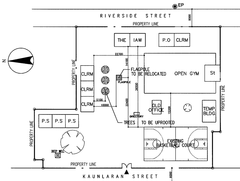
EXISTING SITE PLAN SCALE 1:1000M
