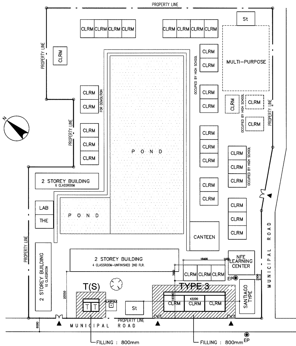
PROPOSED SITE PLAN SCALE 1:1000M
