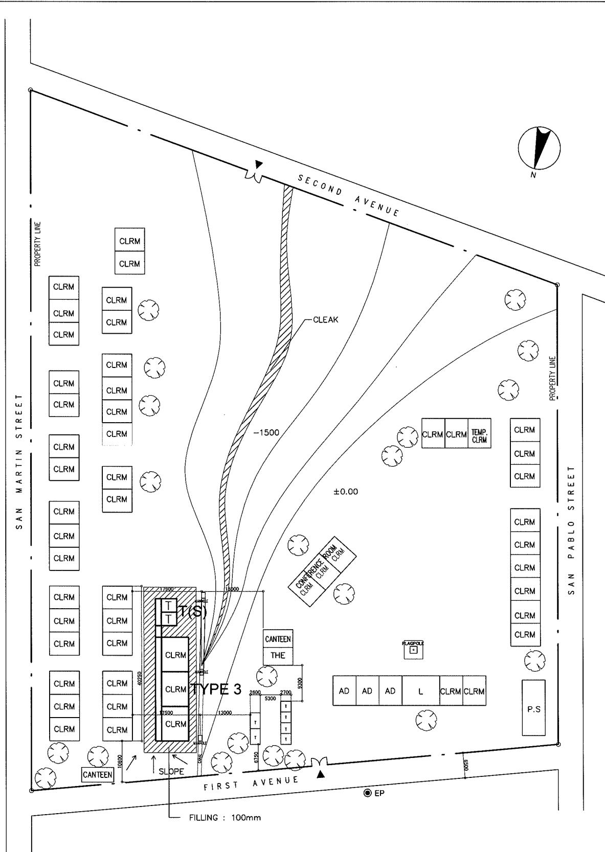
PROPOSED SITE PLAN SCALE 1:1000M
