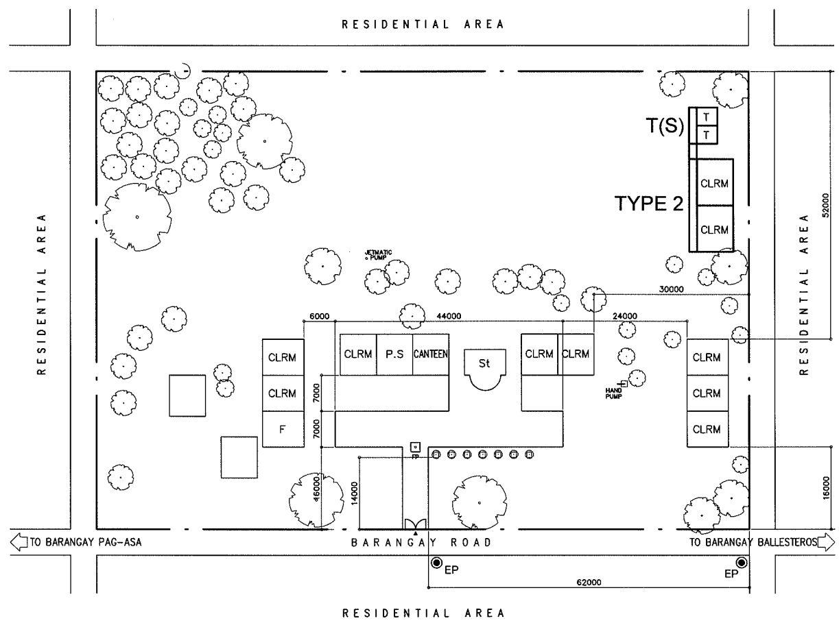
PROPOSED SITE PLAN SCALE 1:1000M
