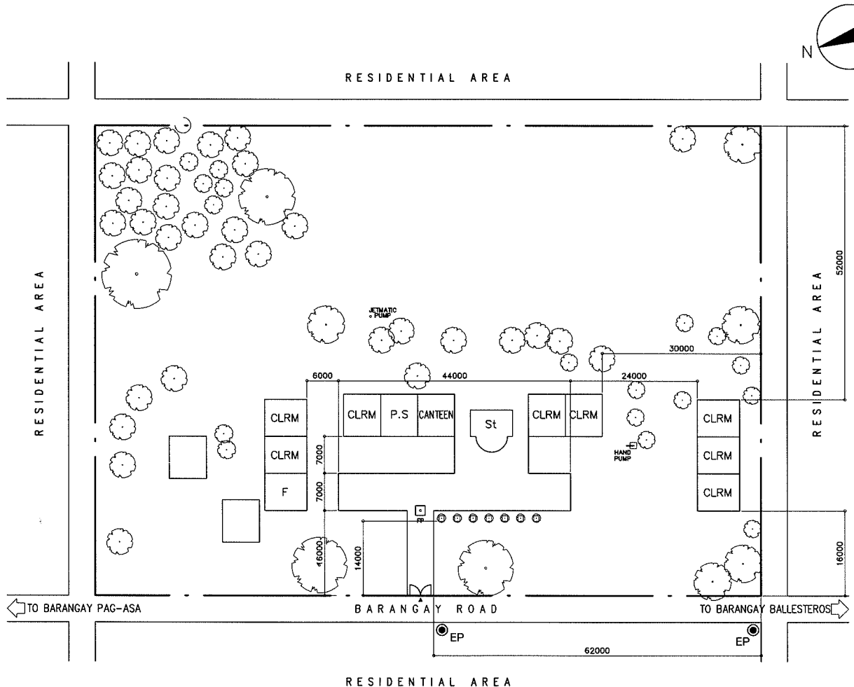
EXISTING SITE PLAN SCALE 1:1000M
