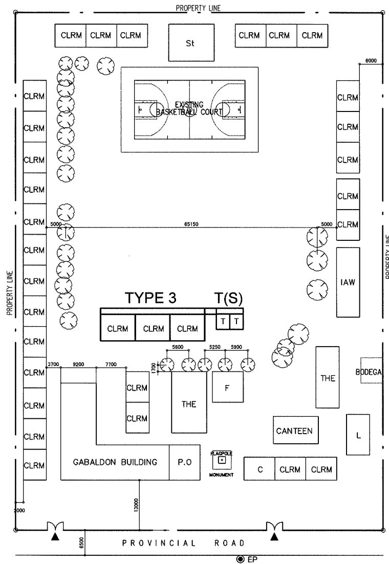
PROPOSED SITE PLAN SCALE 1:1000M
