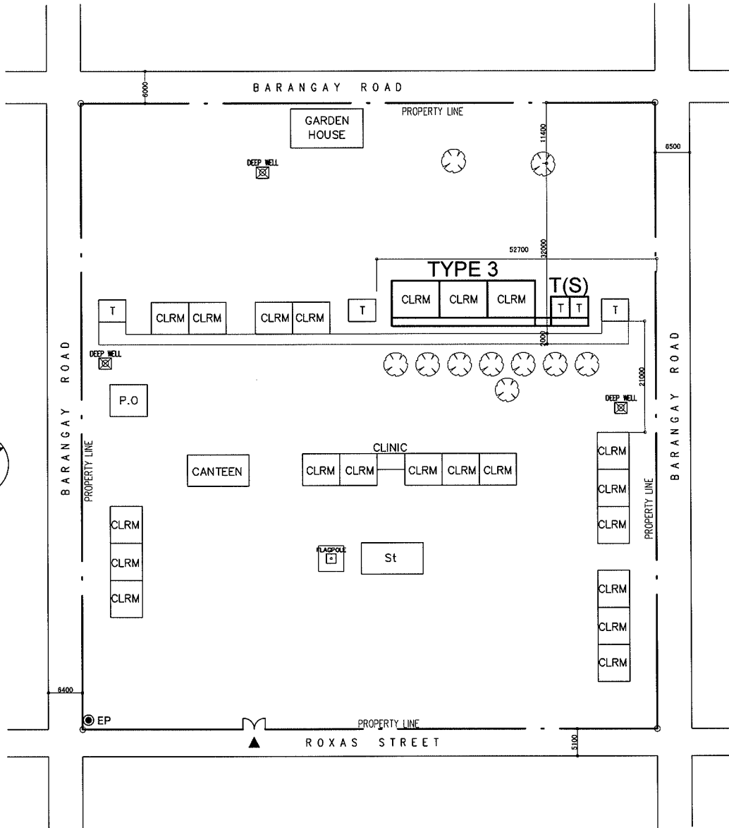
PROPOSED SITE PLAN SCALE 1:1000M
