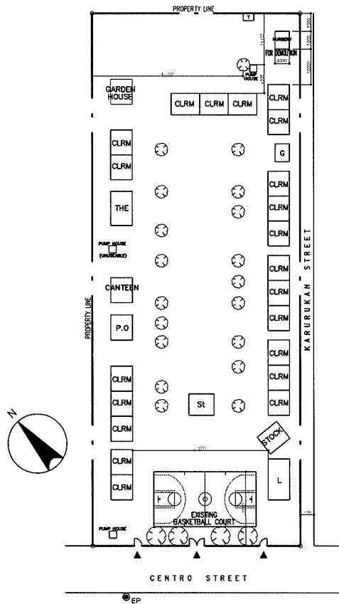
EXISTING SITE PLAN SCALE 1:1500M
