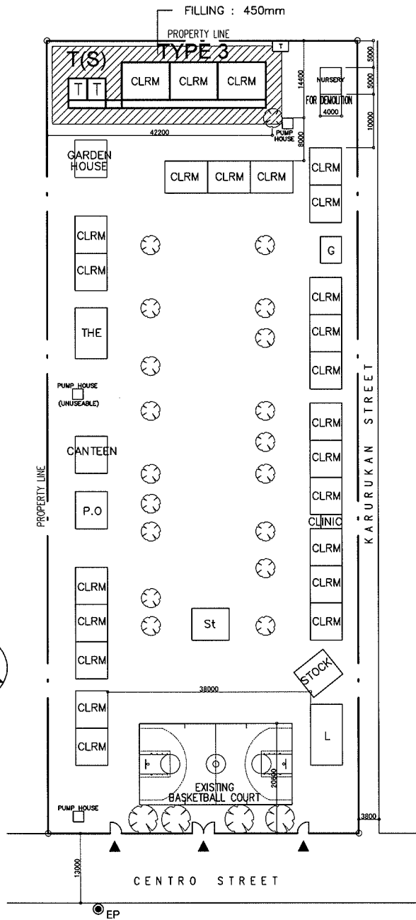
PROPOSED SITE PLAN SCALE 1:1000M
