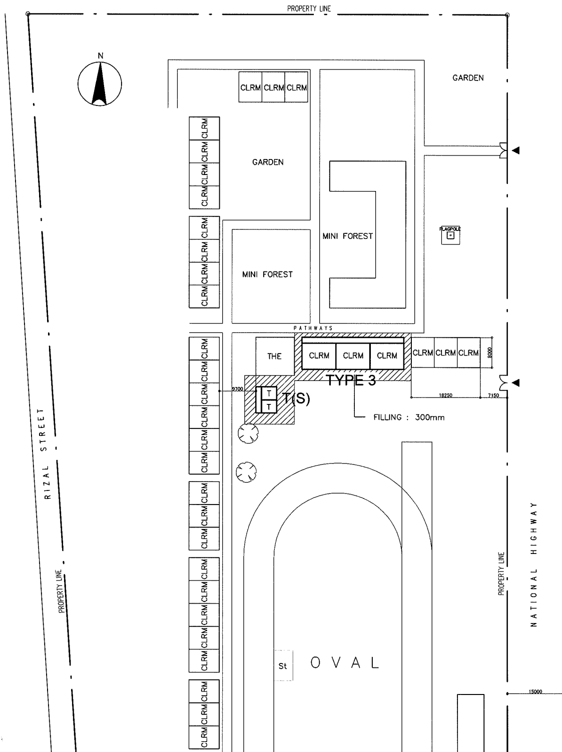
PROPOSED SITE PLAN SCALE 1:1000M
