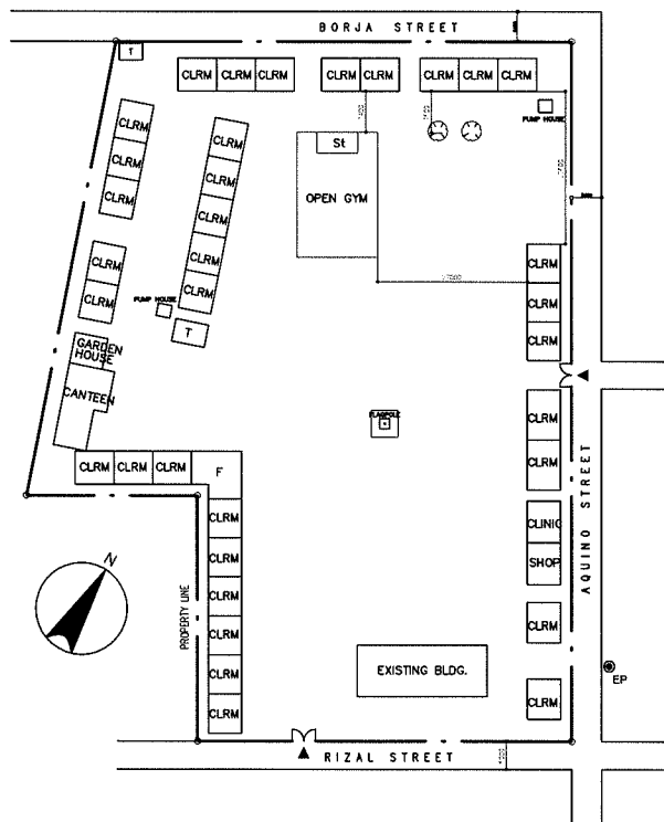
EXISTING SITE PLAN SCALE 1:1500M
