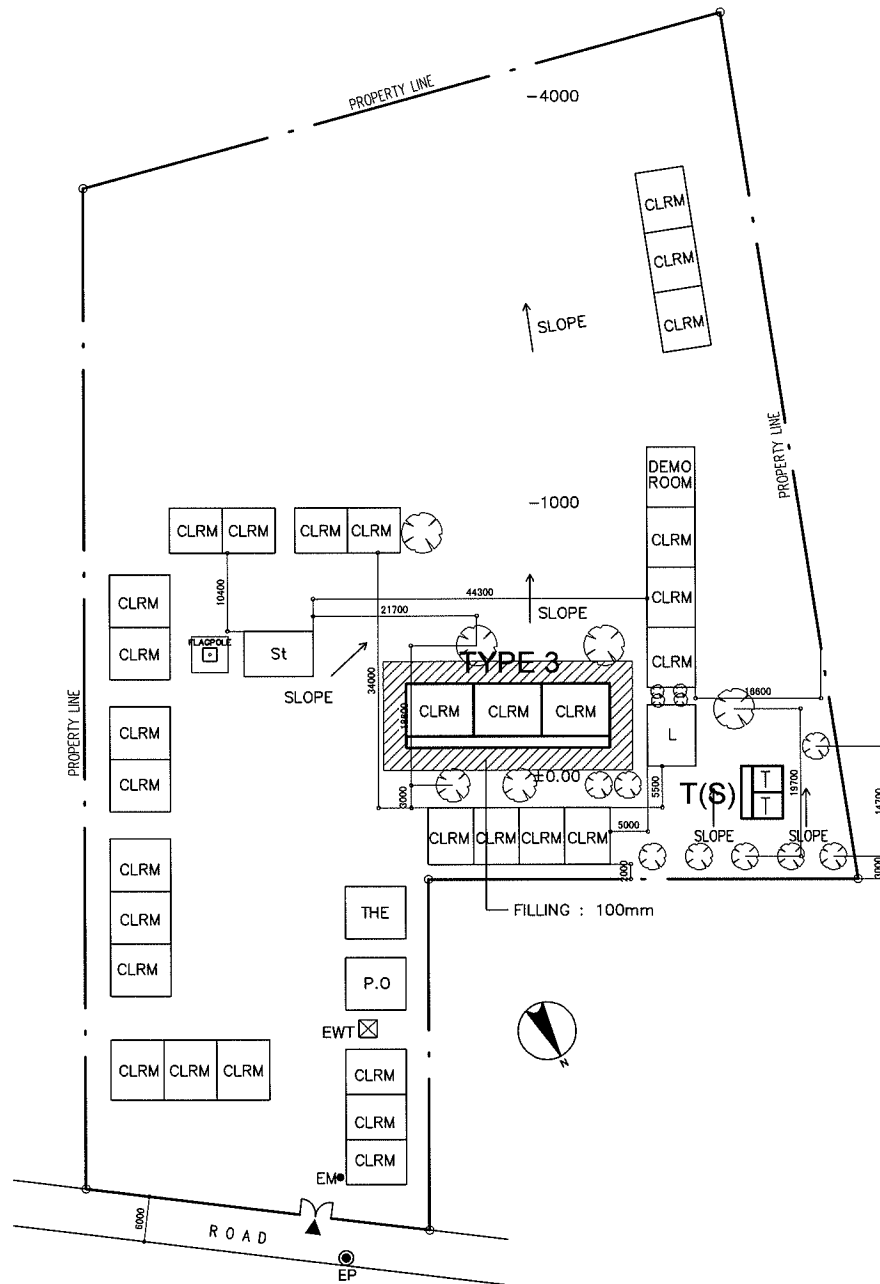
PROPOSED SITE PLAN SCALE 1:1000M
