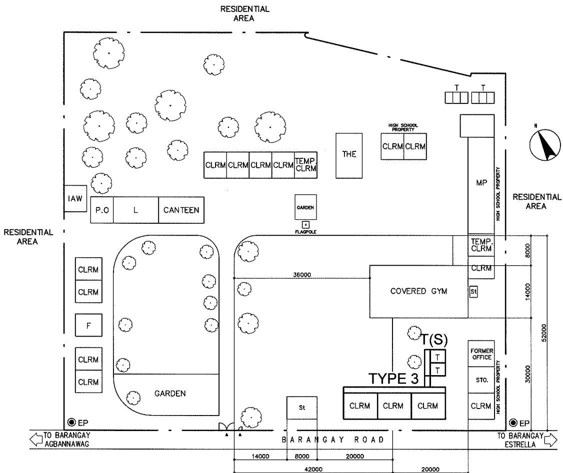
PROPOSED SITE PLAN SCALE 1:1000M
