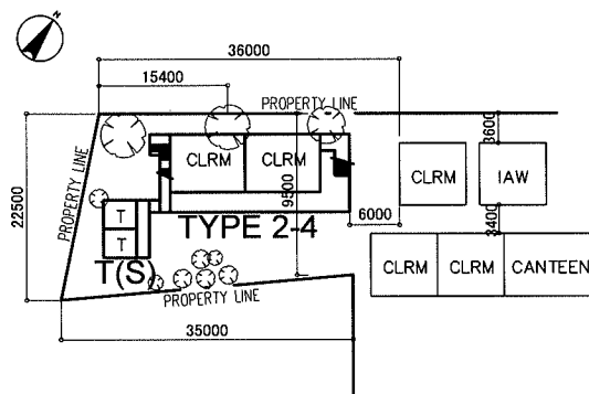
PROPOSED SITE PLAN SCALE 1:1000M
