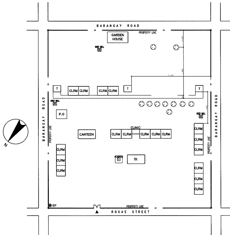
EXISTING SITE PLAN SCALE 1:1500M
