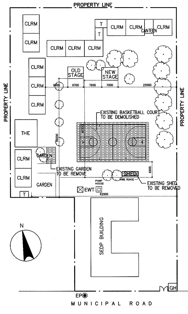
EXISTING SITE PLAN SCALE 1:1000M
