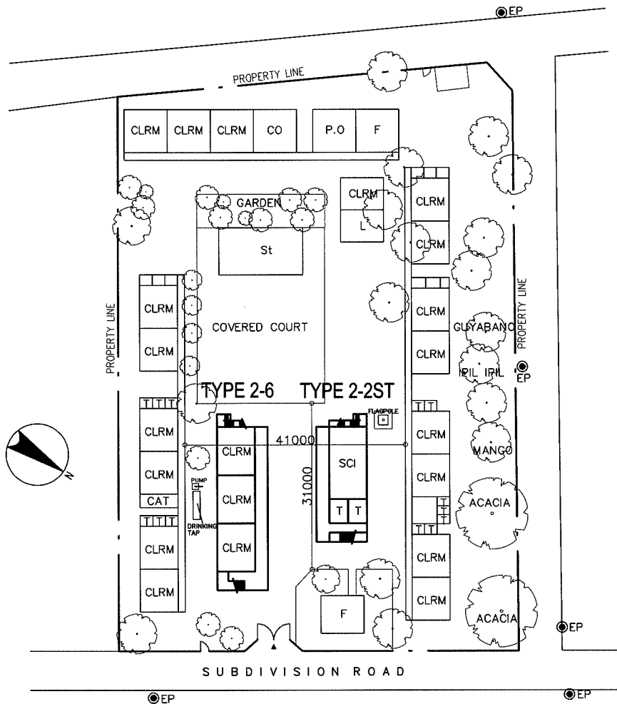
PROPOSED SITE PLAN SCALE 1:1000M
