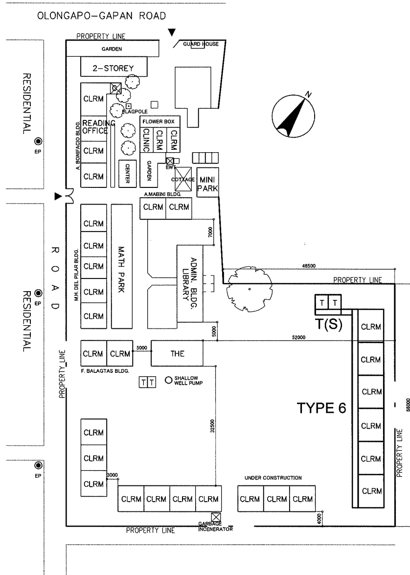
PROPOSED SITE PLAN SCALE 1:1000M
