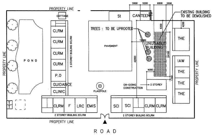
EXISTING SITE PLAN SCALE 1:1000M
