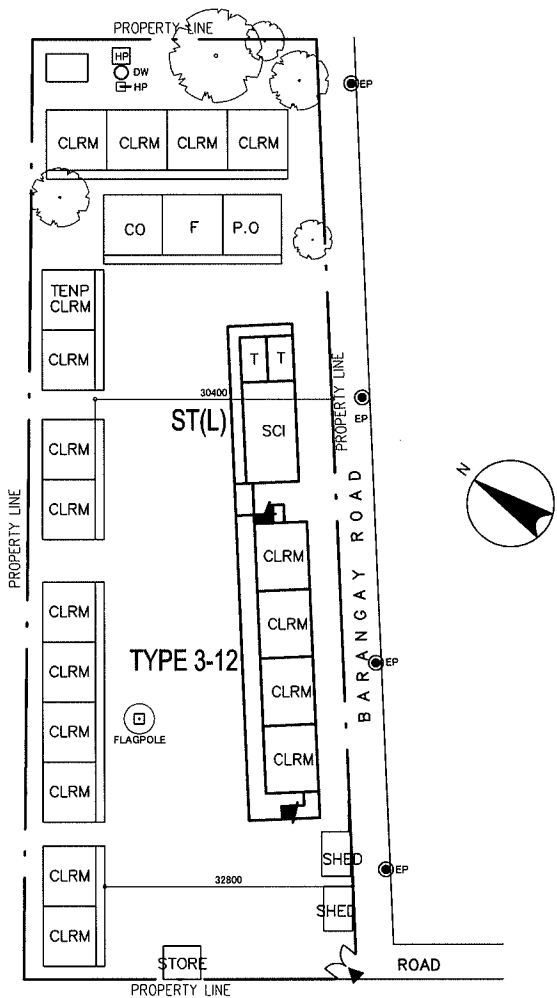
PROPOSED SITE PLAN SCALE 1:1000M
