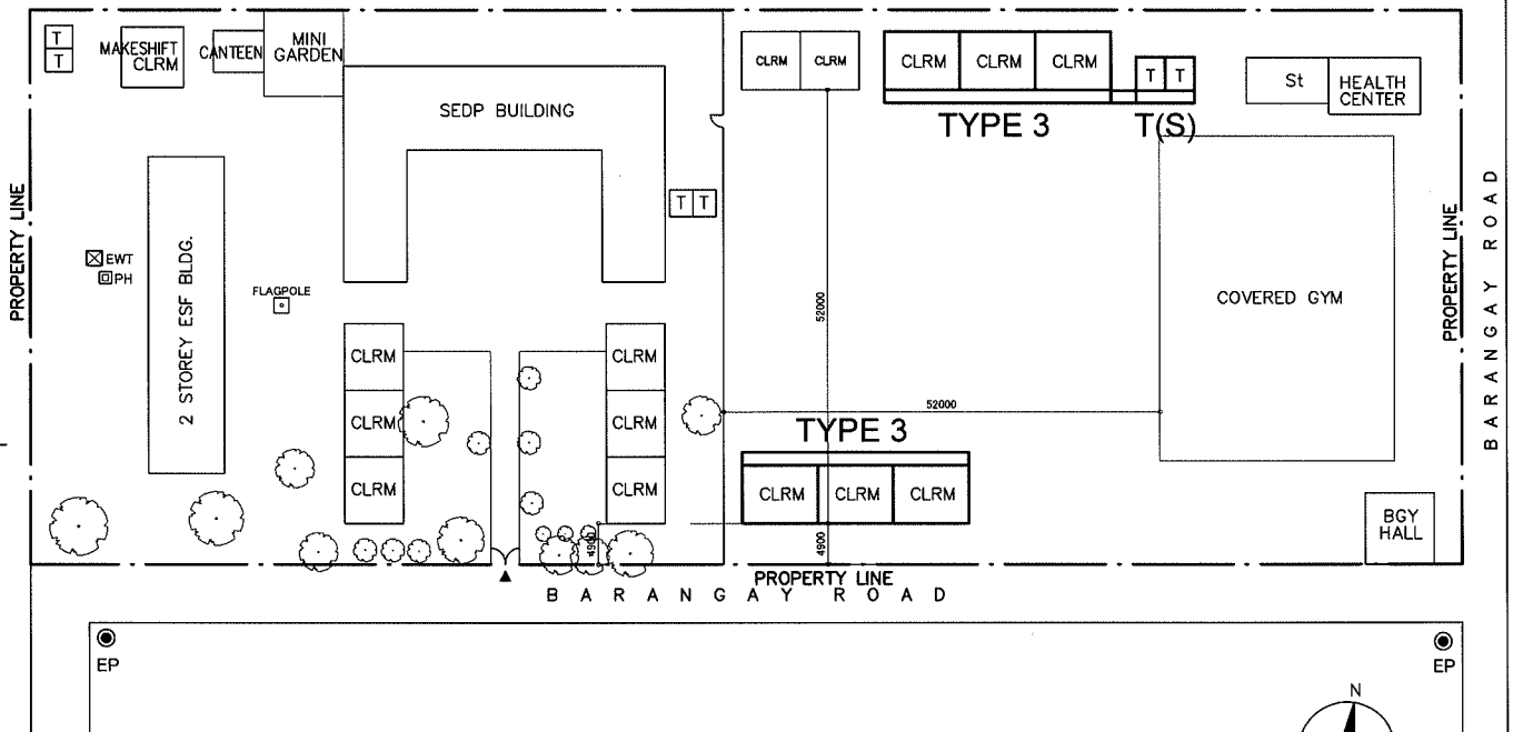
PROPOSED SITE PLAN SCALE 1:1000M
