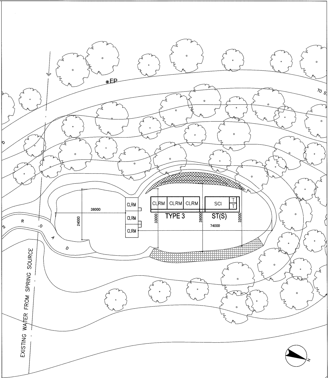
PROPOSED SITE PLAN SCALE 1:1000M
