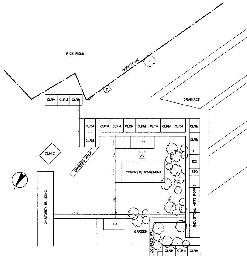
EXISTING SITE PLAN SCALE 1:1500M
