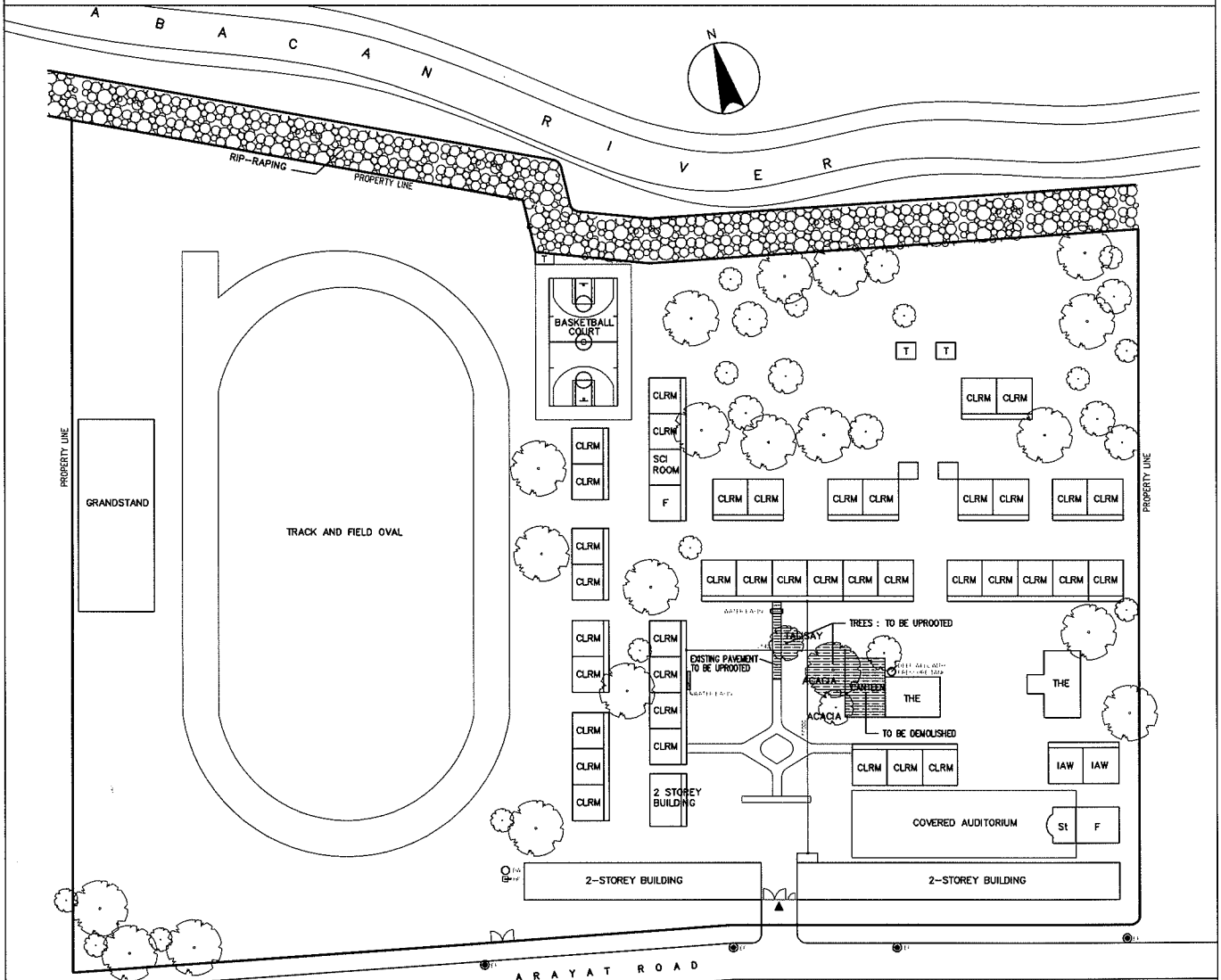
EXISTING SITE PLAN SCALE 1:1500M
