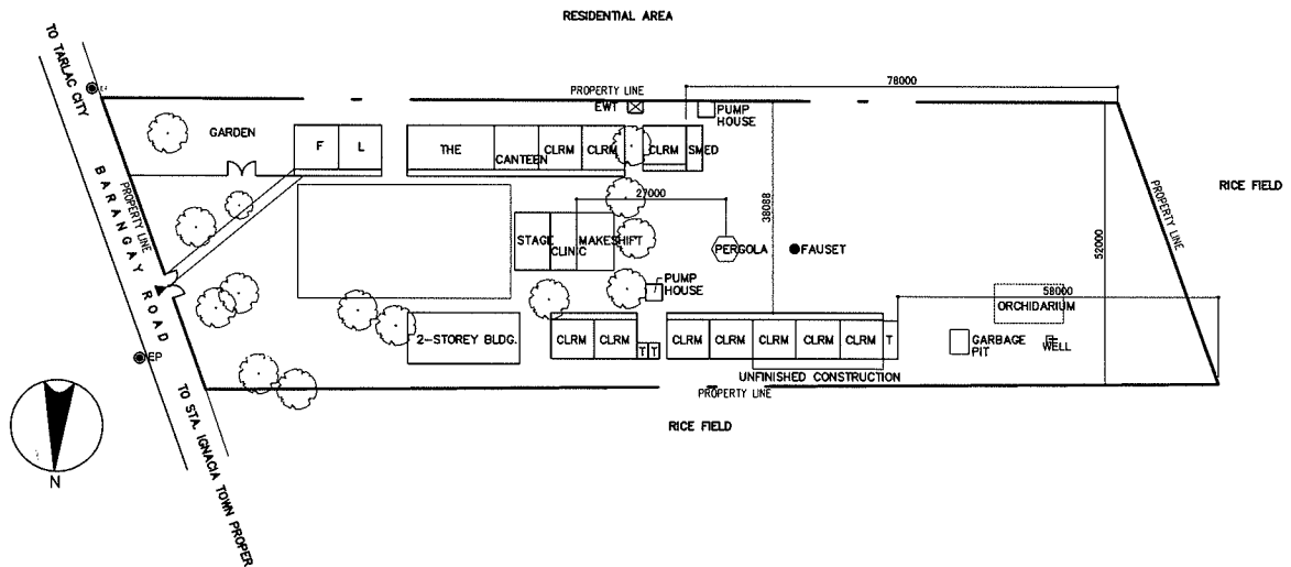
EXISTING SITE PLAN SCALE 1:1500M
