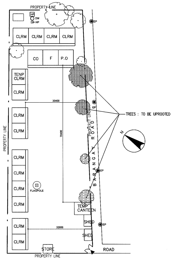
EXISTING SITE PLAN SCALE 1:1000M
