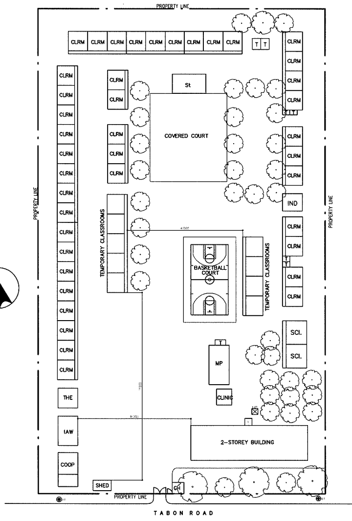
EXISTING SITE PLAN SCALE 1:1500M
