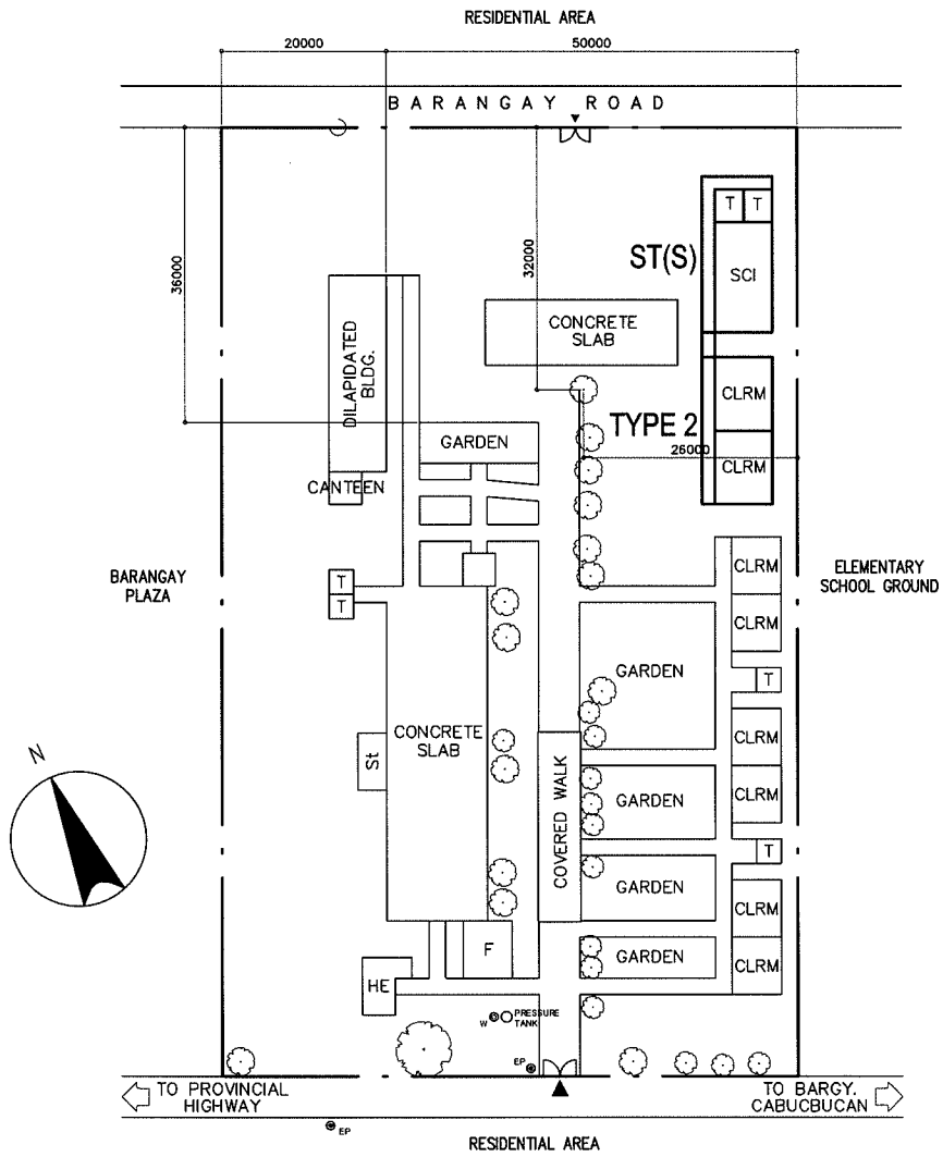
PROPOSED SITE PLAN SCALE 1:1000M
