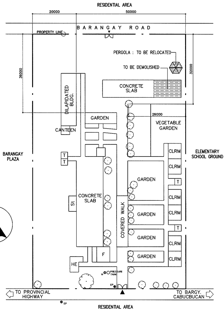
EXISTING SITE PLAN SCALE 1:1000M
