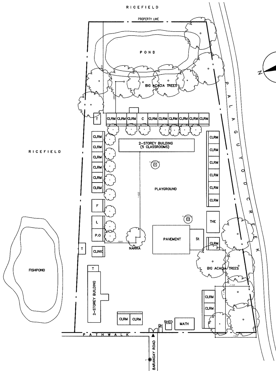
EXISTING SITE PLAN SCALE 1:1500M
