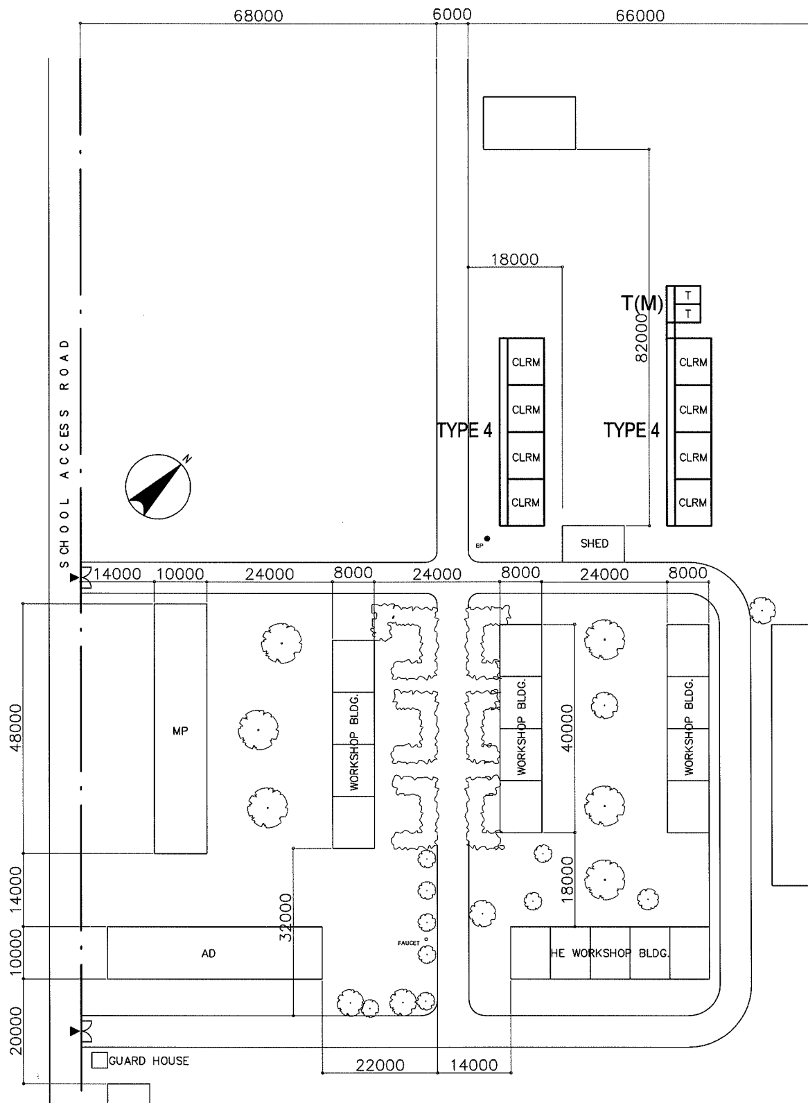
PROPOSED SITE PLAN SCALE 1:1000M
