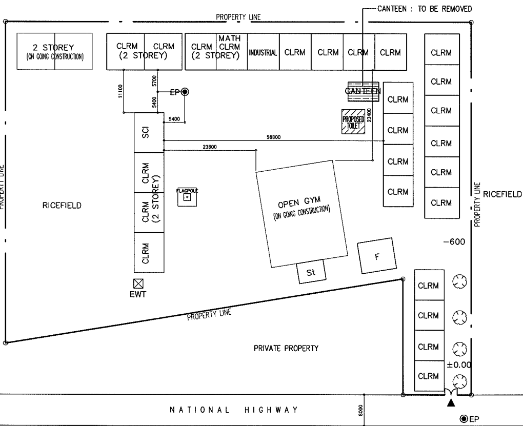
EXISTING SITE PLAN SCALE _____ 1:1000M
