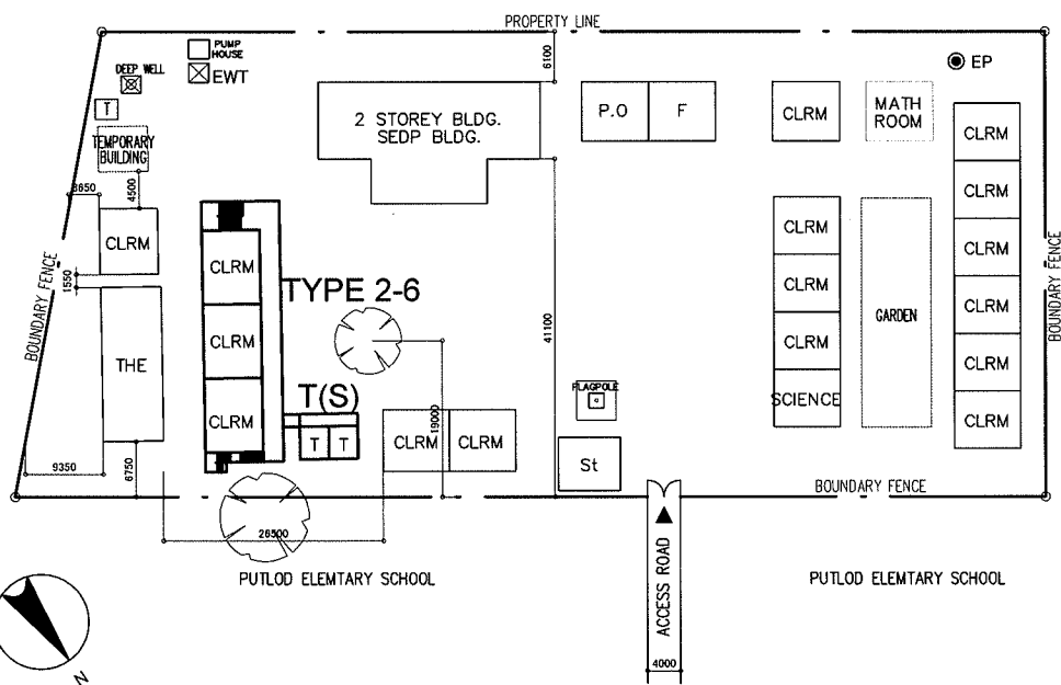
PROPOSED SITE PLAN SCALE 1:1000M
