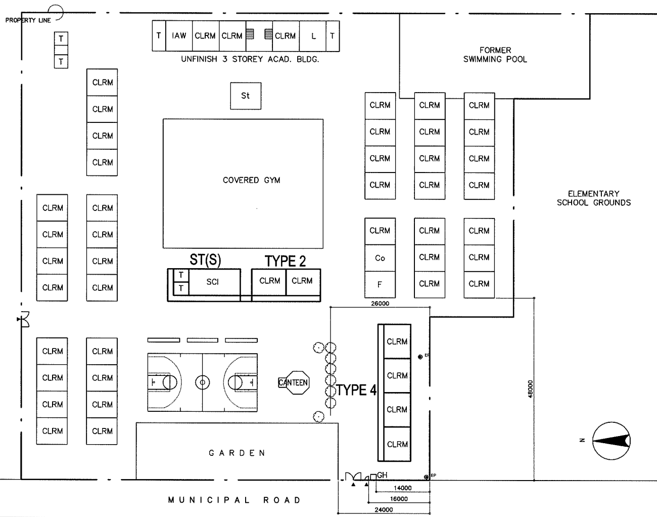
PROPOSED SITE PLAN SCALE 1:1000M
