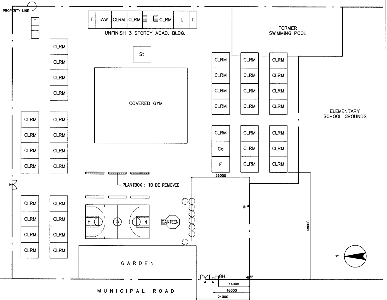
EXISTING SITE PLAN SCALE 1:1000M
