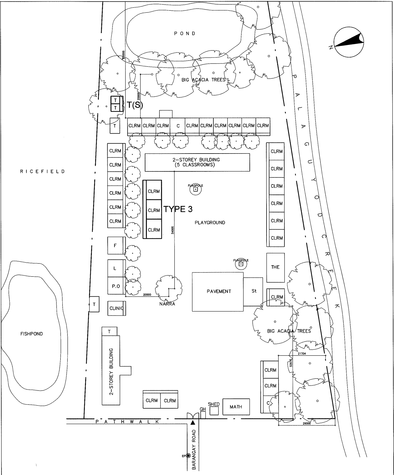
PROPOSED SITE PLAN SCALE 1:1000M
