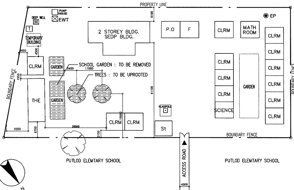
EXISTING SITE PLAN SCALE 1:1000M
