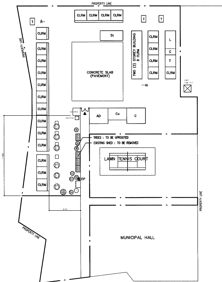
EXISTING SITE PLAN SCALE 1:1500M
