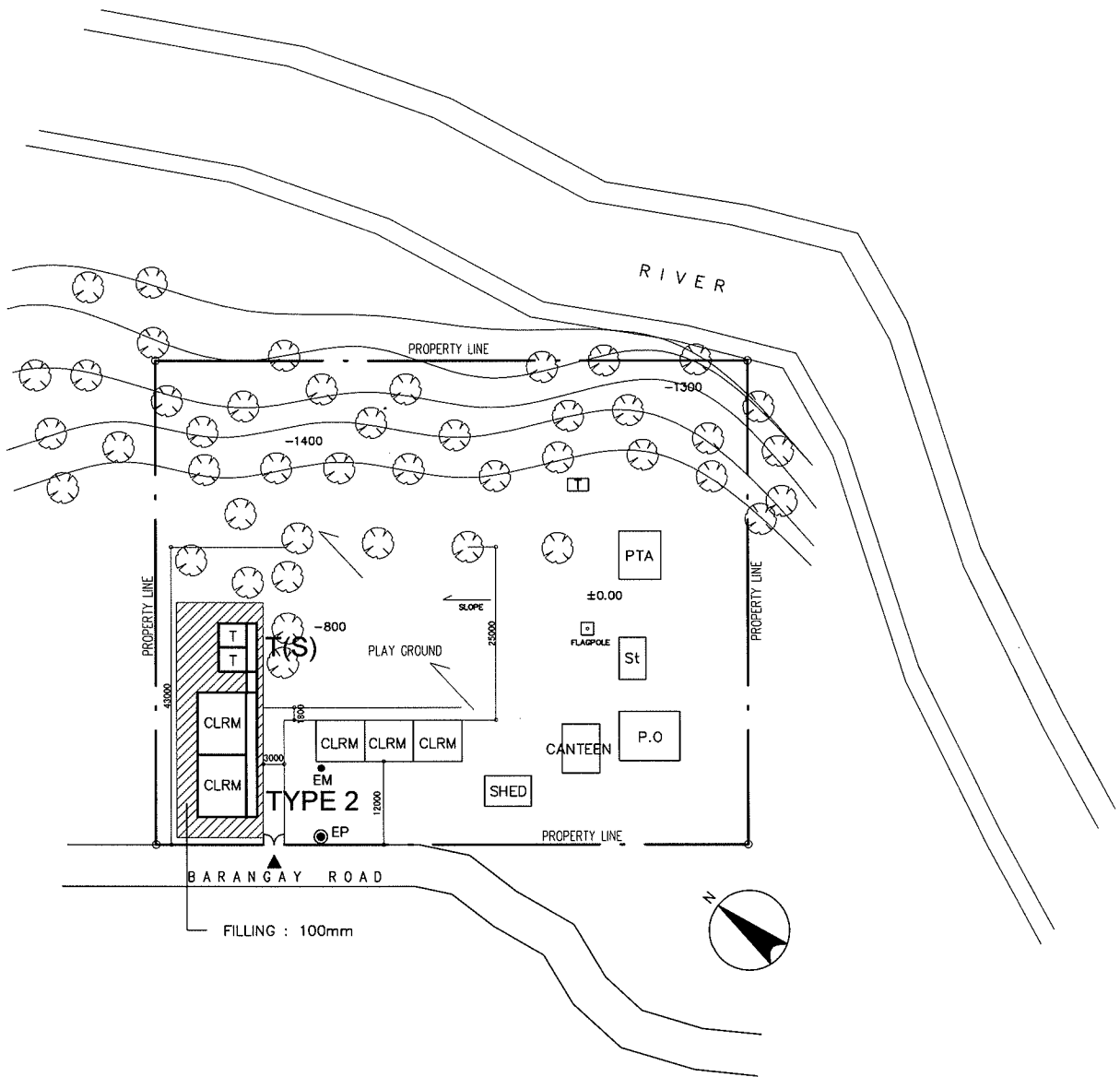
PROPOSED SITE PLAN SCALE 1:1000M
