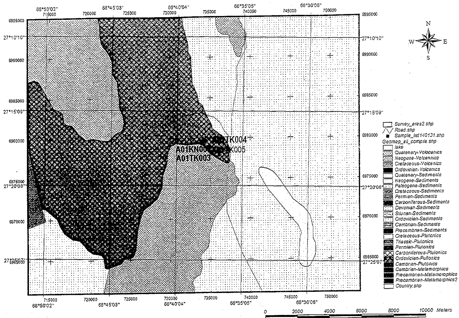
Fig.A-1-28 Sample point of Lagna Blanca alteration zone
