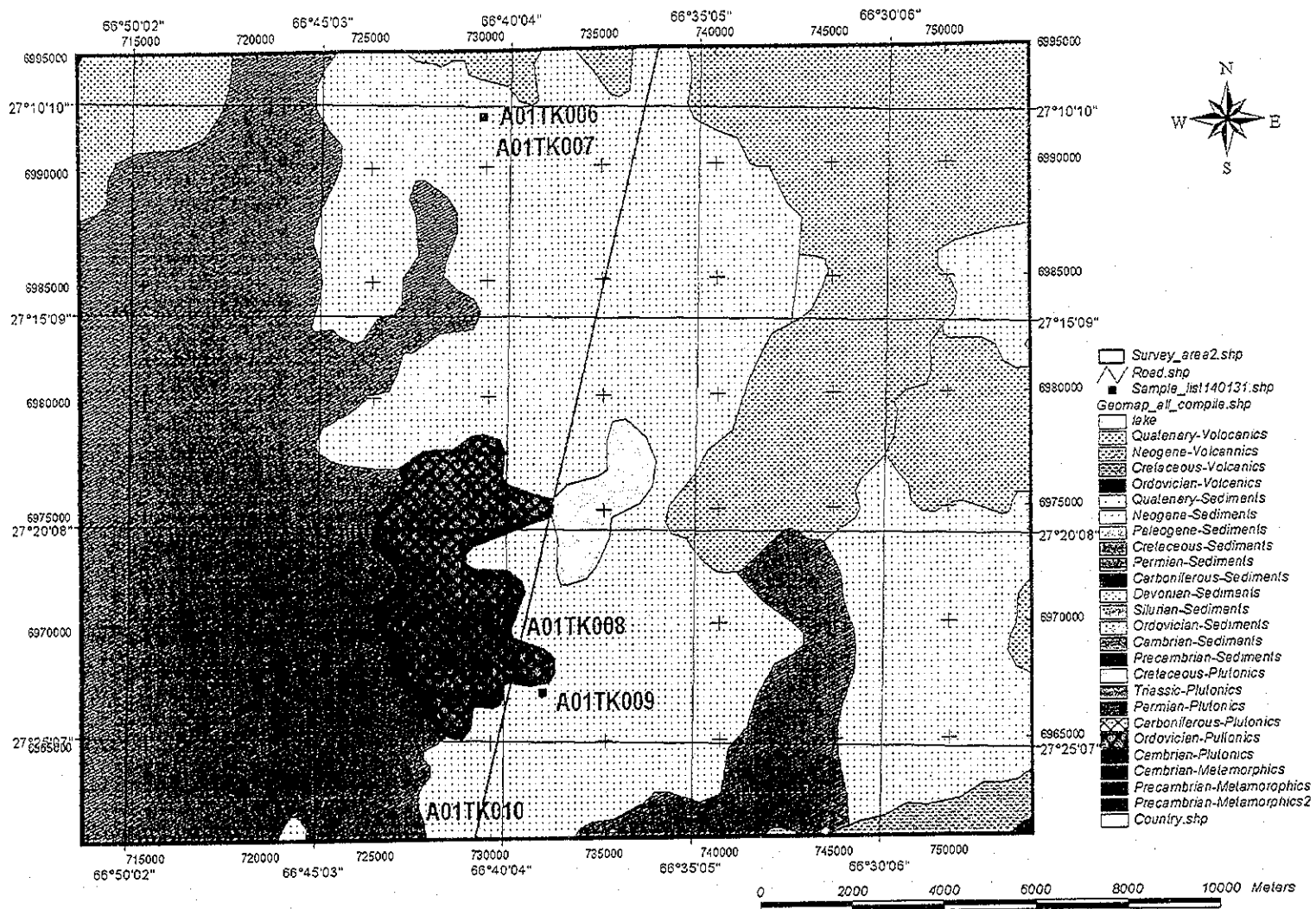
Fig.A-1-26 Sample point of Laguna Grande alteration zone
