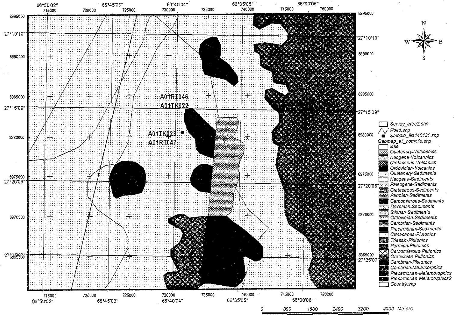
Sample point of Inca Viejo mineral showing
