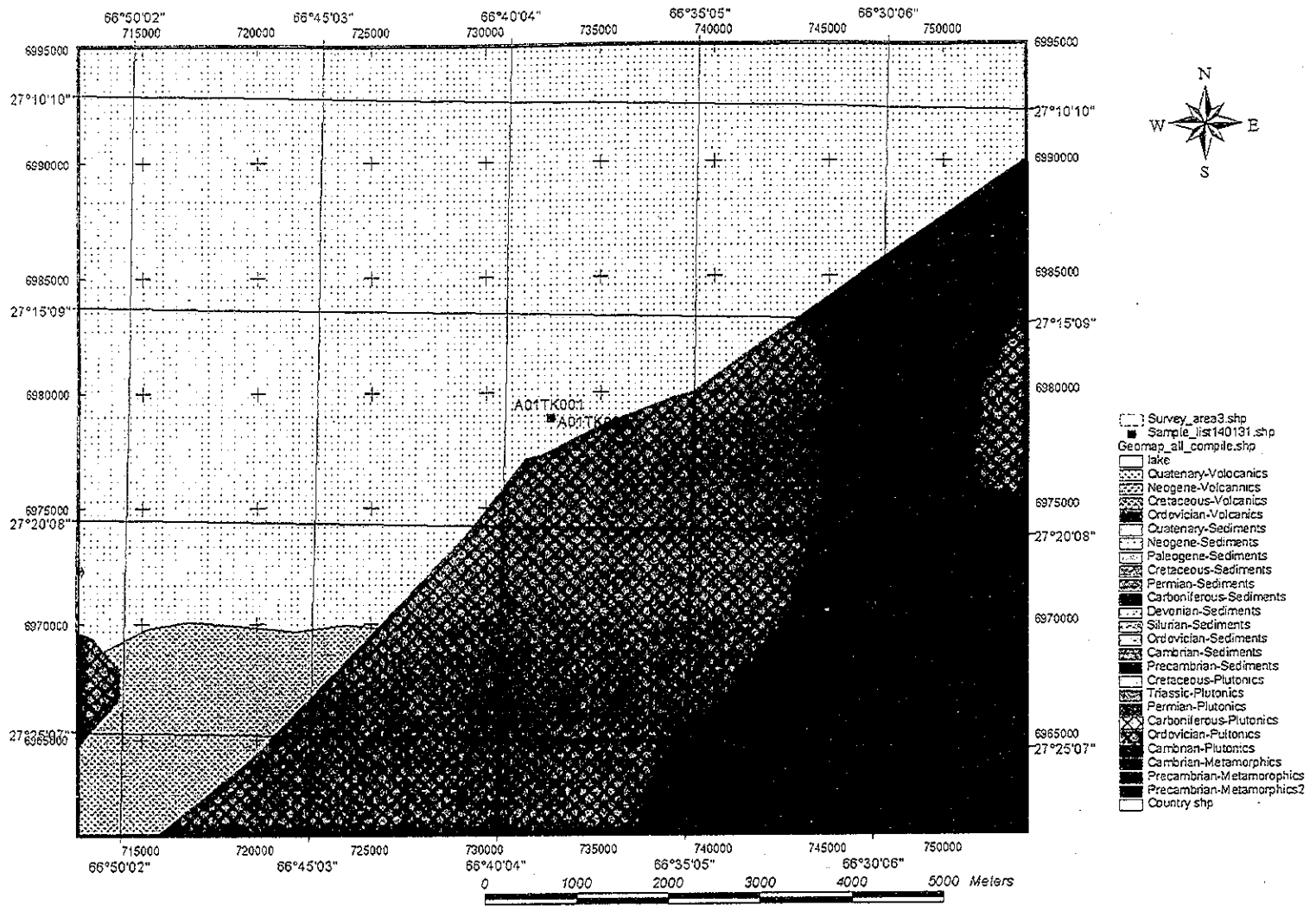
Fig.A-1-34 Sample point of Capillitas NE alteration zone
