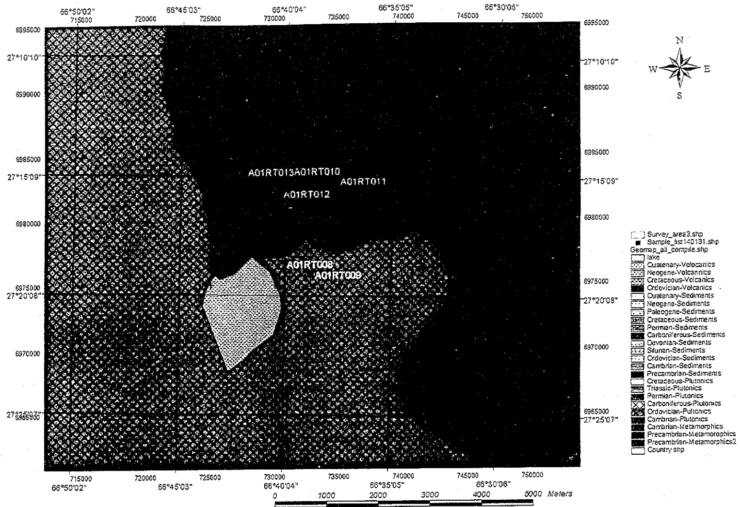
Fig.A-1-32 Sample point of Agua Rica deposit
