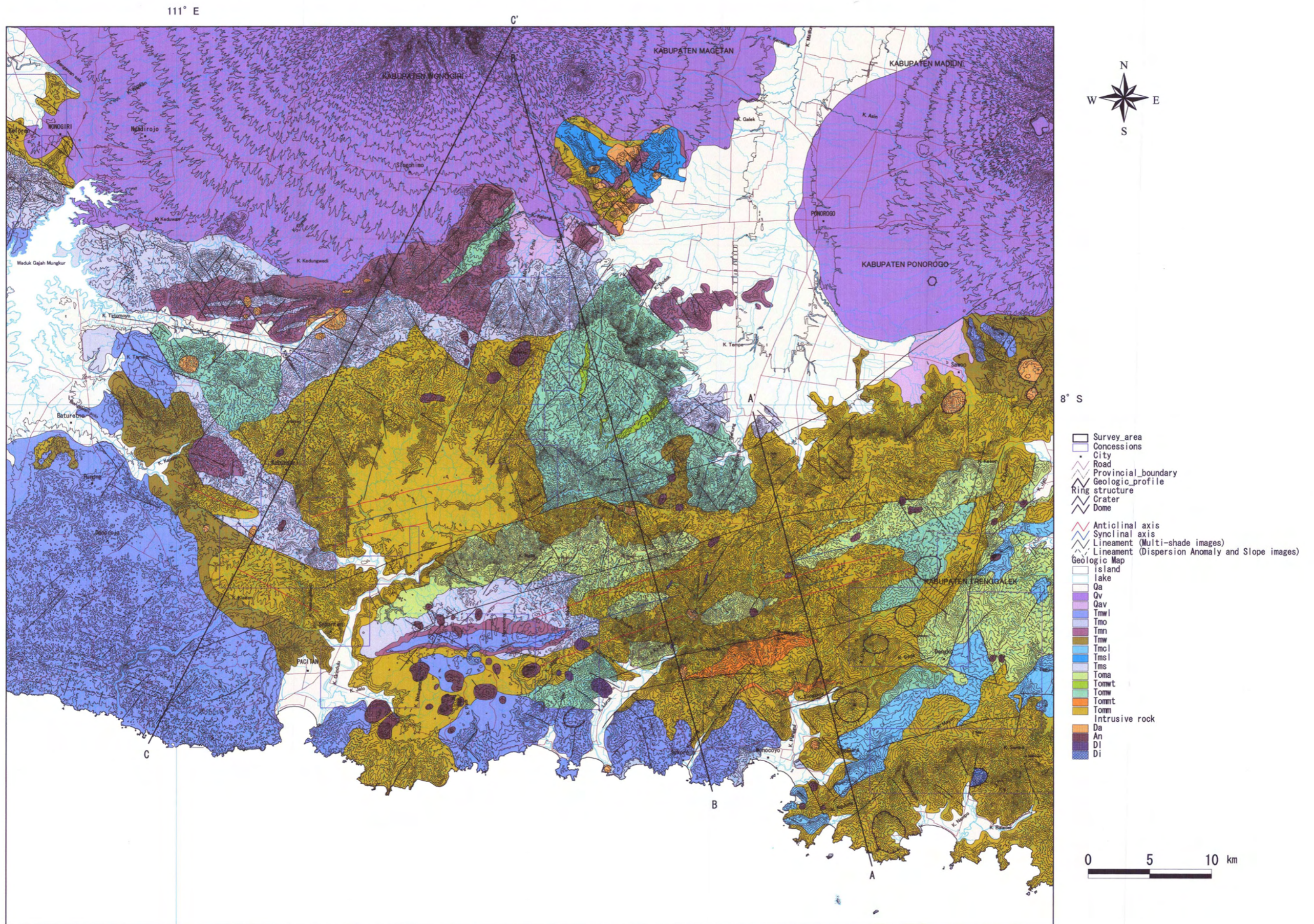
Plate 1 Geologic Map of the Survey Area
