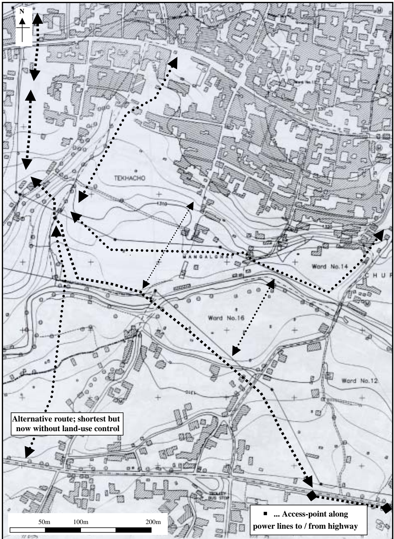
Figure 6.6.1 Disaster Mitigation Bypass Routes for Rescue and Evacuation (in case of designating along electric power lines, in fringe of Bhaktapur built-up area)
