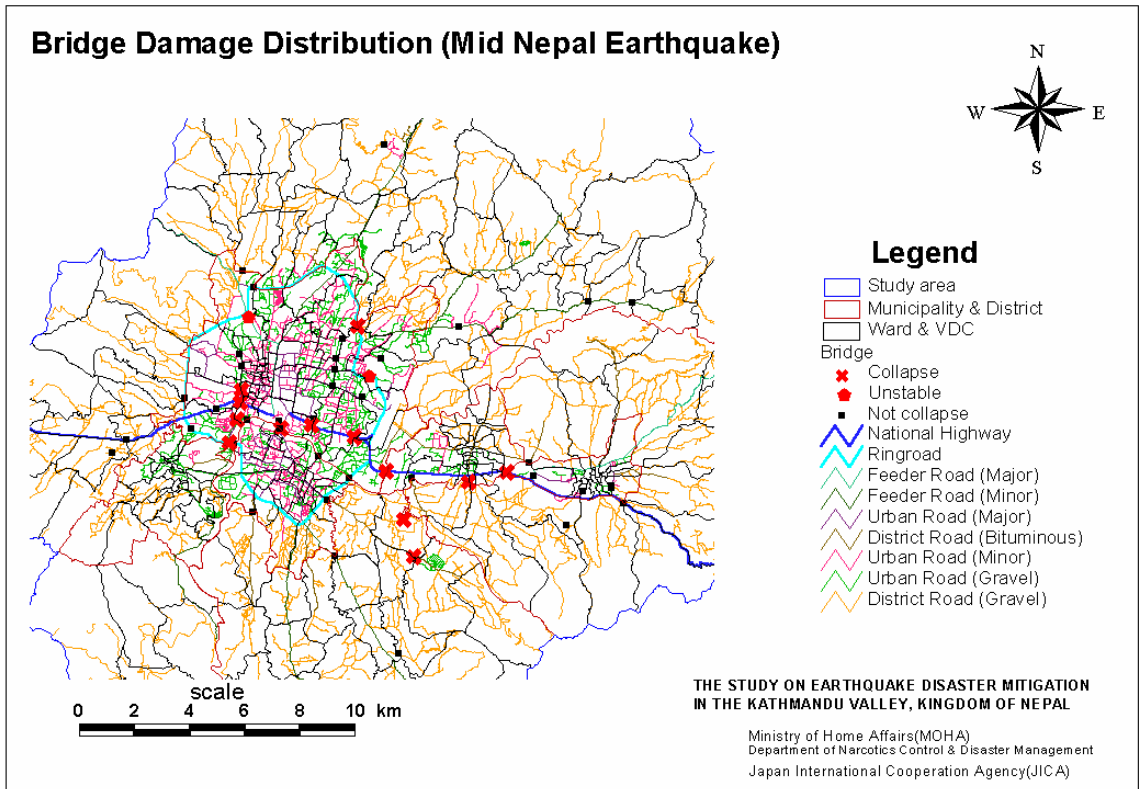
Figure 5.10.3 Damage to Bridge
