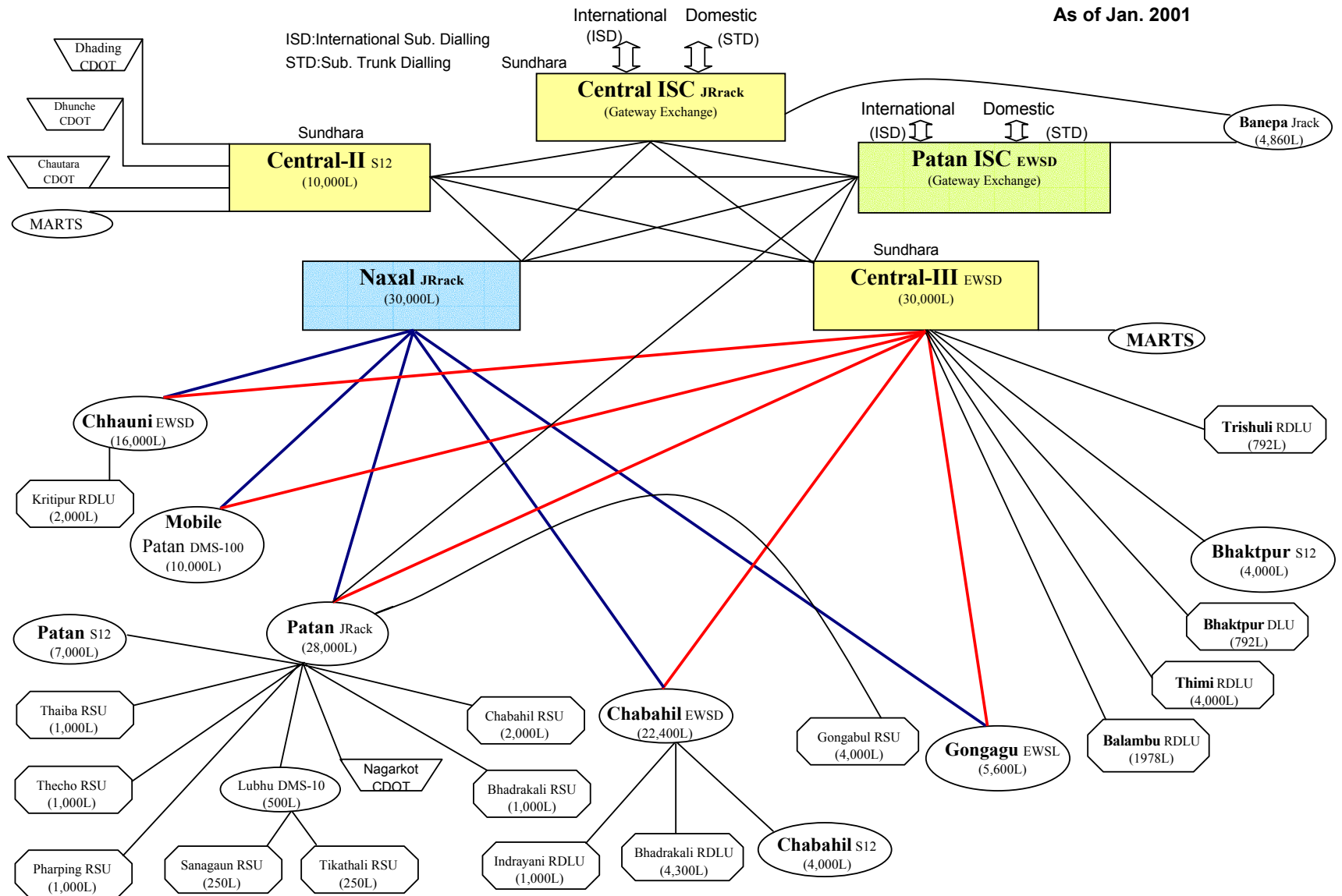
Figure 6.5.1 Trunk Network in Bagmati Zone
