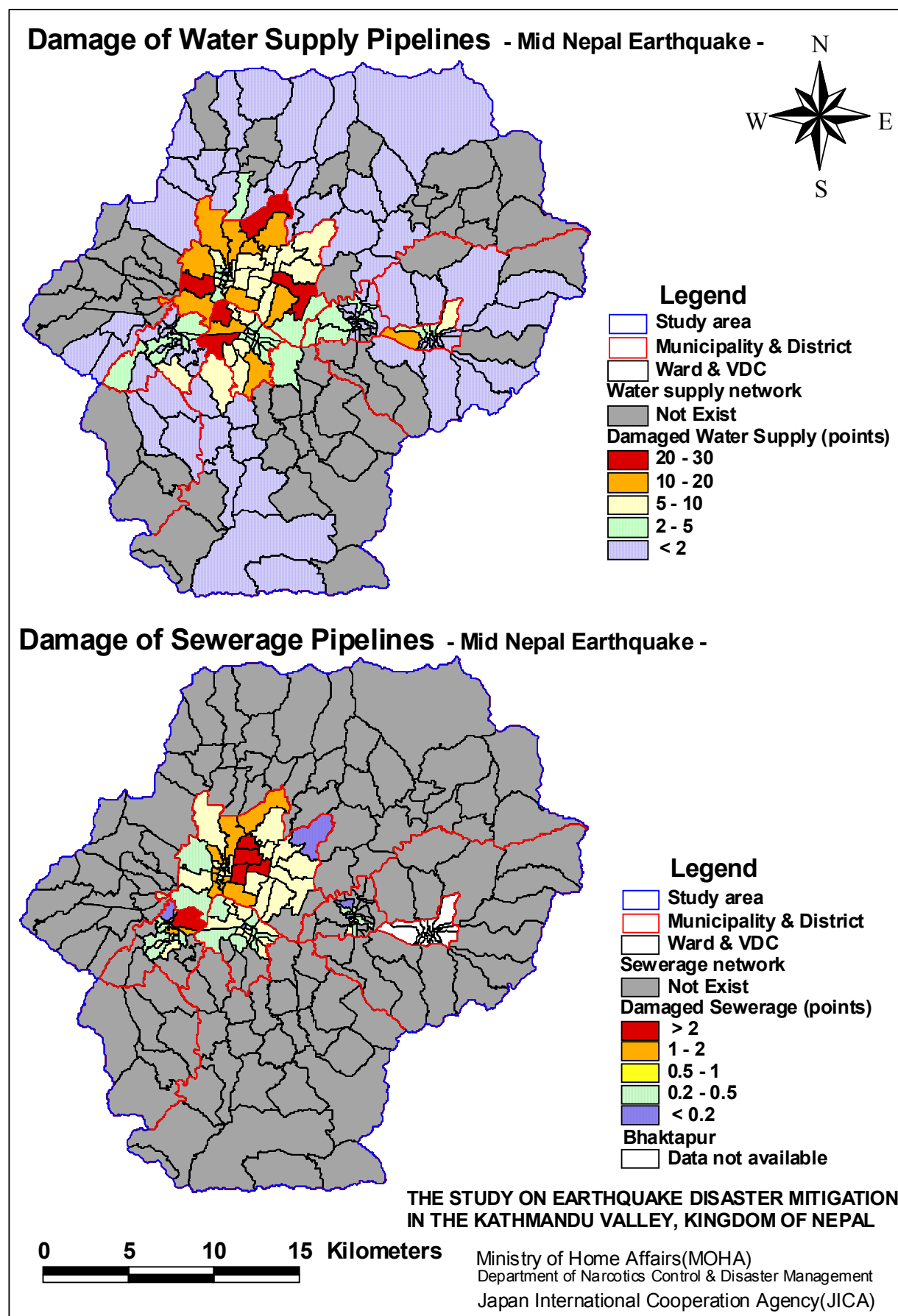
Figure 7.12.1 Damage of Water Supply/ Sewerage Pipelines -Mid Nepal Earthquake-
