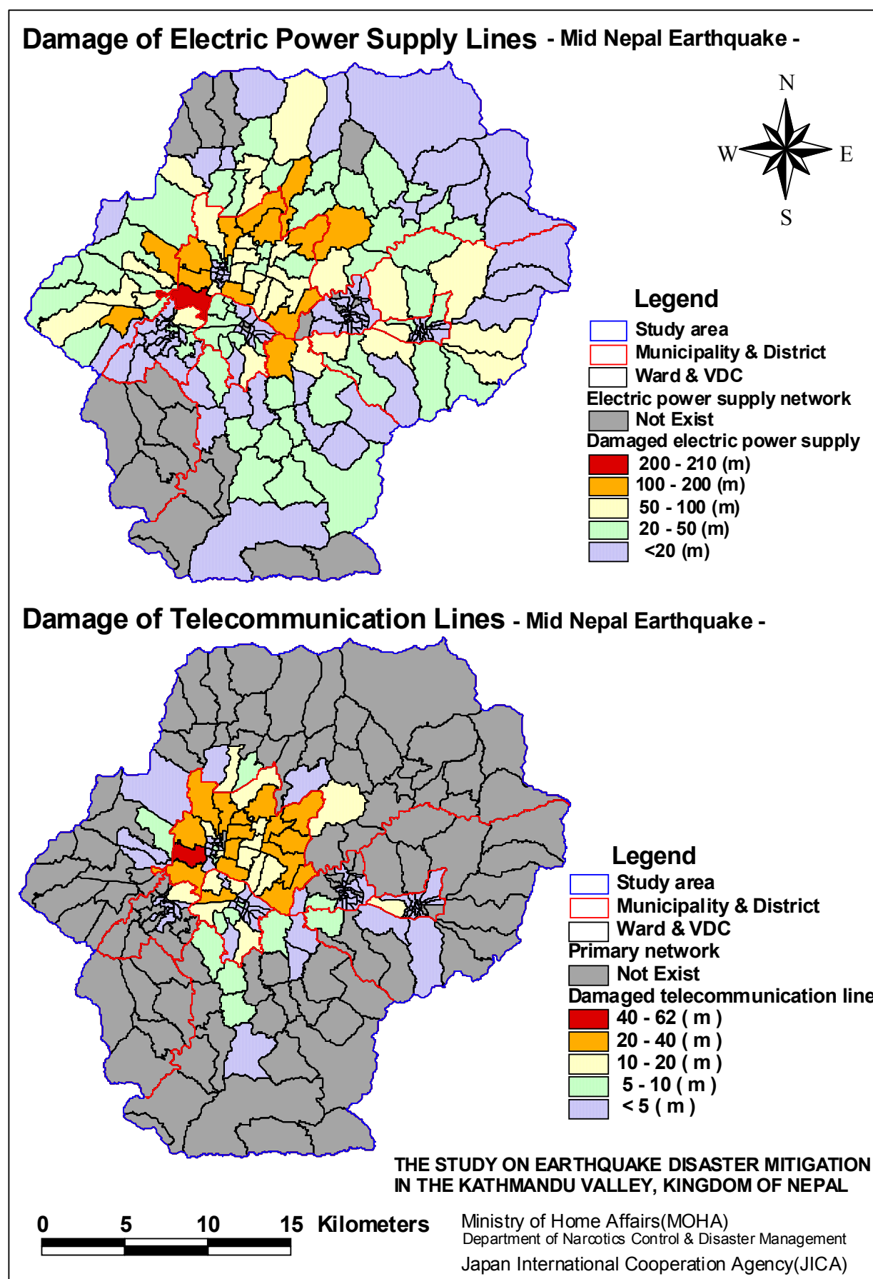
Figure 7.12.2 Damage of Electric Power Supply/ Telecommunication Lines -Mid Nepal Earthquake-
