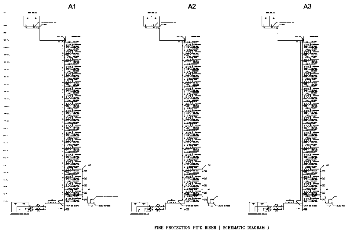
Fire Protection Pipe Riser (Schematic Diagram)
