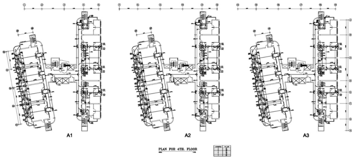
Layout Plan of Plumbing, Sanitary and Fire Protection Work (1/2)
