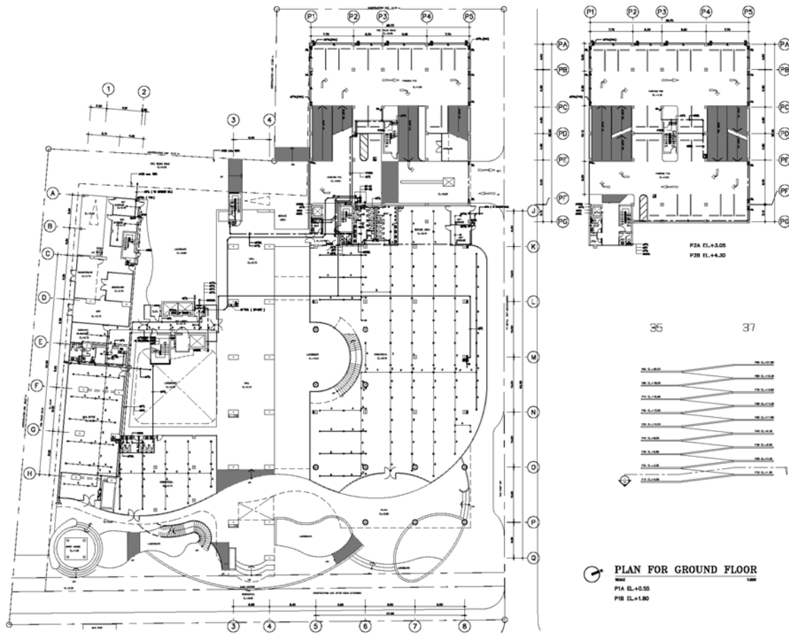
Site Plan for Plumbing, Sanitary and Fire Protection Work
