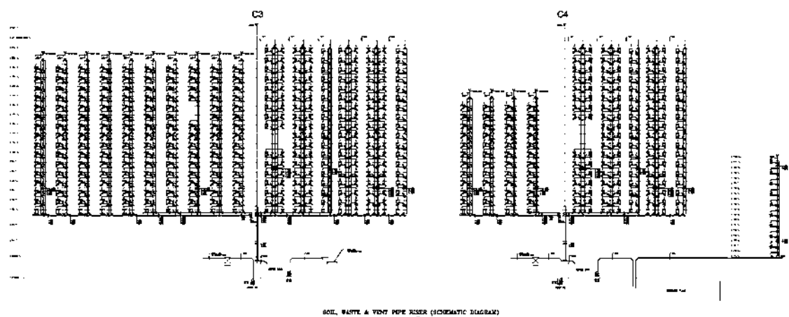
Soil, Waste and Vent Pipe Riser (Schematic Diagram) (2/2)
