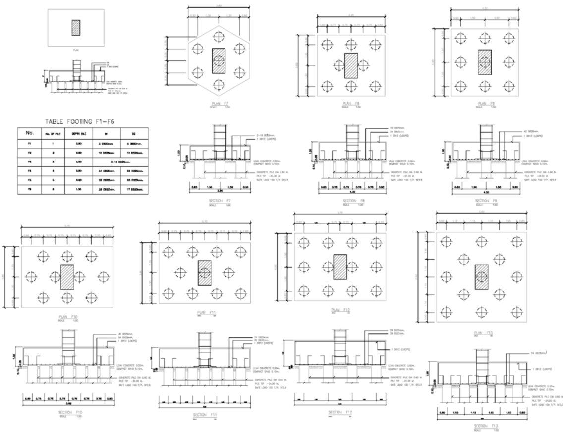
Foundation Plan (1/3)
