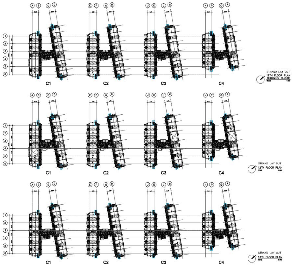
Strand Layout Plan (11th Floor ~ 13th Floor)
