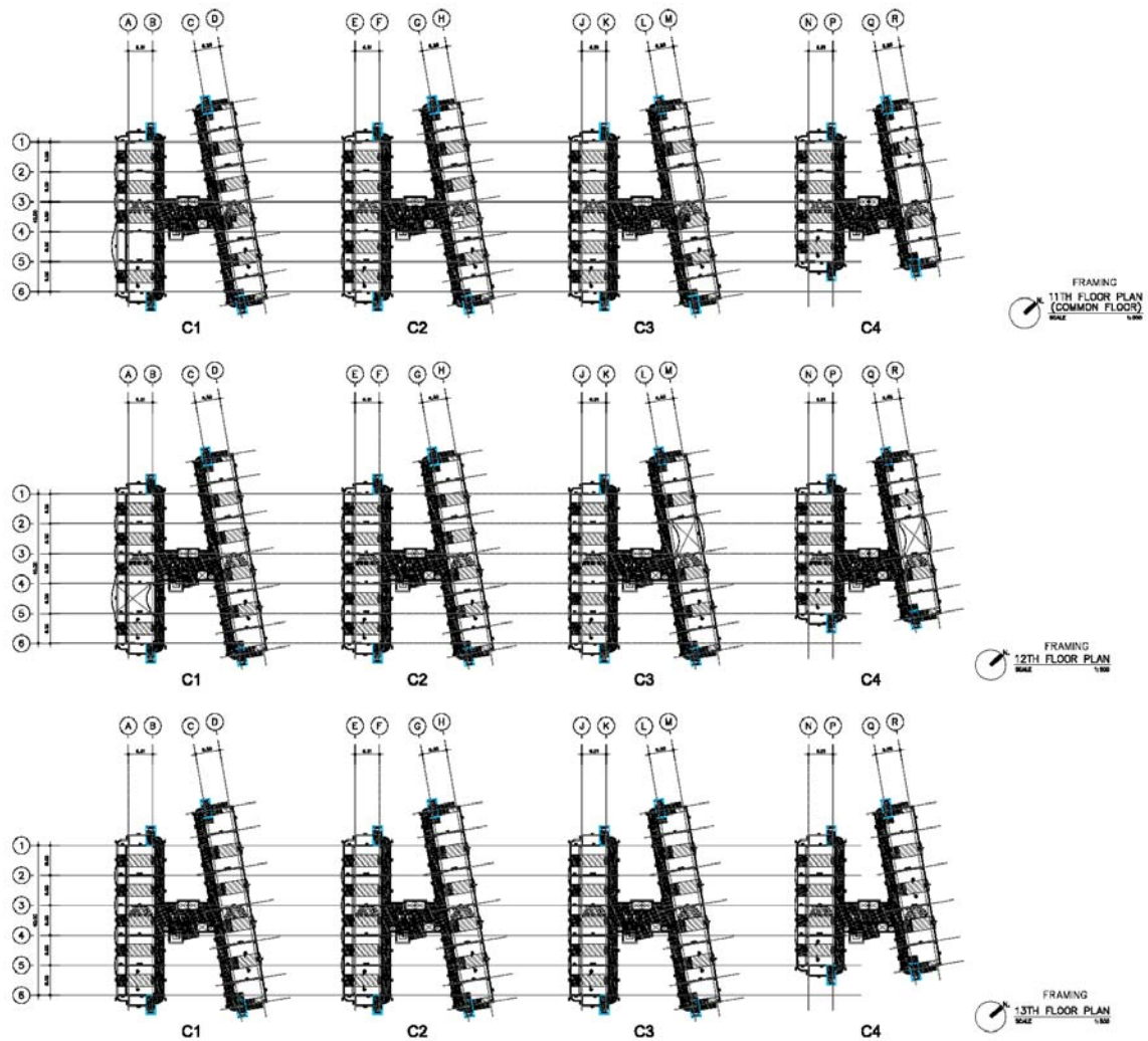
Framing Plan (11th Floor ~ 13th Floor)
