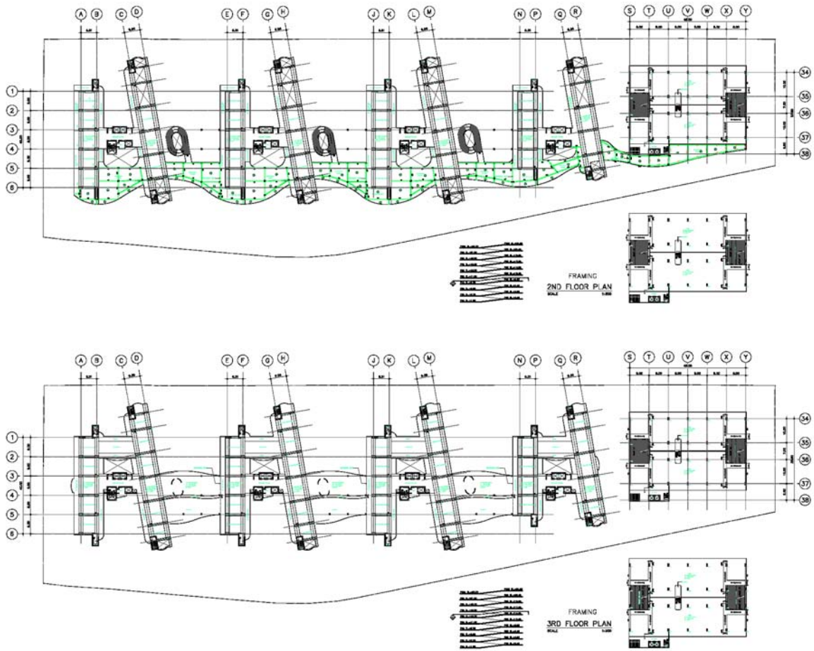
Framing Plan (2nd Floor ~ 3rd Floor)
