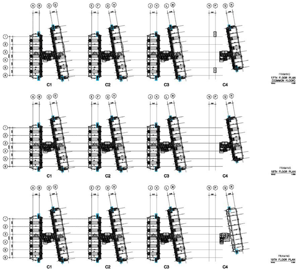
Framing Plan (17th Floor ~ 19th Floor)
