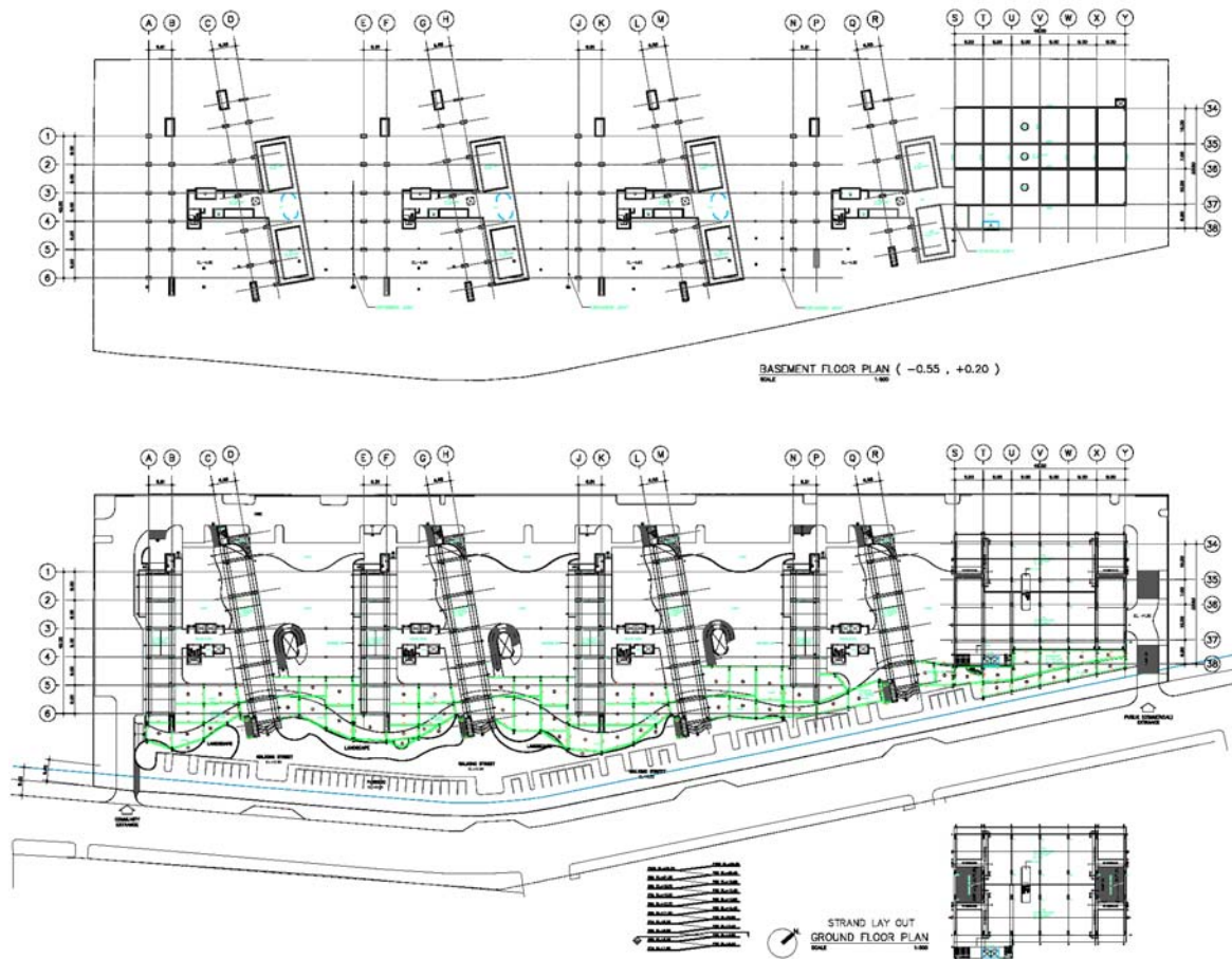
Strand Layout Plan (Basement ~ Ground Floor)
