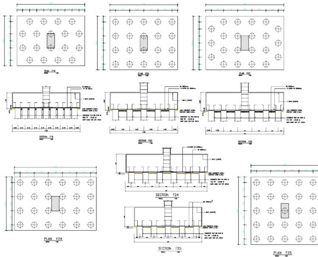
Foundation Plan (3/3)
