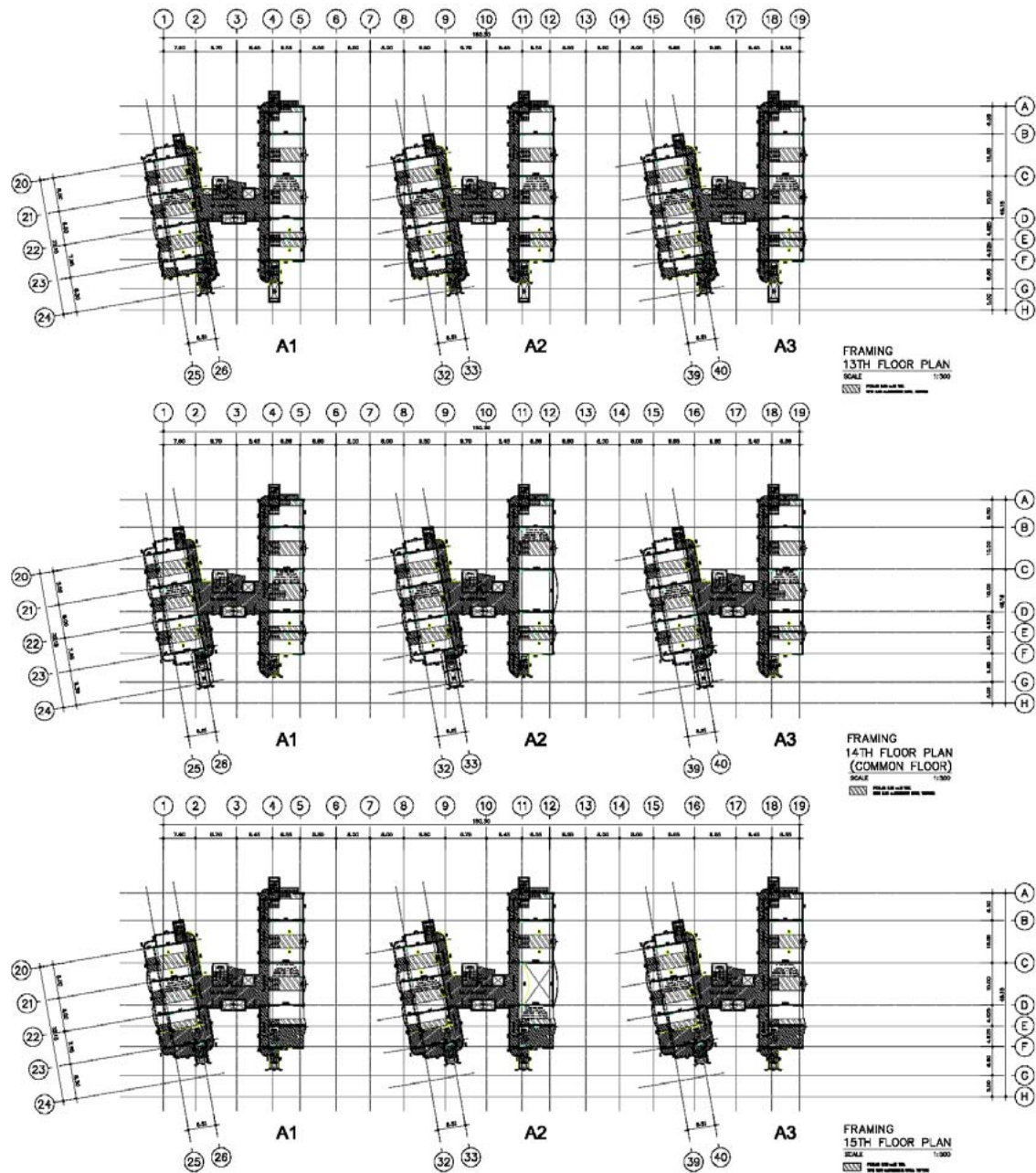
Framing Plan (13th Floor ~ 15th Floor)
