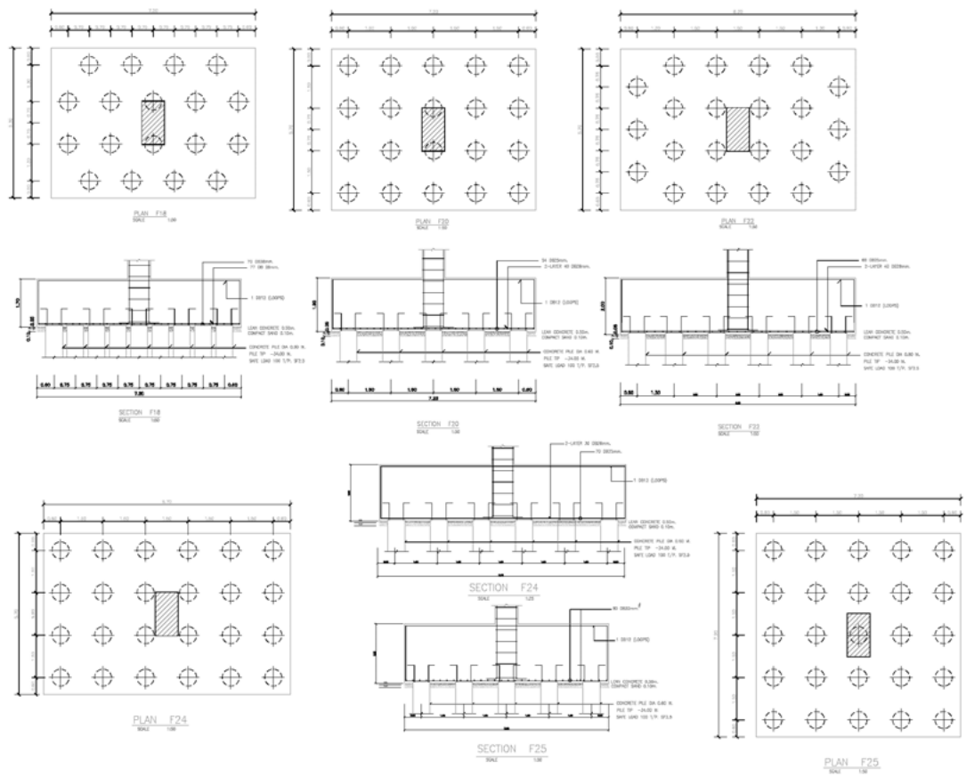
Foundation Plan (3/3)
