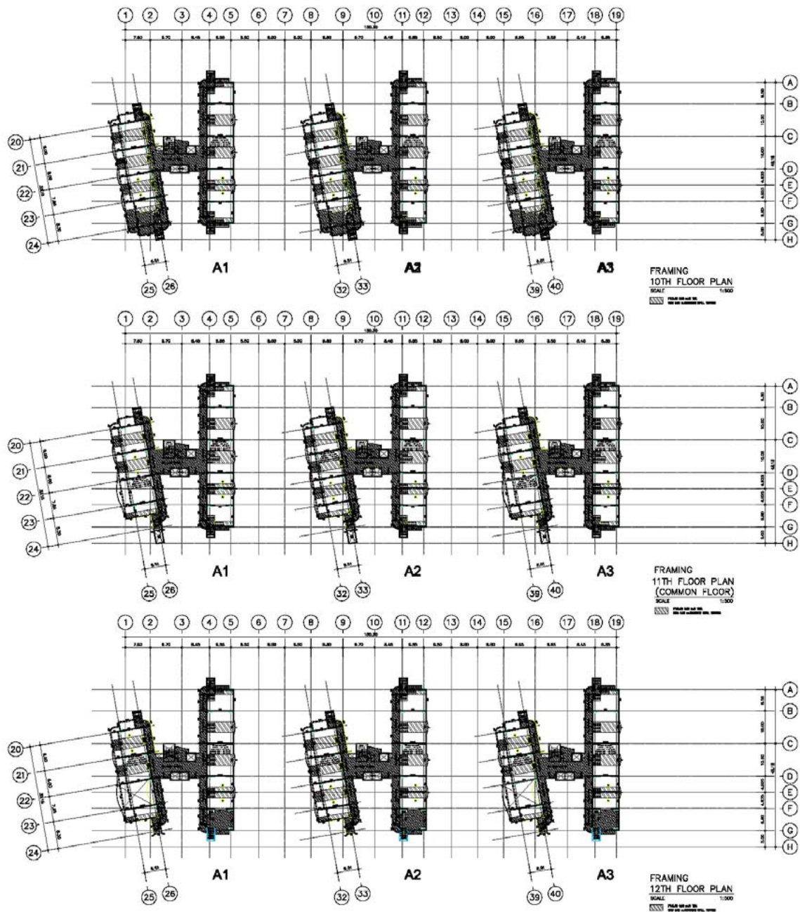
Framing Plan (11th Floor ~ 12th Floor)
