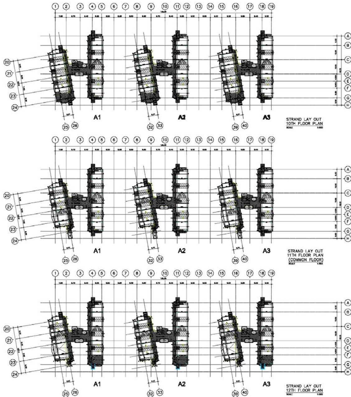
Strand Layout Plan (10th Floor ~ 12th Floor)
