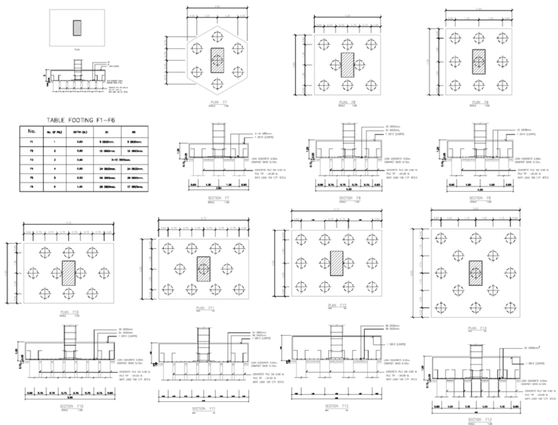
Foundation Plan (1/3)
