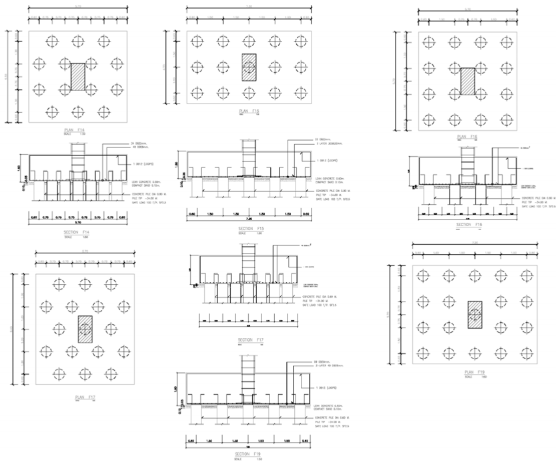
Foundation Plan (2/3)
