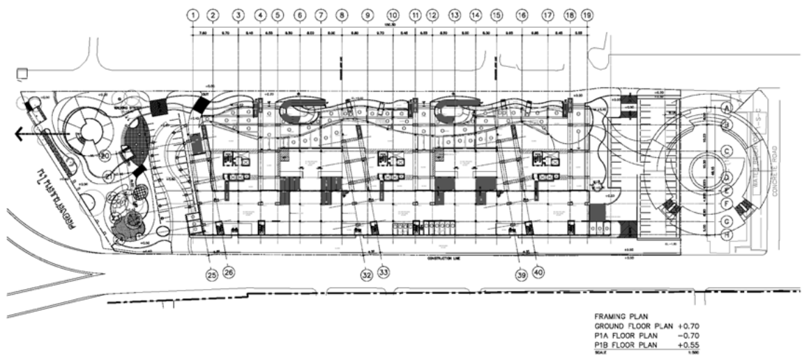
Framing Plan (Ground Floor ~ P1B)
