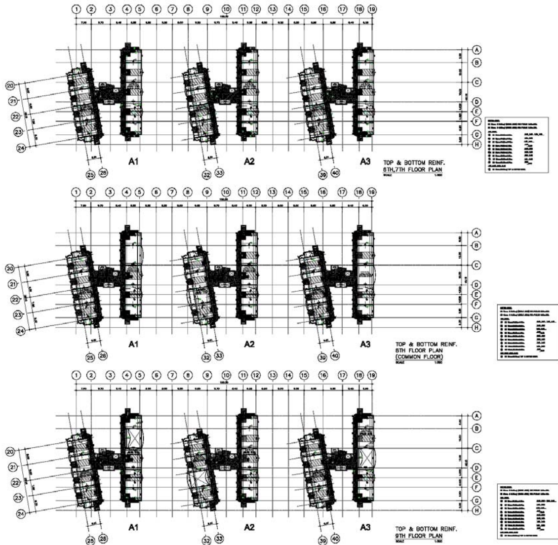
Top and Bottom Reinforcement Plan (6th Floor ~ 9th Floor)
