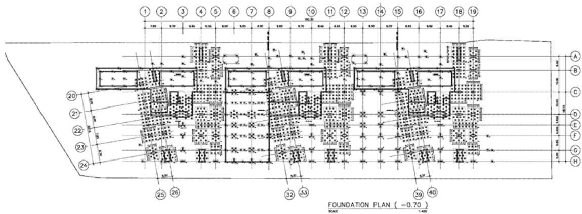
Foundation Plan
