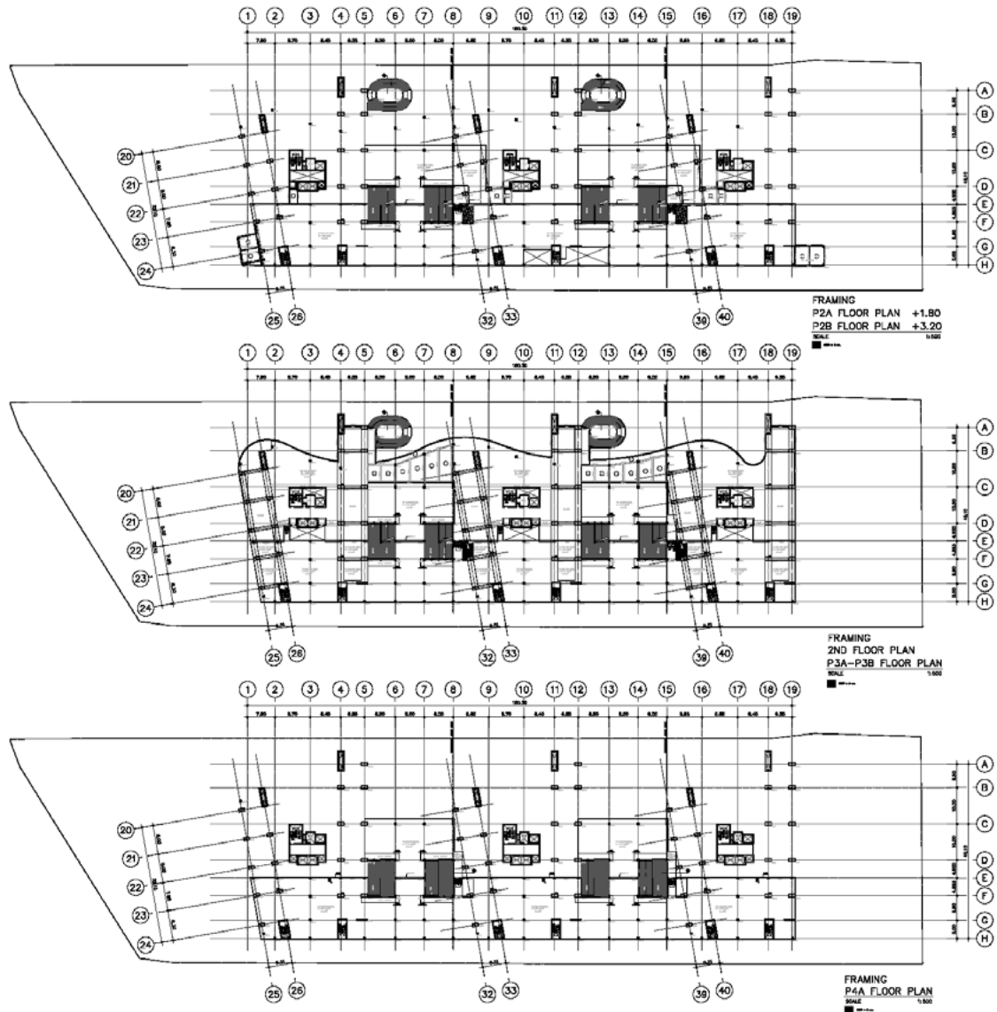
Framing Plan (P2A ~ P4A)
