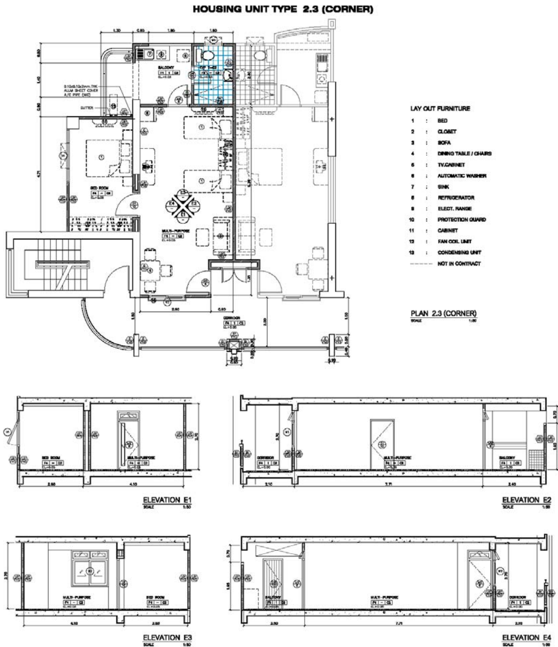
Housing Unit Plan (Type 2.3)
