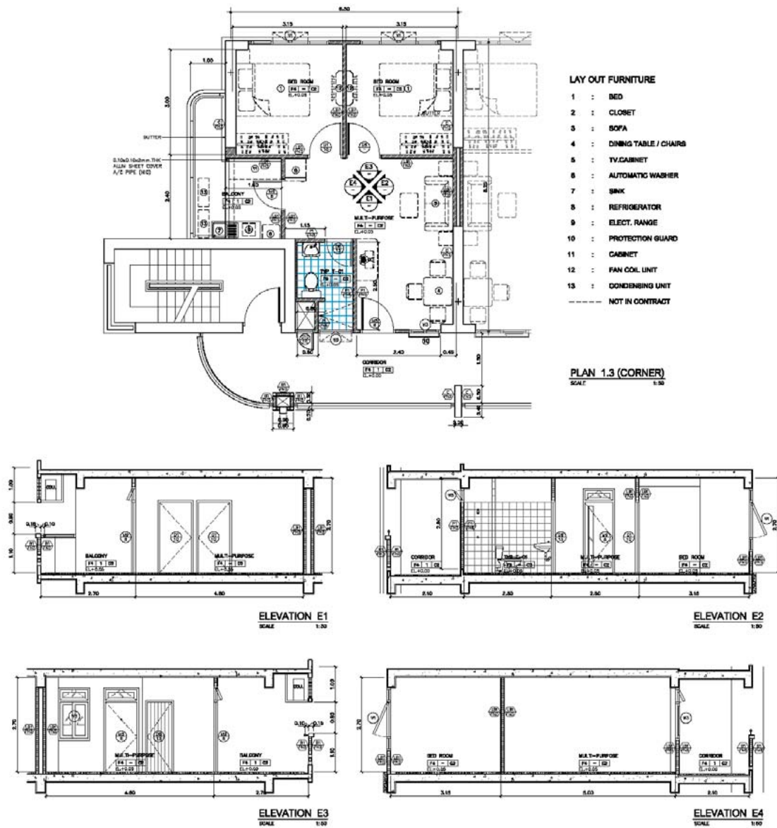
Housing Unit Plan (Type 1.3)
