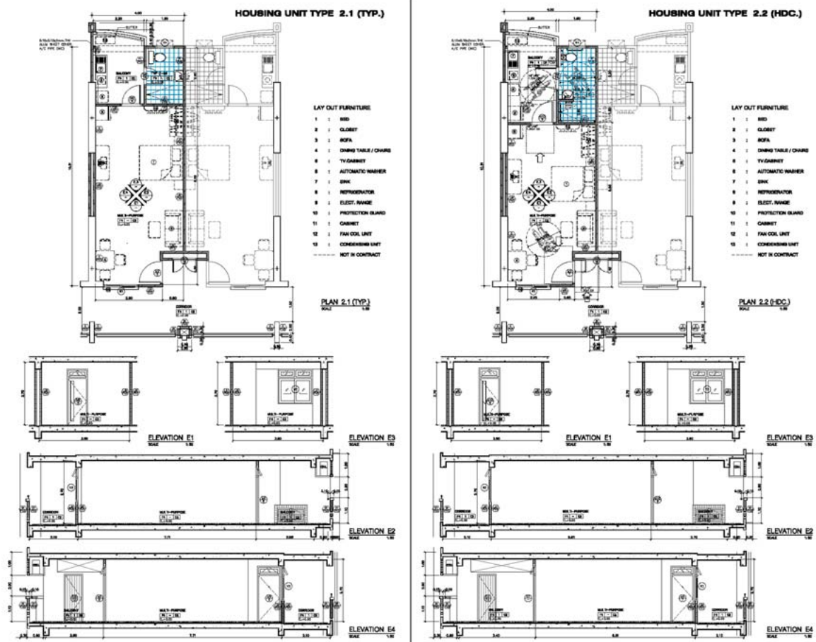
Housing Unit Plan (Type 2.1 and 2.2)
