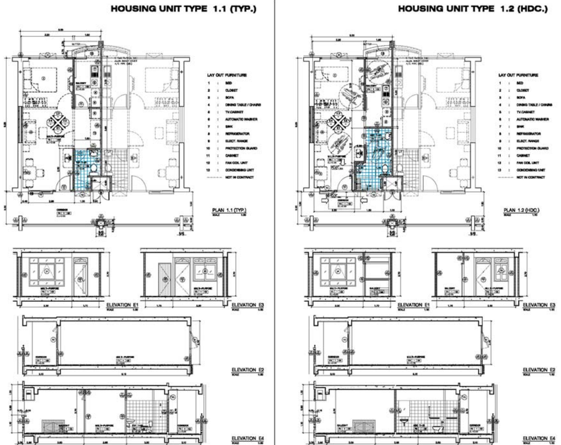
Housing Unit Plan (Type 1.1 and 1.2)
