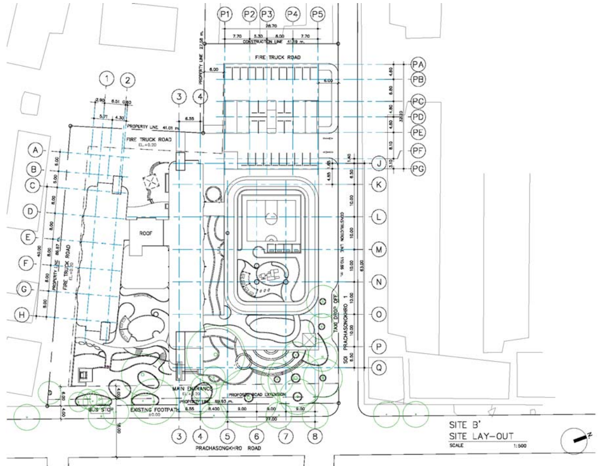
Site Layout
