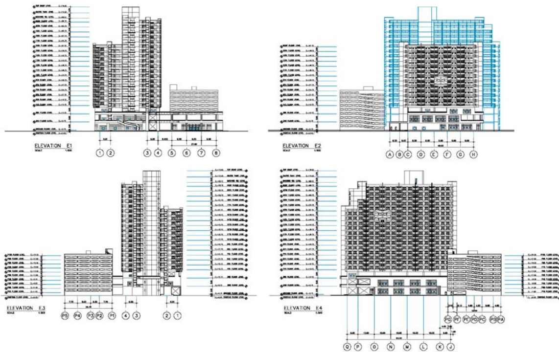
Elevation Viewed from Four Directions
