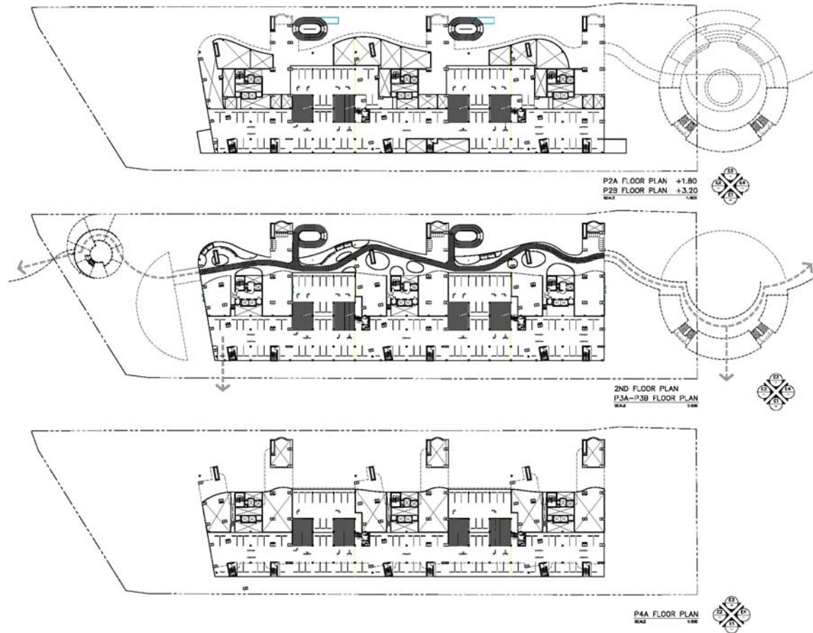
Floor Plan (P2A ~ P4A)
