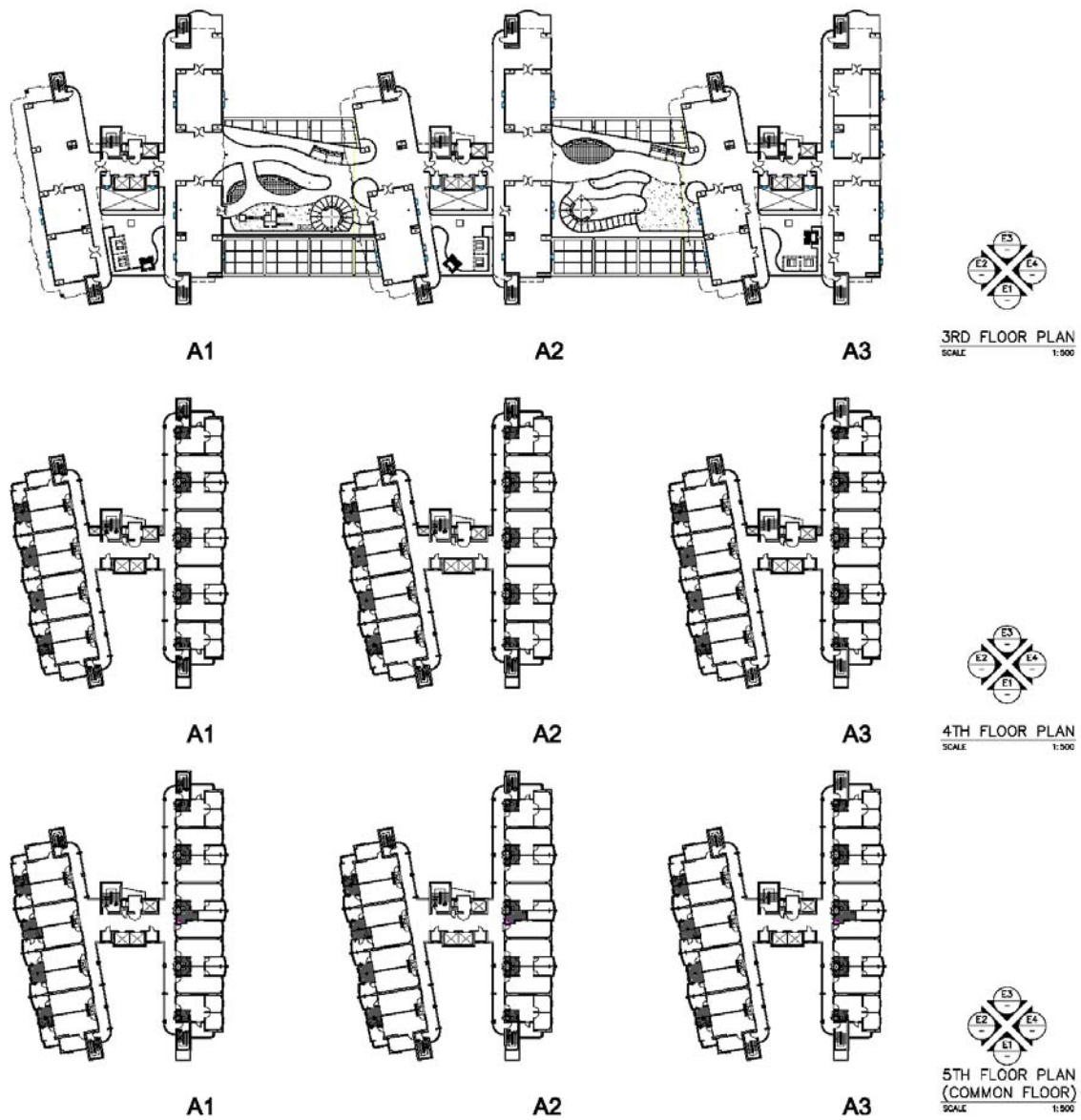
Floor Plan (3rd Floor ~ 5th Floor)
