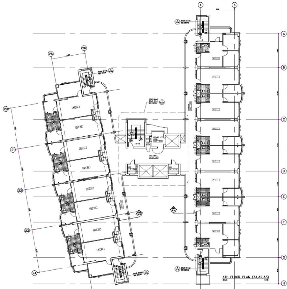
Floor Plan (4th Floor)
