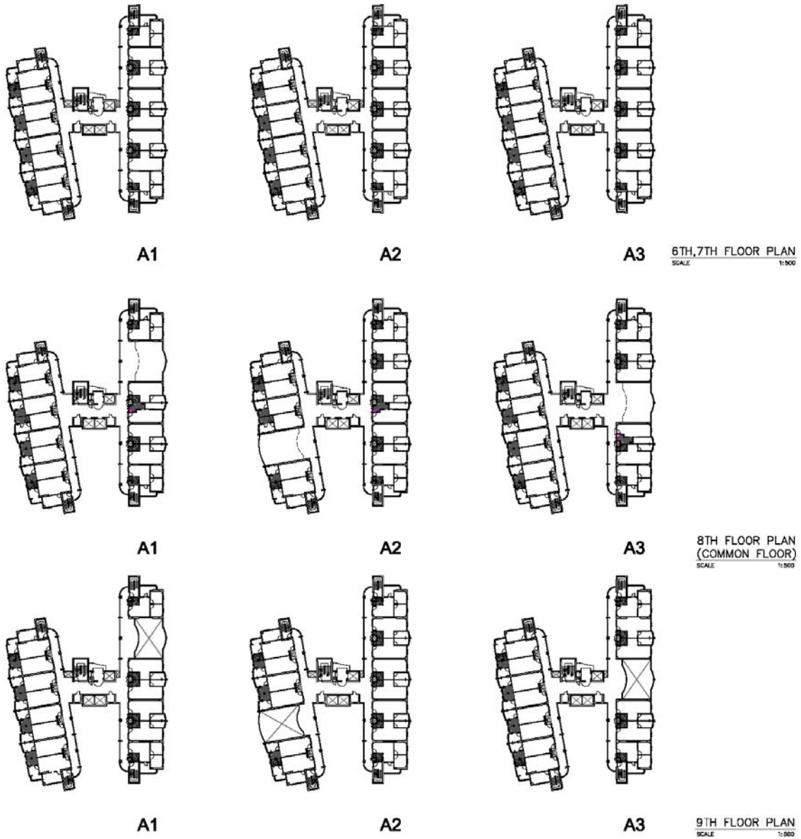
Floor Plan (6th Floor ~ 9th Floor)
