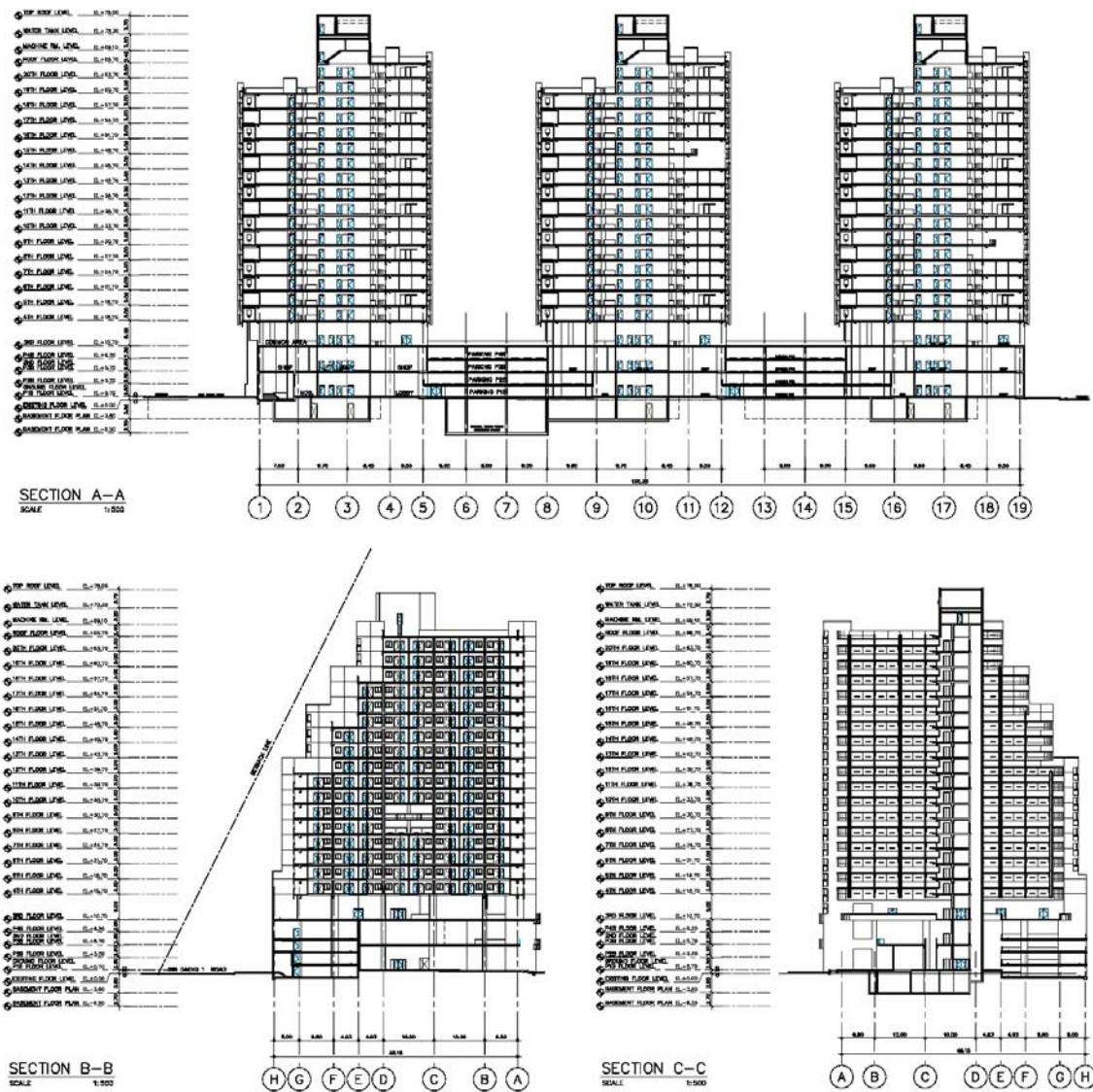
Elevation (Section A-A, B-B, C-C)
