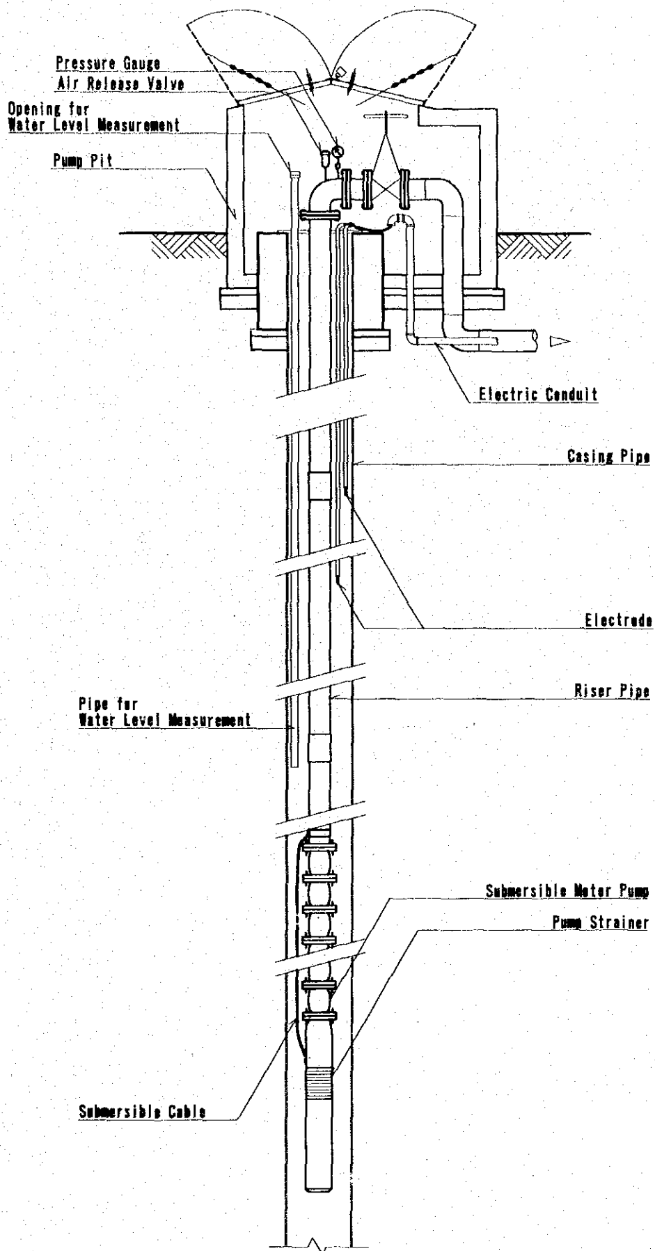
SUBMERSIBLE MOTOR PUMP AND PUMP PIT
