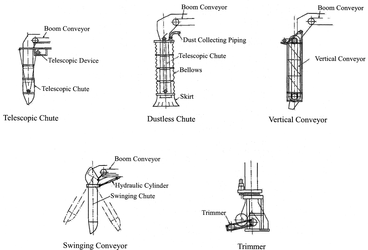
Chutes for Ship Loaders
