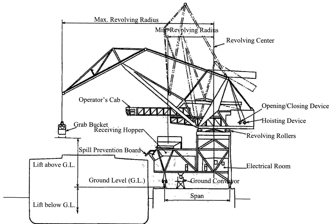
Grab Bucket Ship Unloader, Level Luffing Crane Type
