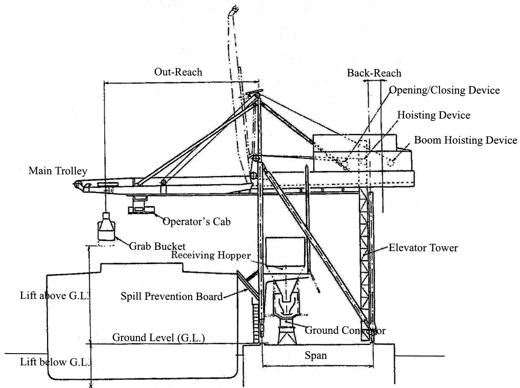
Grab Bucket Ship Unloader, Gantry Crane Type
