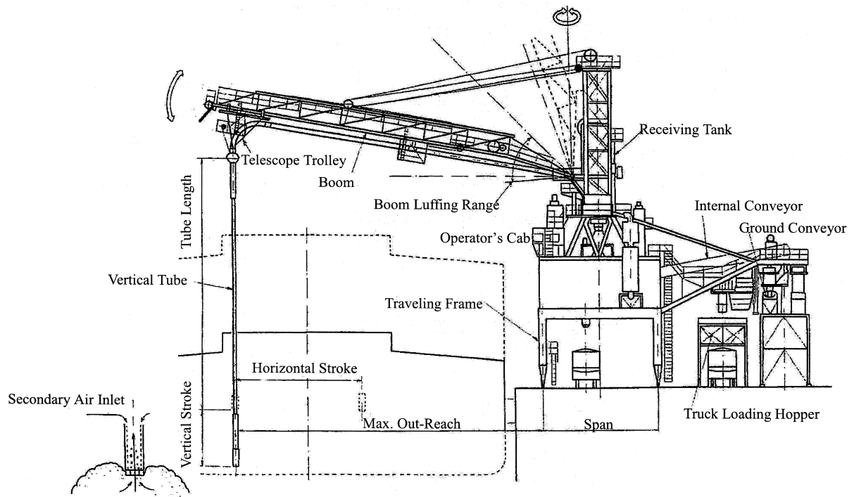
Pneumatic Ship Unloader
