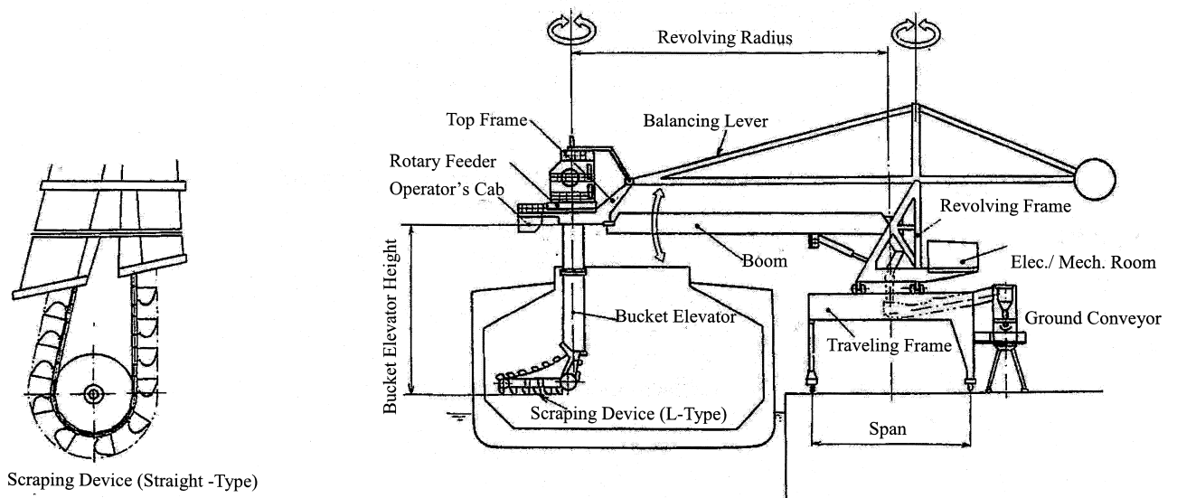
Mechanical Continuous Unloader, Bucket Elevator Type
