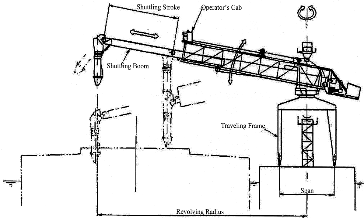
Ship Loader, Traveling/Luffing/Shuttling/Revolving Type
