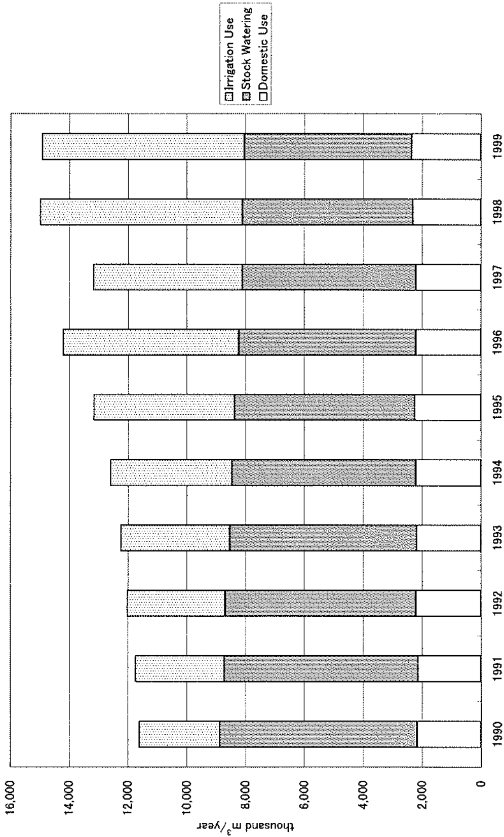
Fig. 12-44 Variation of Groundwater Use in 1990-1999 by Usage
