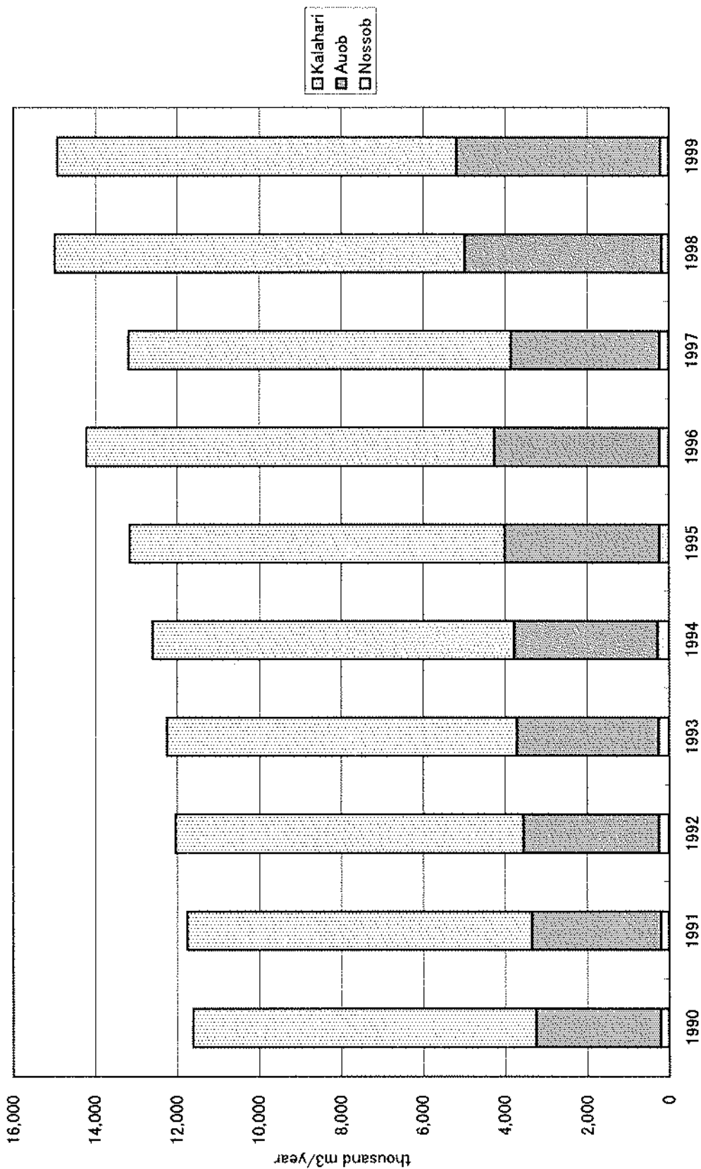
Fig. 12-45 Variation of Groundwater Use in 1990-1999 by Aquifer
