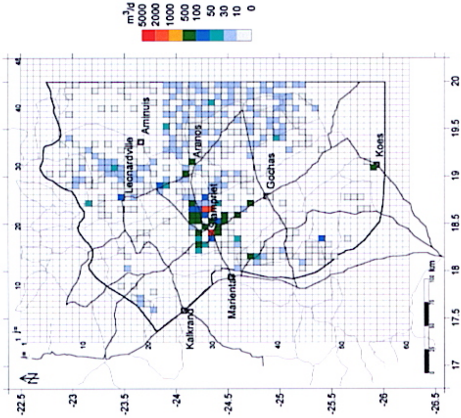
Fig. 12-33 Distribution of Groundwater Use in Auob Aquifer in 1999
