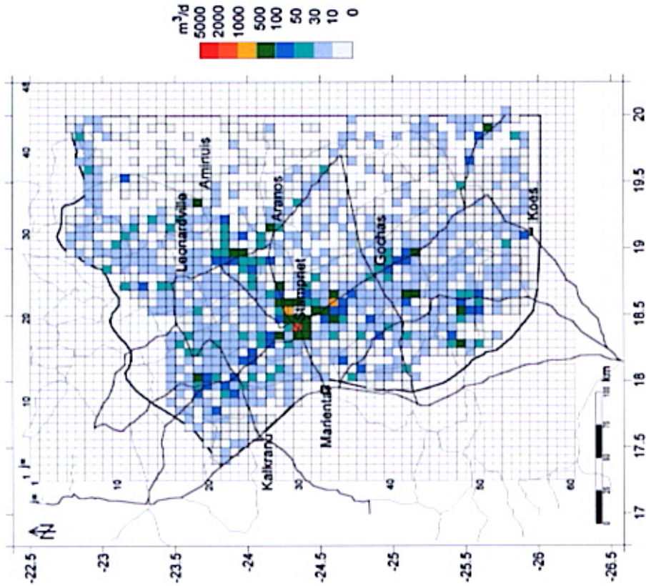
Fig. 12-32 Distribution of Groundwater Use in Kalahari Aquifer in 1999
