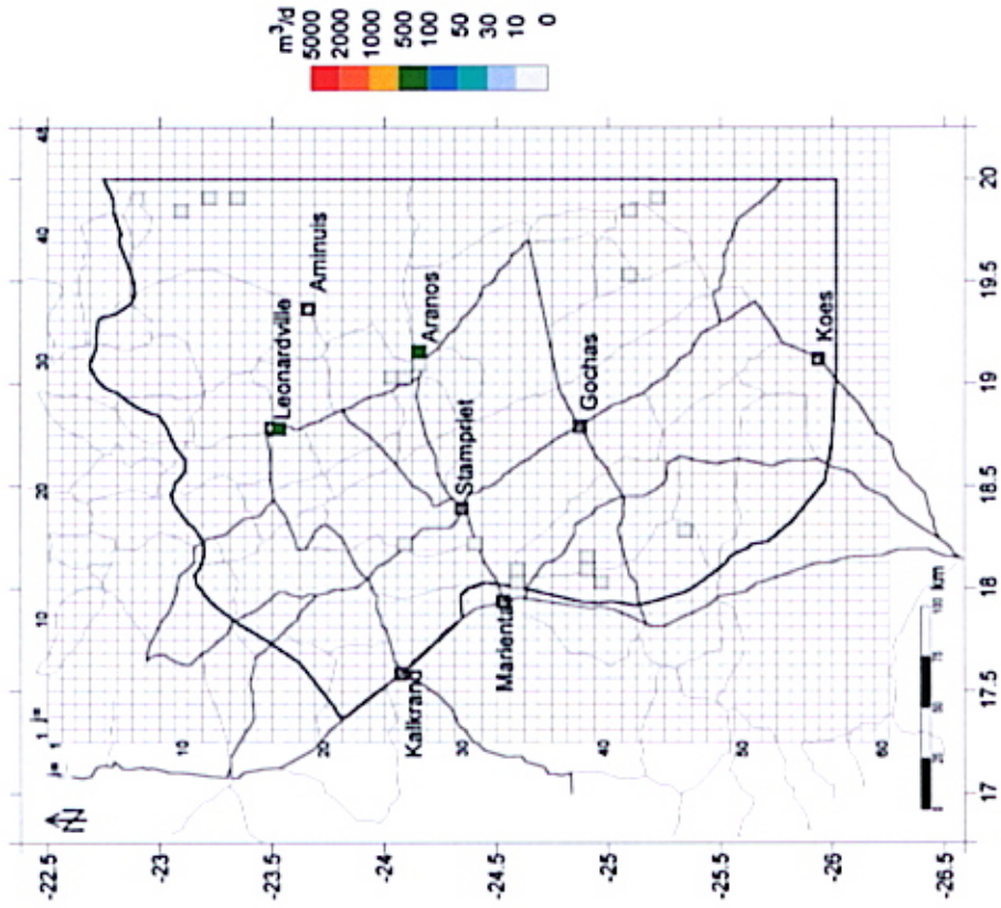
Fig. 12-37 Distribution of Domestic Use in Nossob Aquifer in 1999
