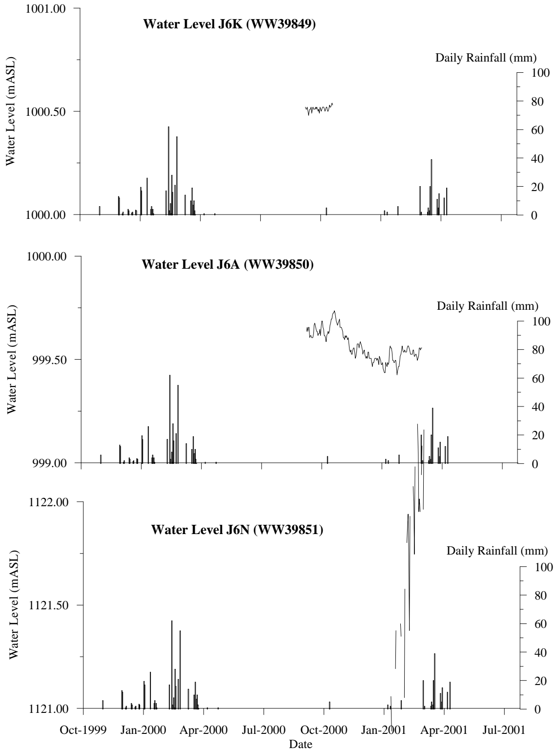
Fig. 8.4-11(6) ) Fluctuation of Piezometric Head at JICA Test Borehole J-6
