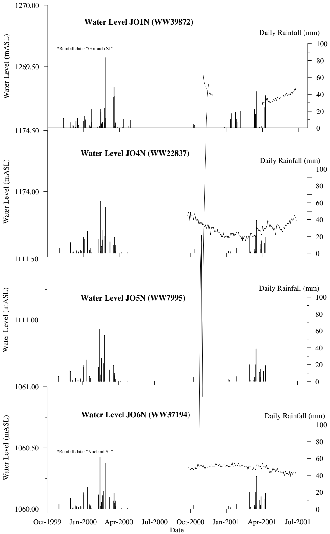
Fig. 8.4-12 (2) Fluctuation of Piezometric Head in Nossob Aquifer at Existing Borehole
