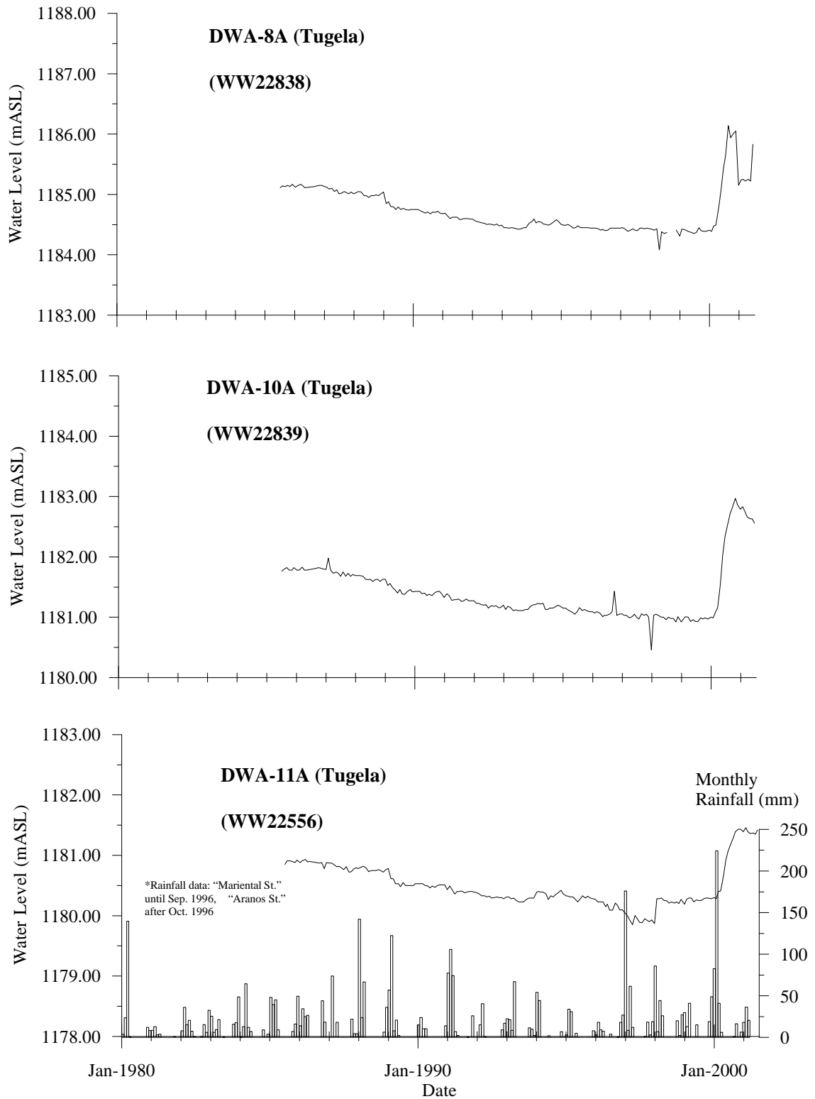
Fig. 8.4-9 (3) Fluctuation of Piezometric Head in Auob Aquifer at DWA's Observation Boreholes
