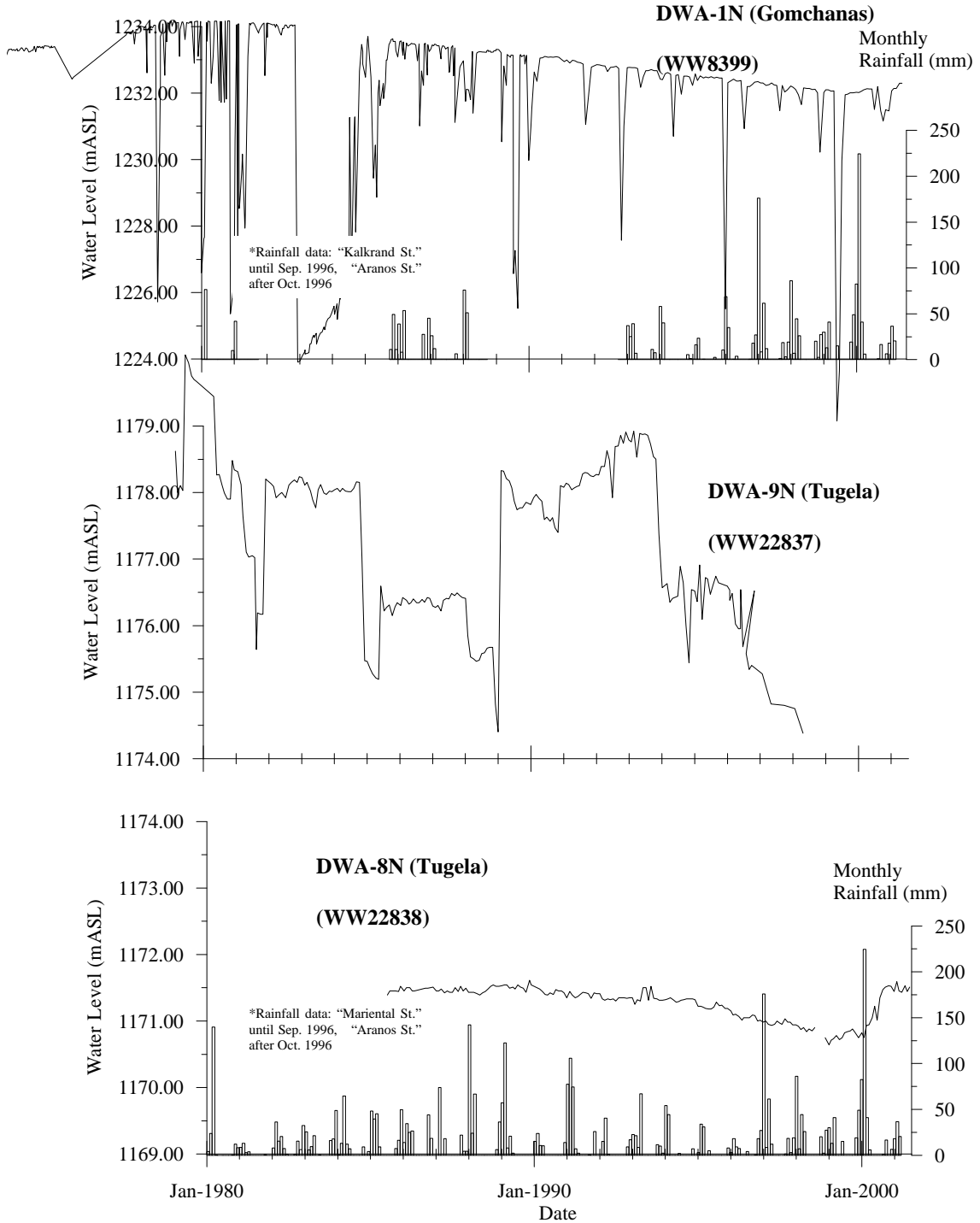
Fig. 8.4-10 (1) Fluctuation of Piezometric Head in Nossob Aquifer at DWA's Observation Boreholes
