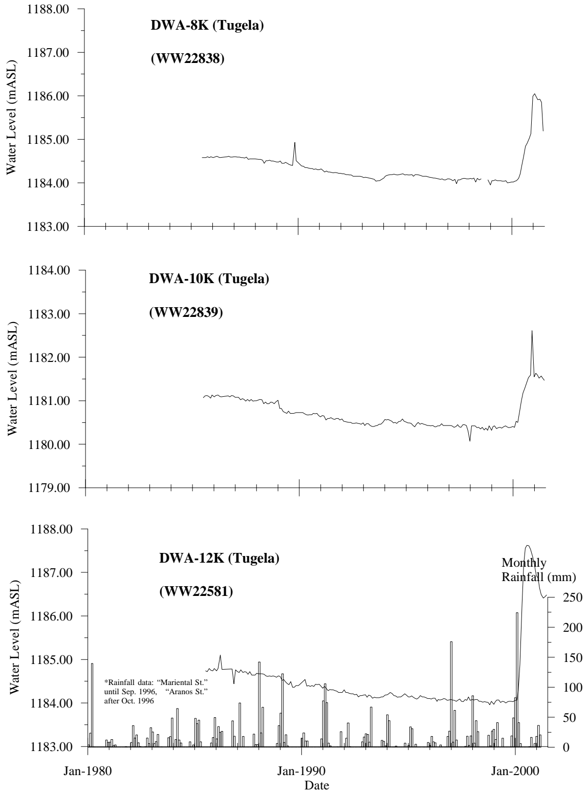
Fig.8.4-8 (3) Fluctuation of Water Level in Kalahari Aquifer at DWA's Observation Boreholes
