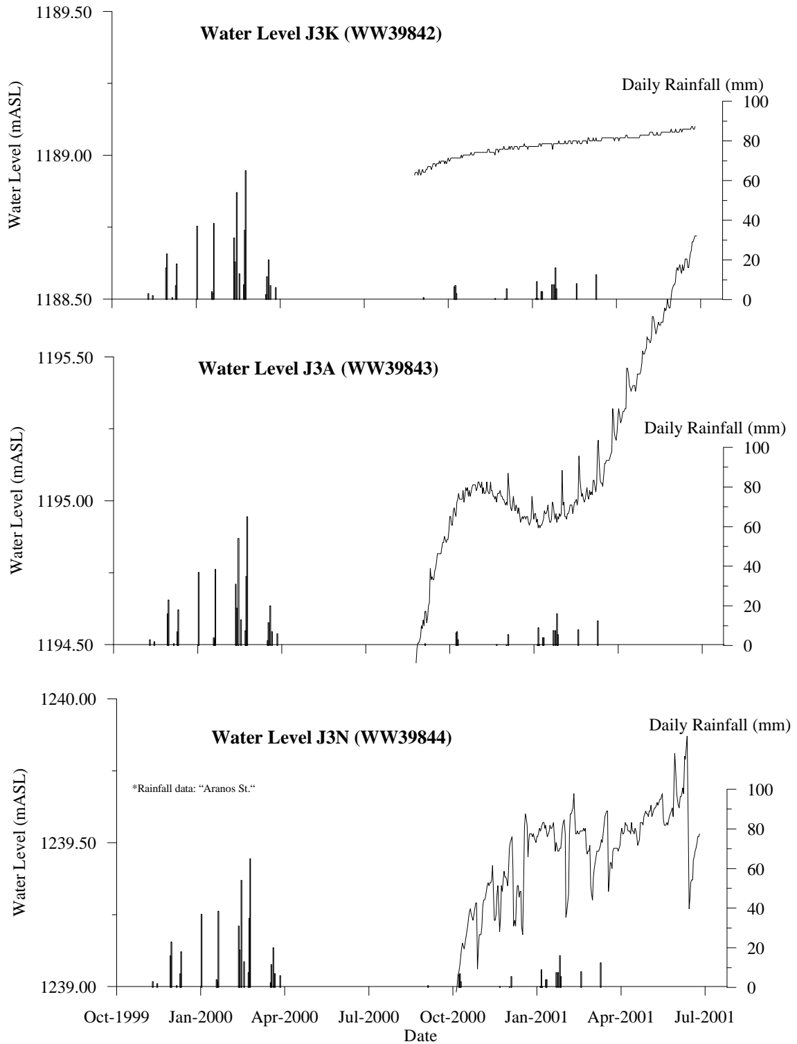
Fig. 8.4-11 (3) Fluctuation of Piezometric Head at JICA Test Borehole J-3
