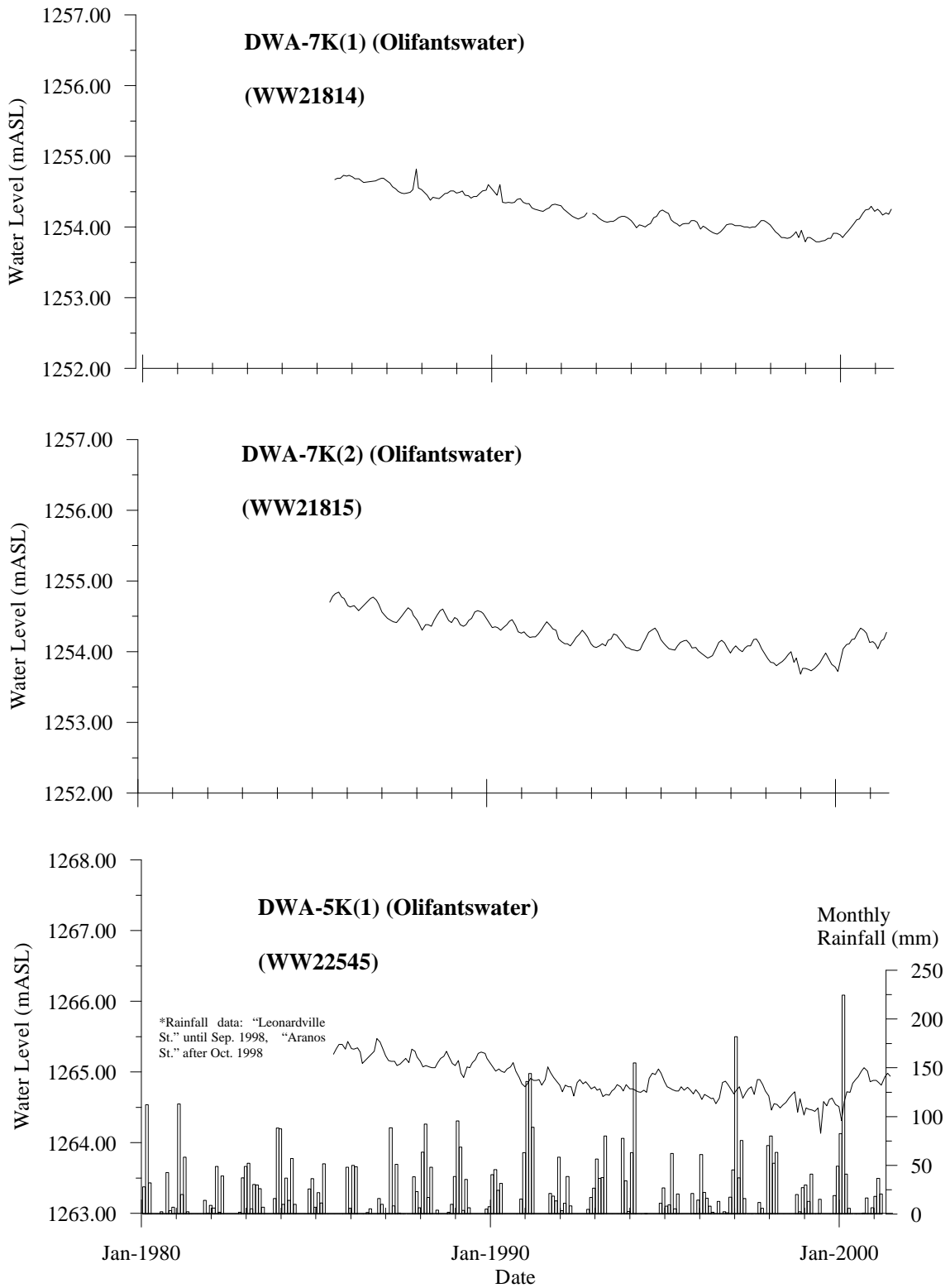
Fig.8.4-8 (1) Fluctuation of Water Level in Kalahari Aquifer at DWA's Observation Boreholes
