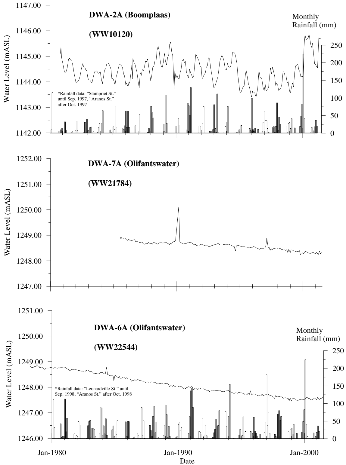
Fig. 8.4-9 (1) Fluctuation of Piezometric Head in Auob Aquifer at DWA's Observation Boreholes
