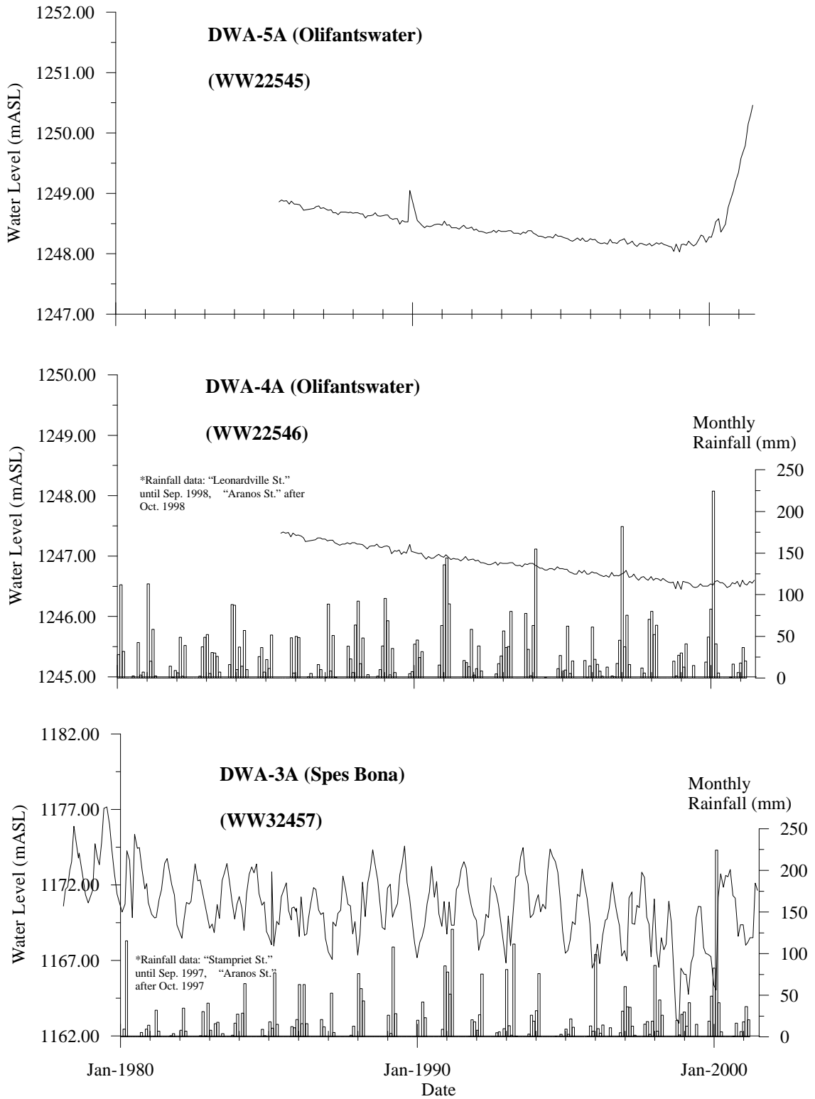
Fig. 8.4-9 (2) Fluctuation of Piezometric Head in Auob Aquifer at DWA's Observation Boreholes
