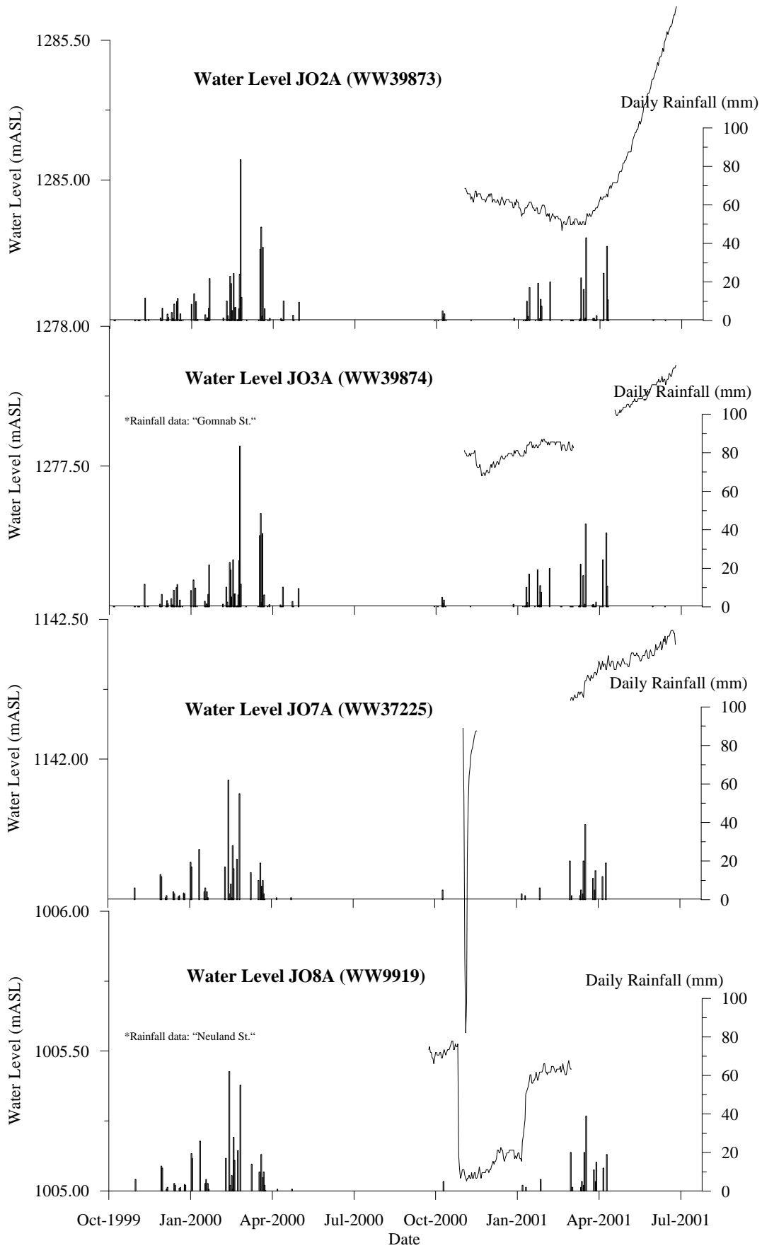
Fig. 8.4-12(1) Fluctuation of Piezometric Head in Auob Aquifer at Existing Borehole
