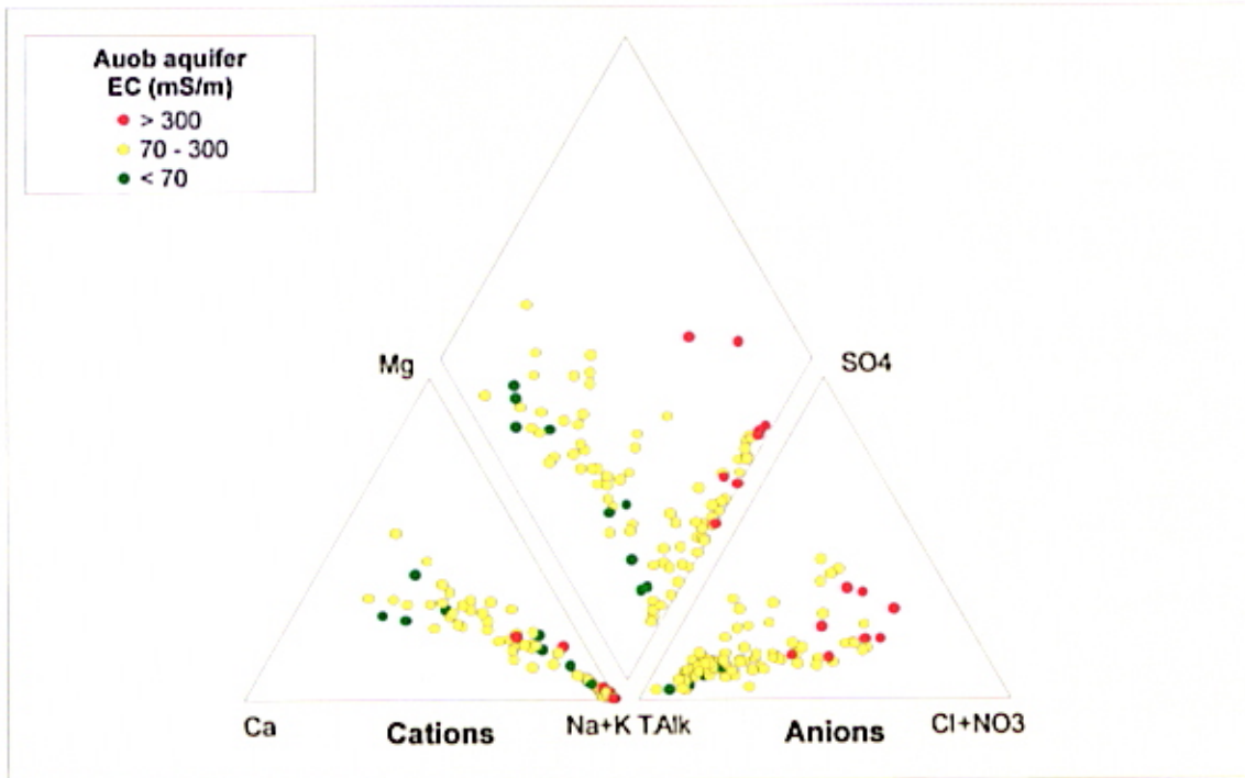
Figure 7.18e Trilinear Diagram Showing the Relative Chemical Composition and the Overall Salinity of Groundwater in the Auob Aquifer
