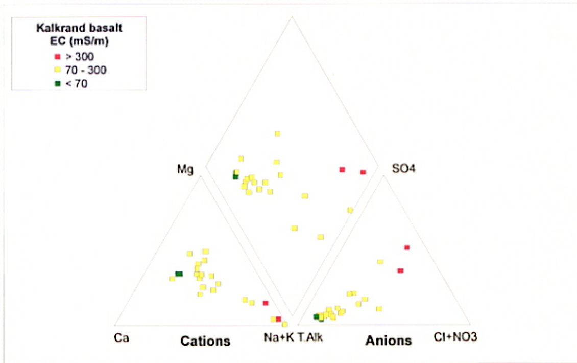
Figure 7.18c Trilinear Diagram Showing the Relative Chemical Composition and the Overall Salinity of Groundwater in the Kalkrand Basalt
