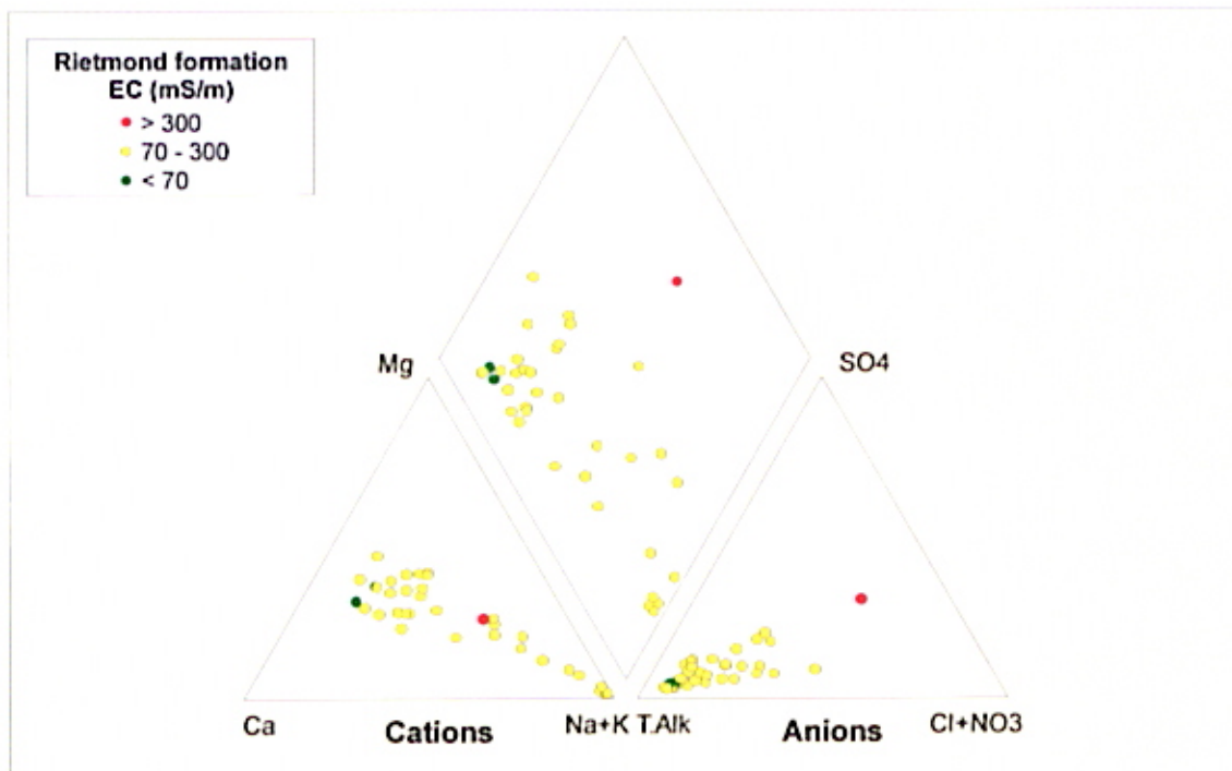
Figure 7.18d Trilinear Diagram Showing the Relative Chemical Composition and the Overall Salinity of Groundwater in the Rietmond Formation
