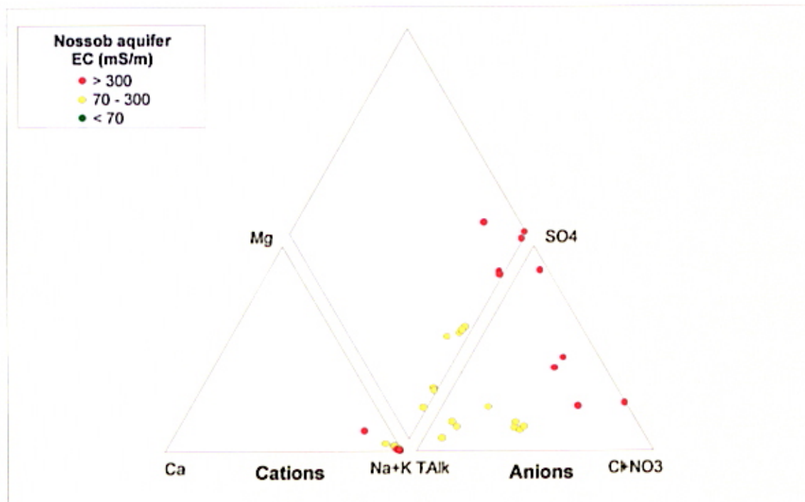
Figure 7.18f Trilinear Diagram Showing the Relative Chemical Composition and the Overall Salinity of Groundwater in the Nossob Aquifer
