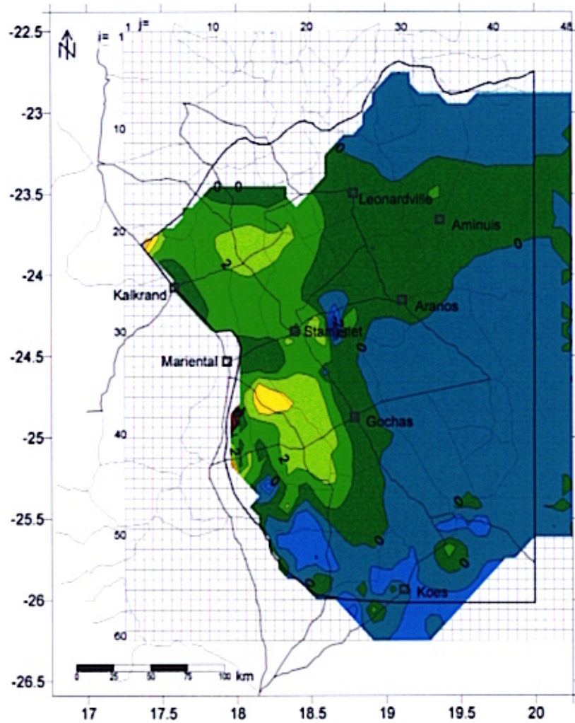
Fig.5.3-16 Calculated Drawdown of the Kalahari Aquifer, Case 5 (100 years after)
