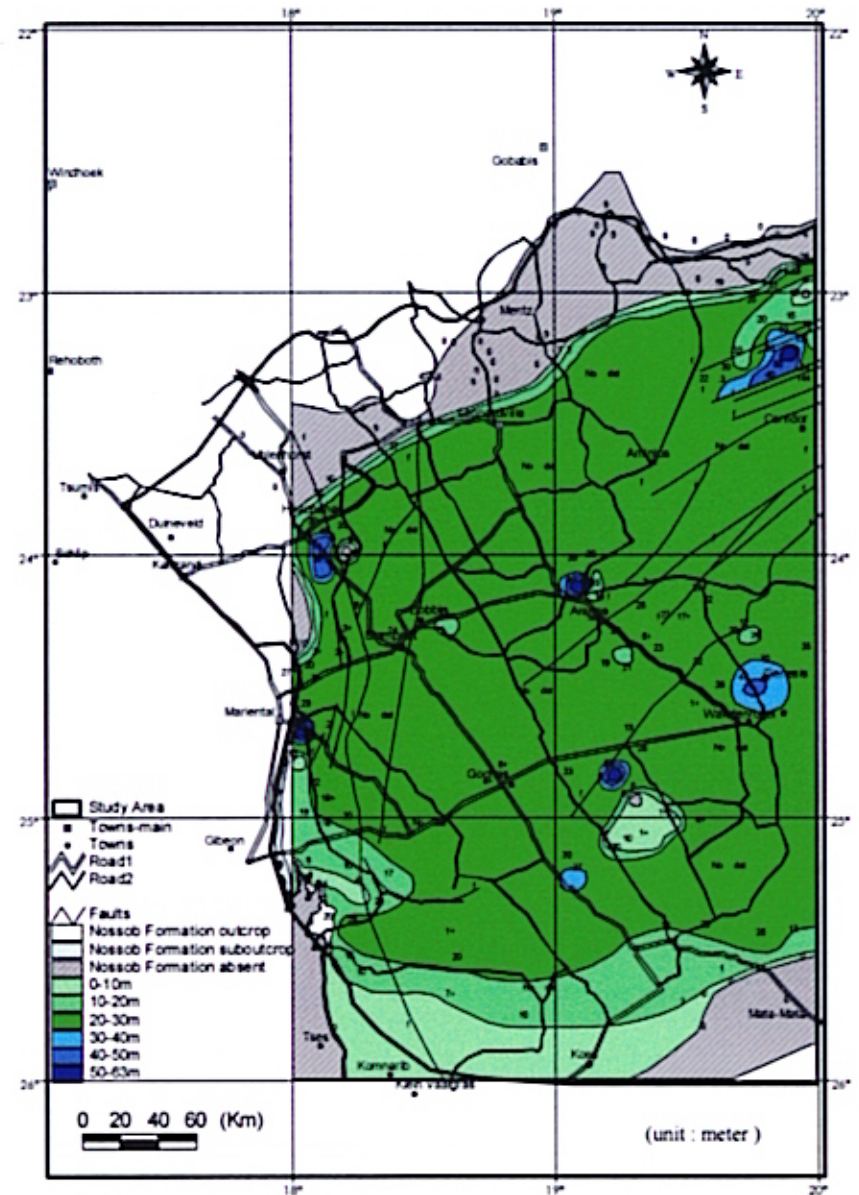
Fig. 3.6-8 Isopachs of Nossob Aquifer
