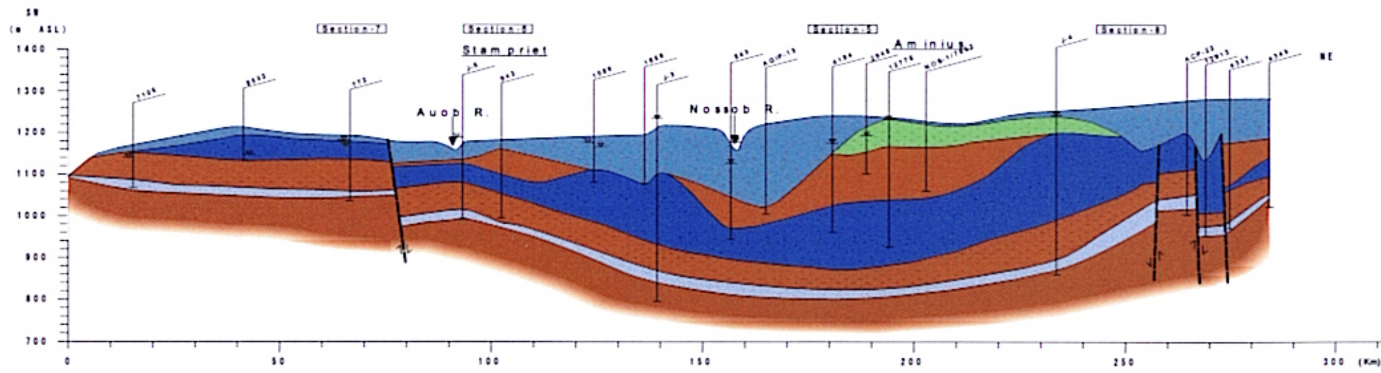
Fig. 3.6-9 (1) Hydrogeological Cross Section
