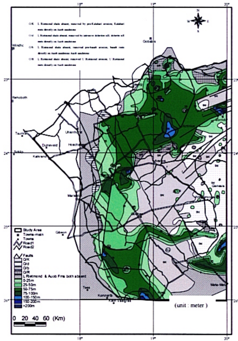
Fig. 3.6-3 Isopachs of Lower Rictmond Member
