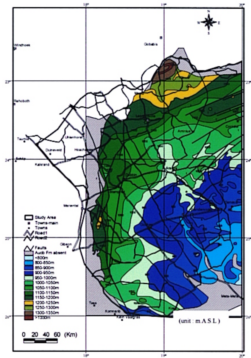
Fig. 3.6-4 Top of Auob Aquifer
