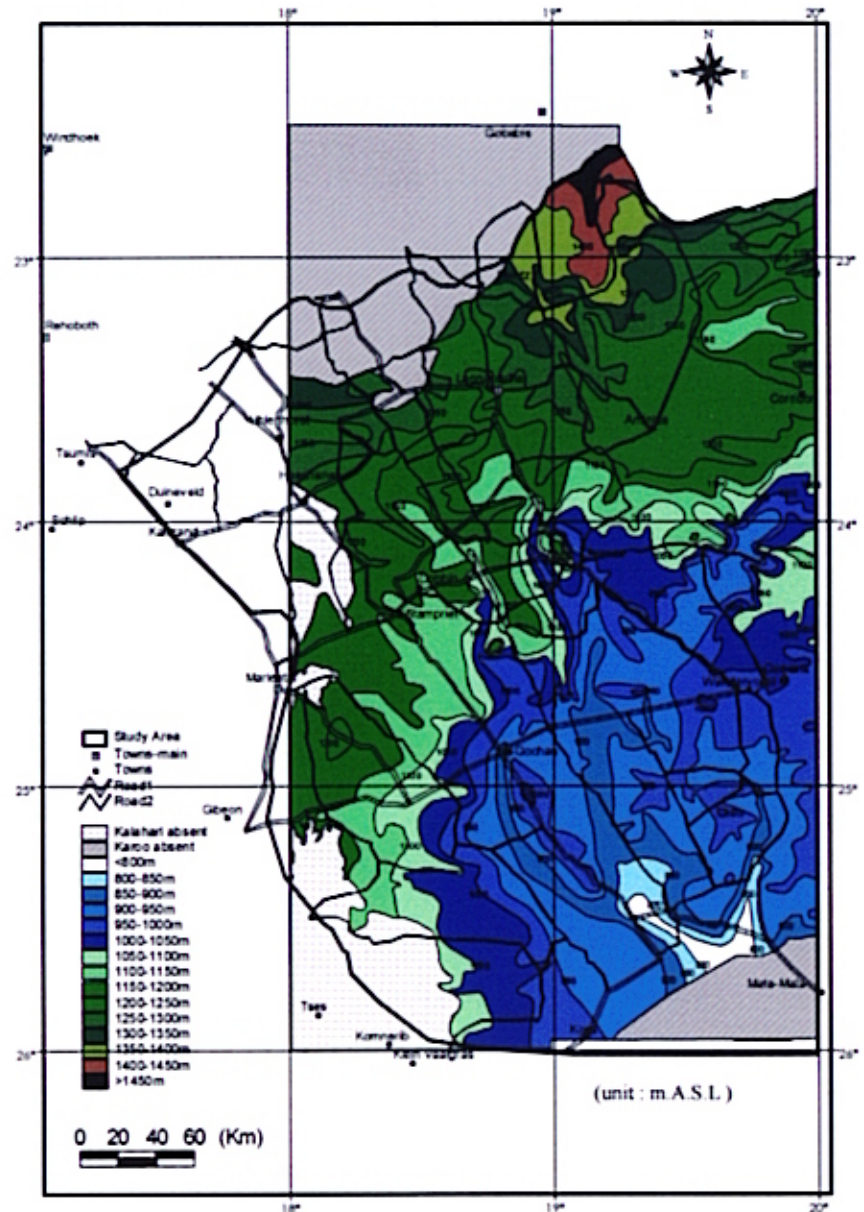
Fig. 3. 6-2 Bottom of Kalahari Beds
