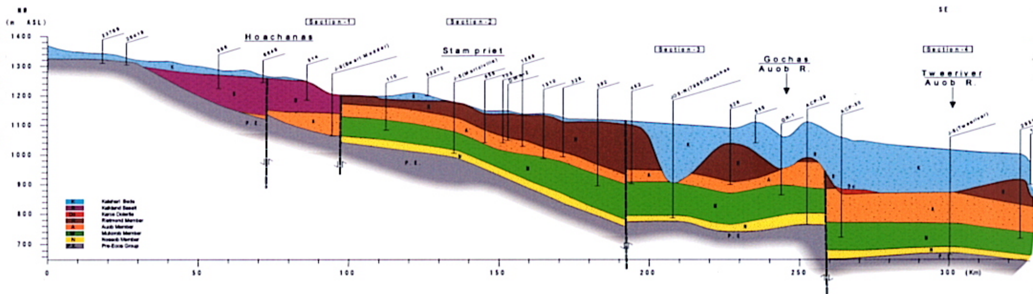
Geological Cross Section of the Study Area (3)
