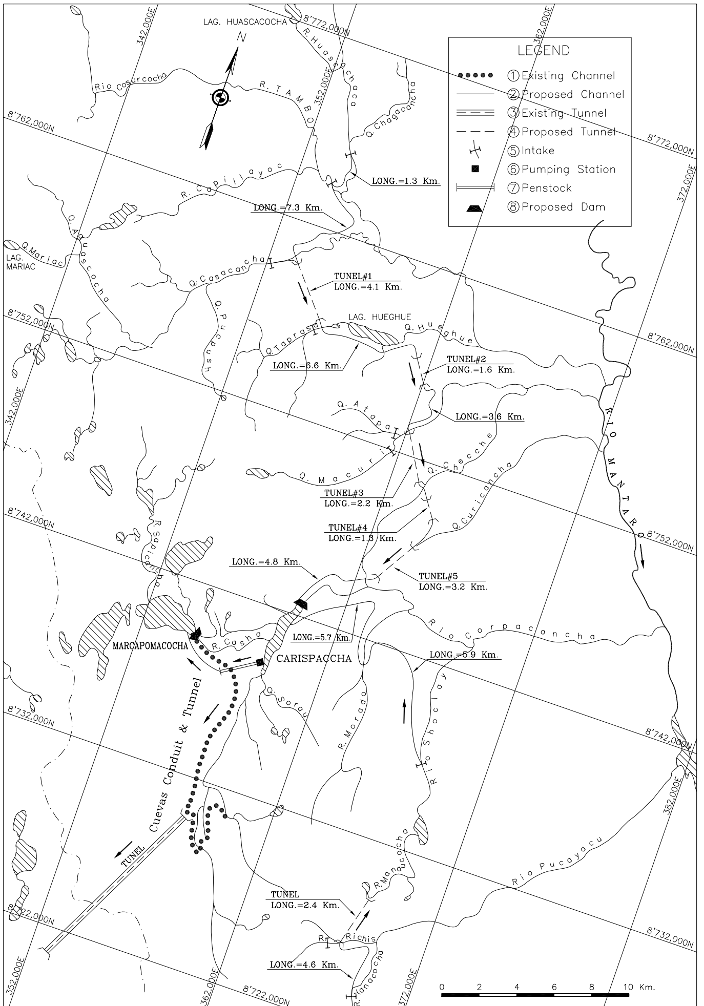
Figure 5.1.10 MANTARO WATER CONVEYANCE GENERAL PLAN (STAGE-1 & STAGE-2)
