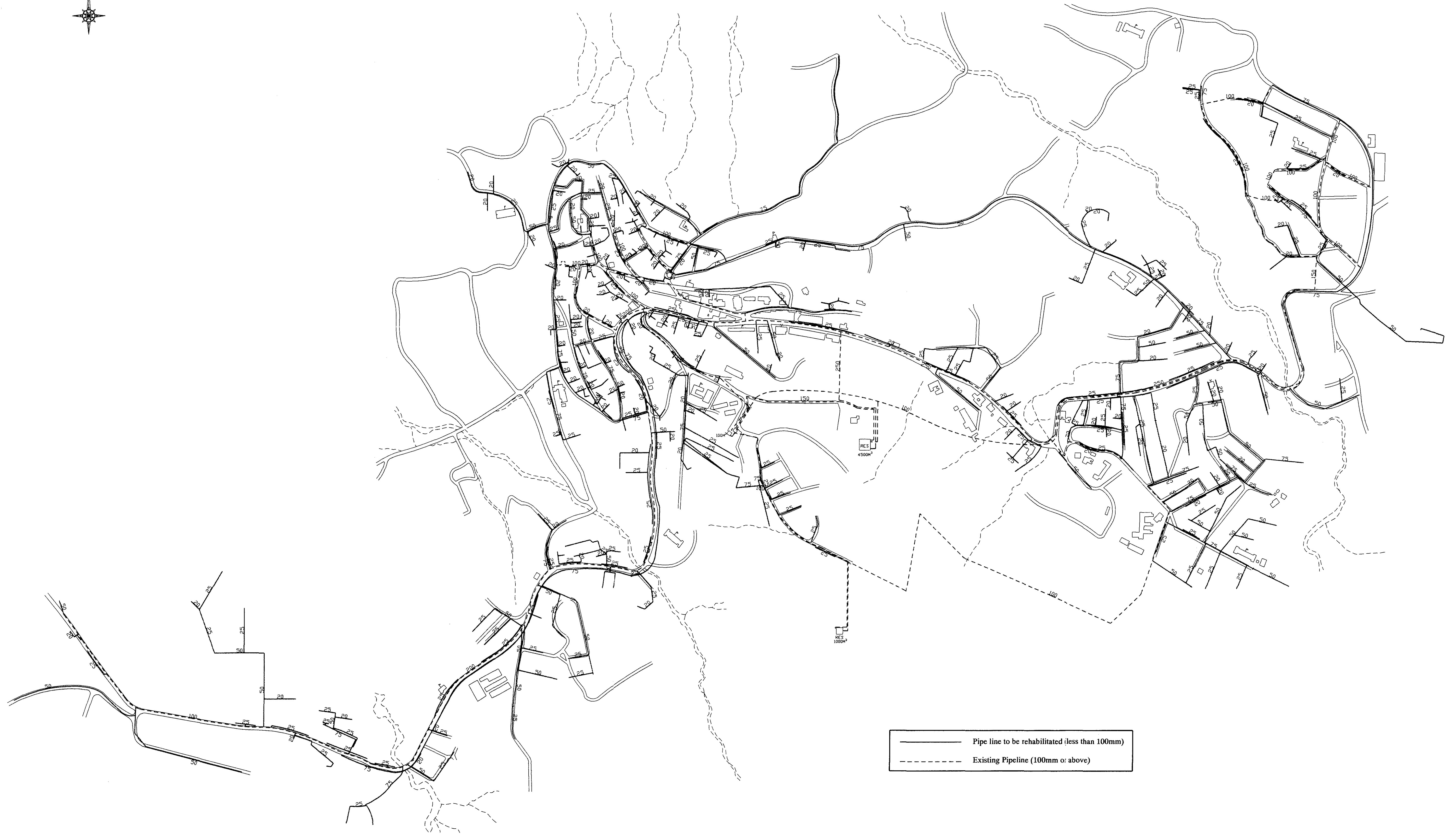
Fig. 4.4.5-1 Rehabilitation Plan for Tafilah City
