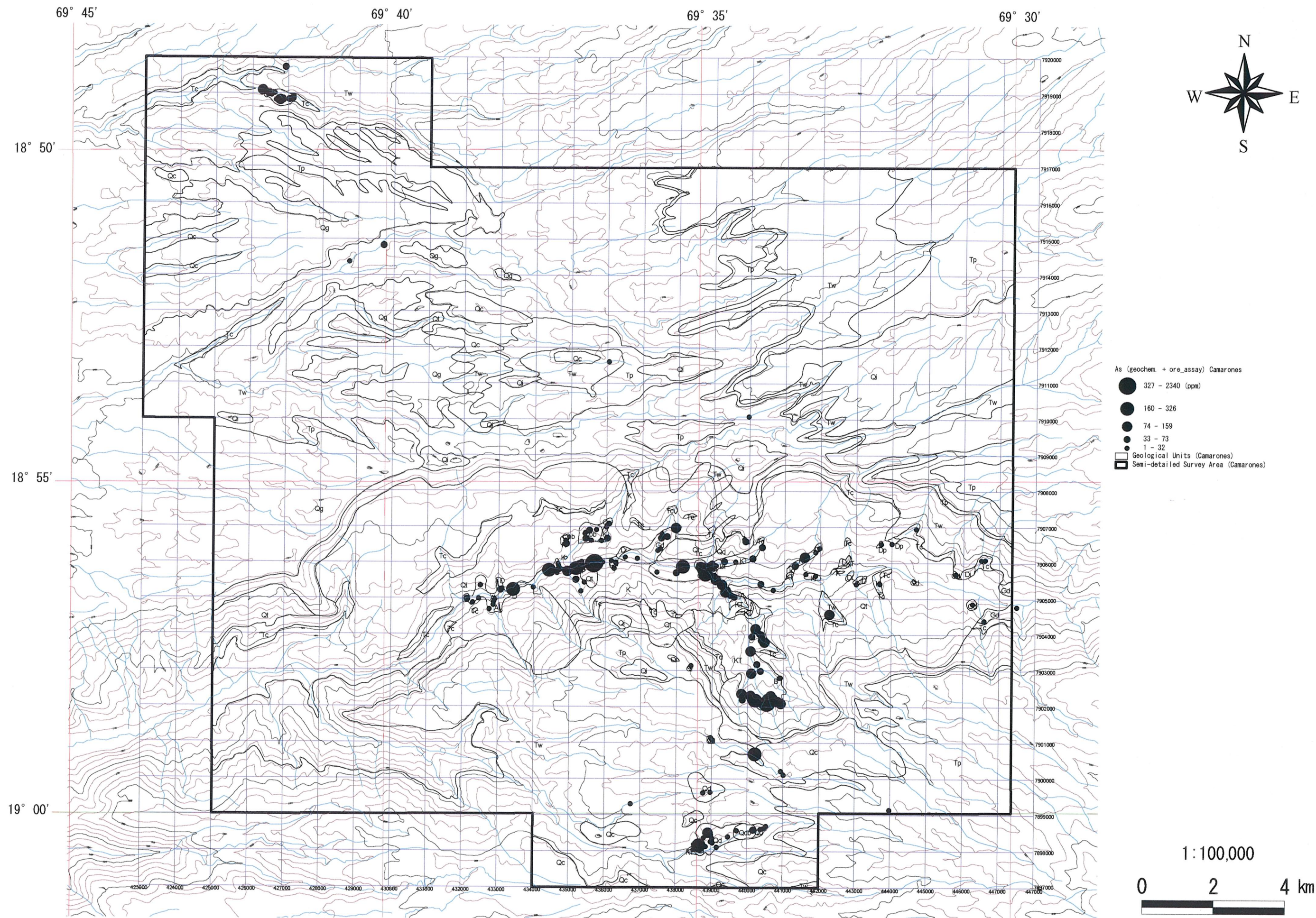
Fig. 2-2-43 (7) Geochemical Anomaly Map in the Camarones Area (As)
