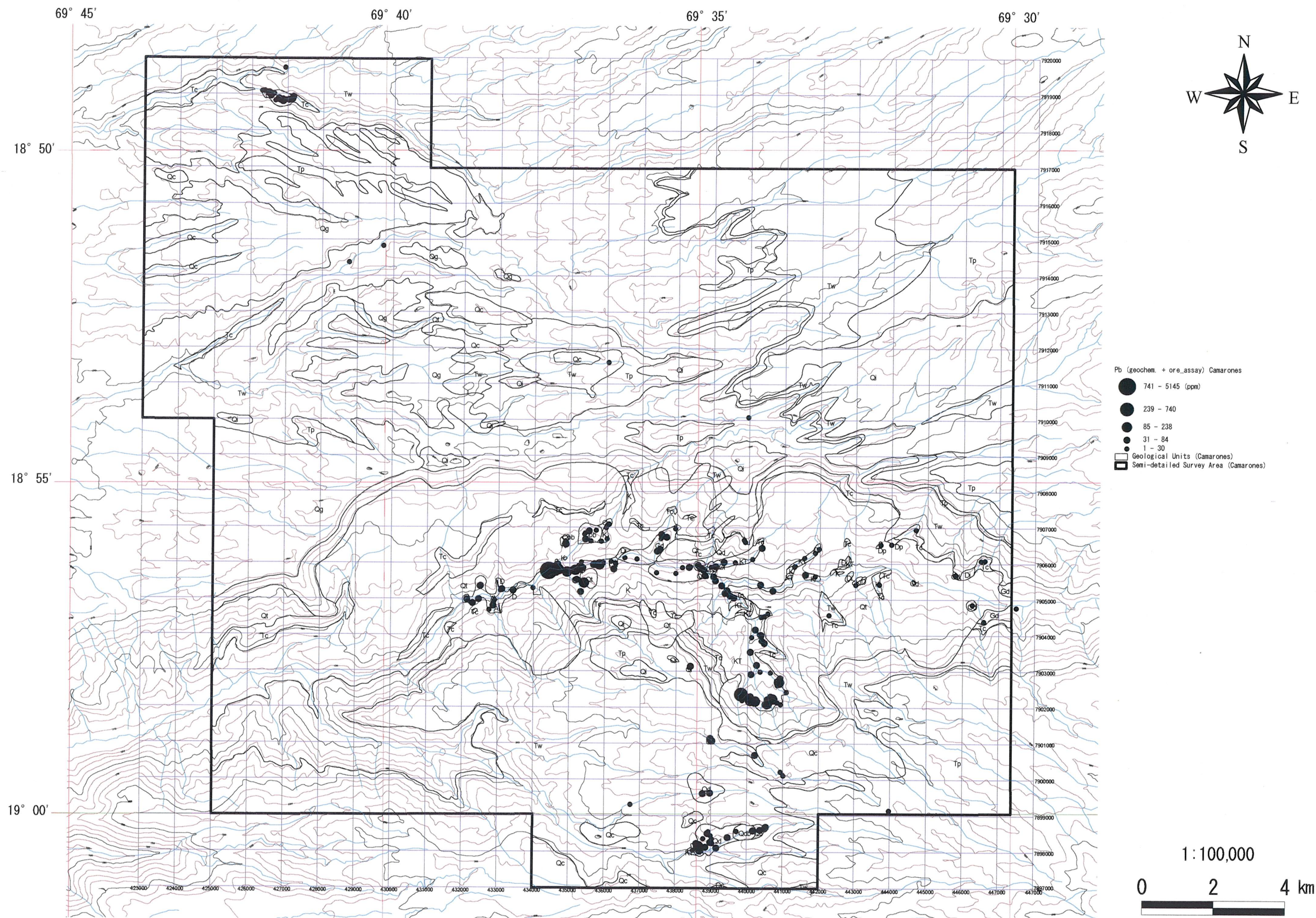
Fig. 2-2-43 (4) Geochemical Anomaly Map in the Camarones Area (Pb)
