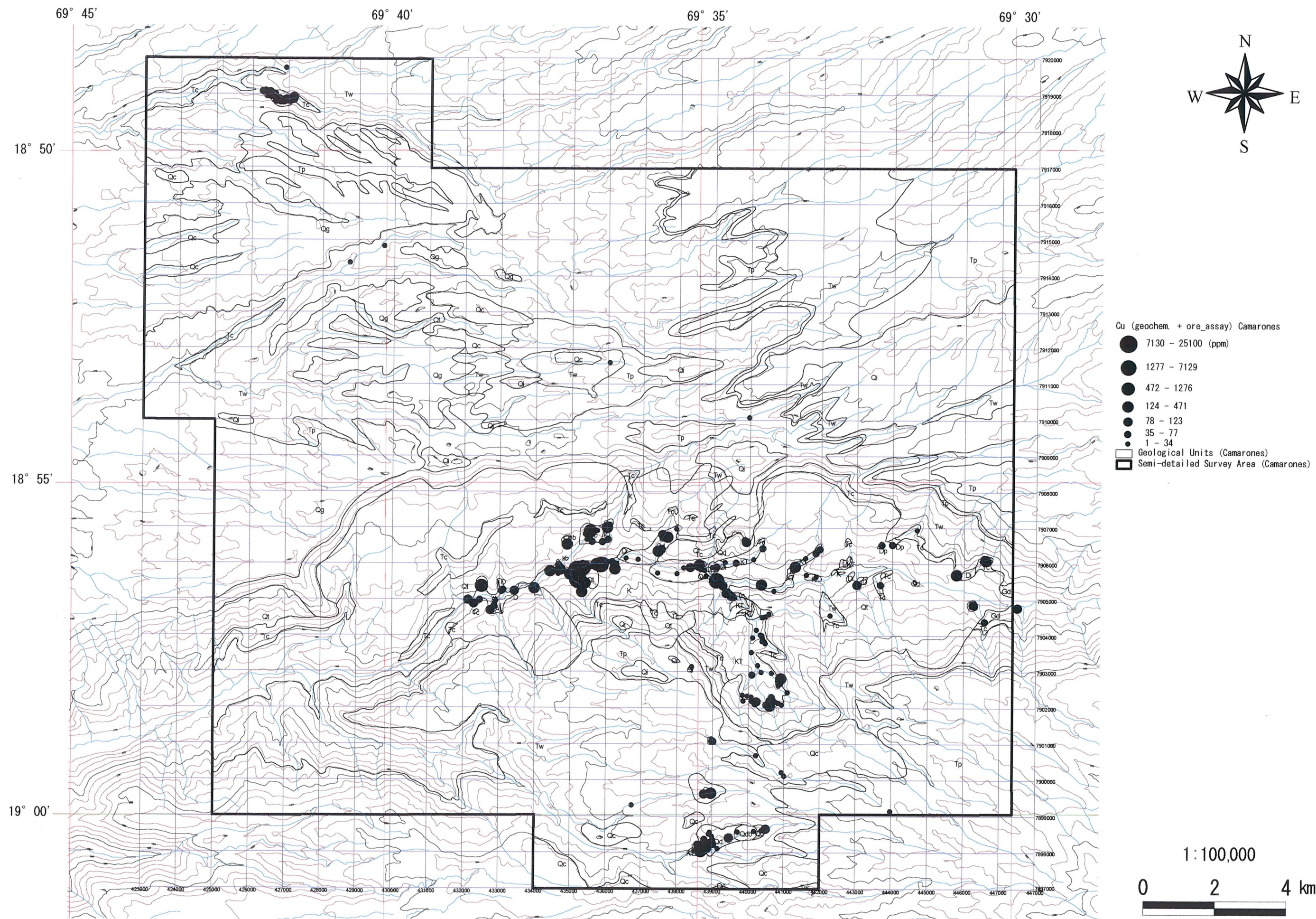
Fig. 2-2-43 (3) Geochemical Anomaly Map in the Camarones Area (Cu)
