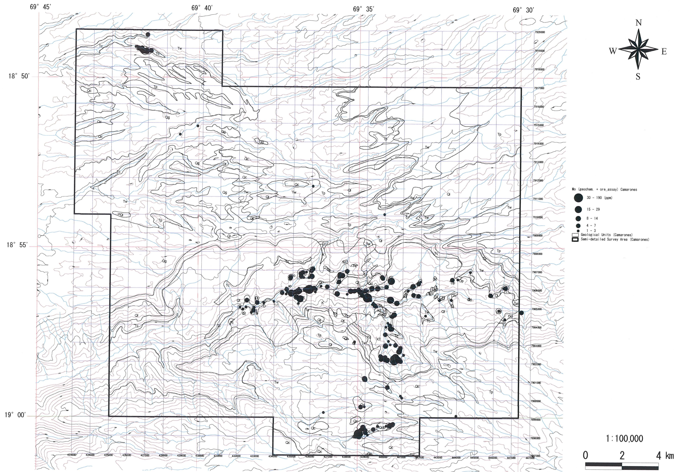
Fig. 2-2-43 (6) Geochemical Anomaly Map in the Camarones Area (Mo)
