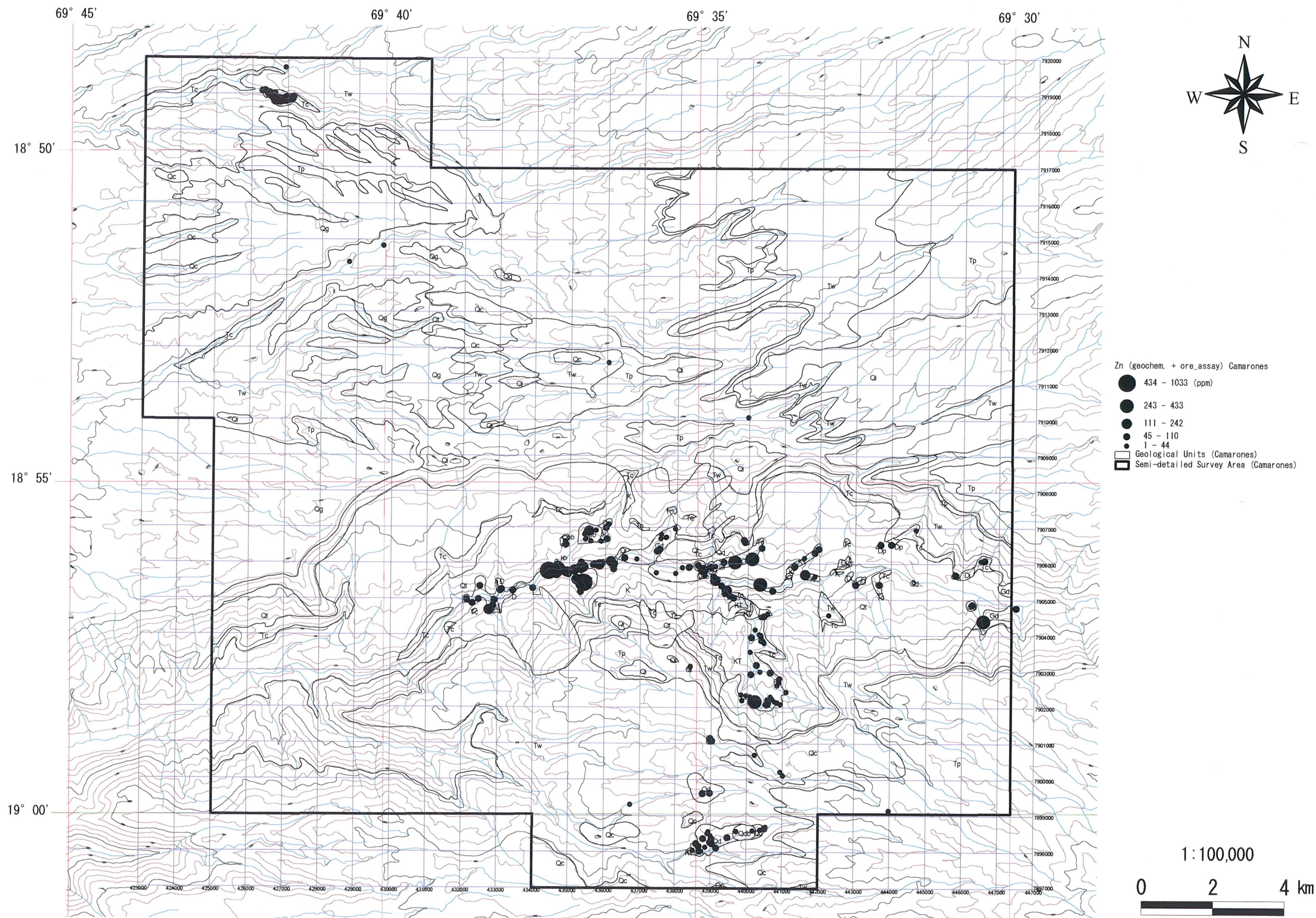
Fig. 2-2-43 (5) Geochemical Anomaly Map in the Camarones Area (Zn)
