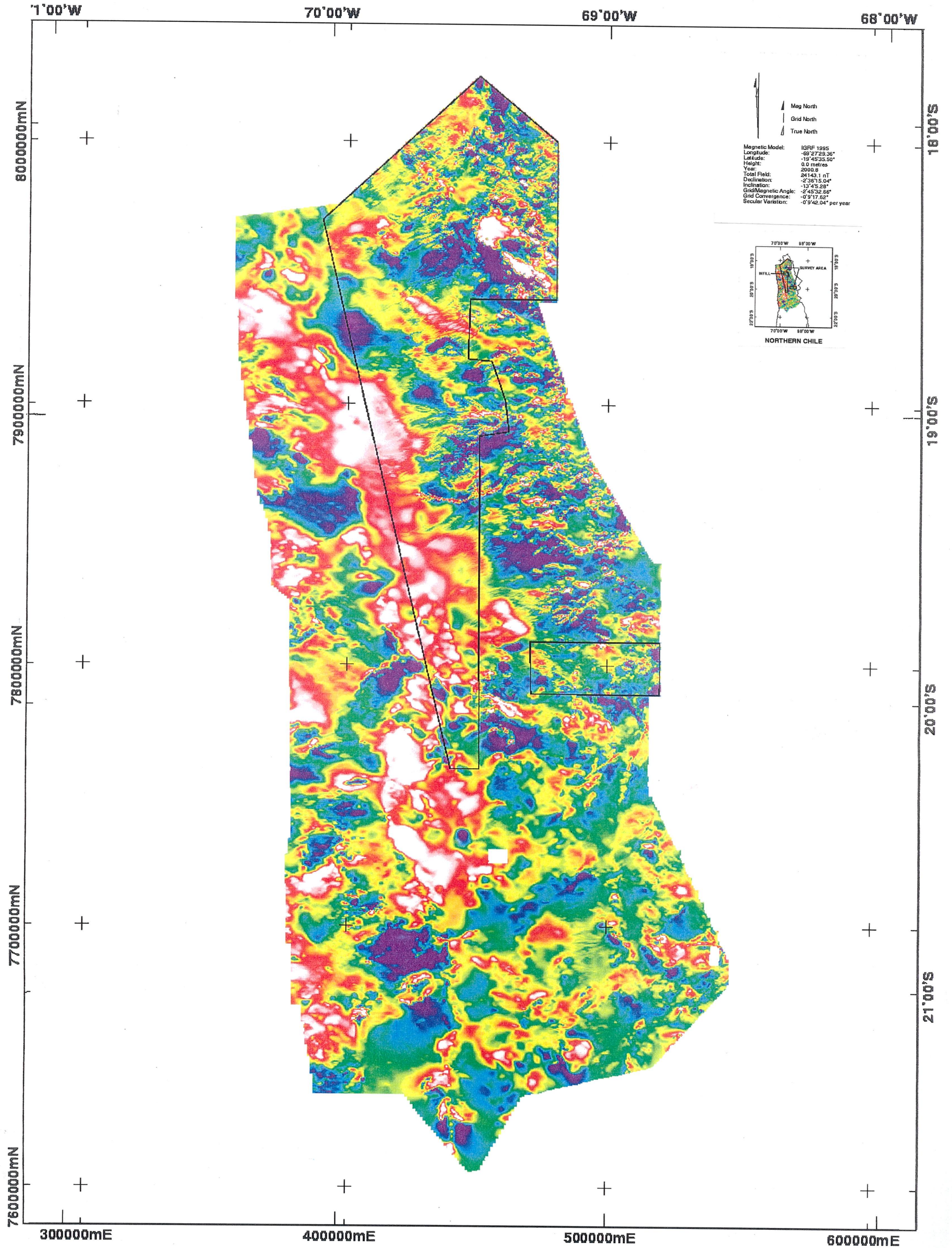
AP-9 Total Magnetic Intensity (Reduced to the Pole)
