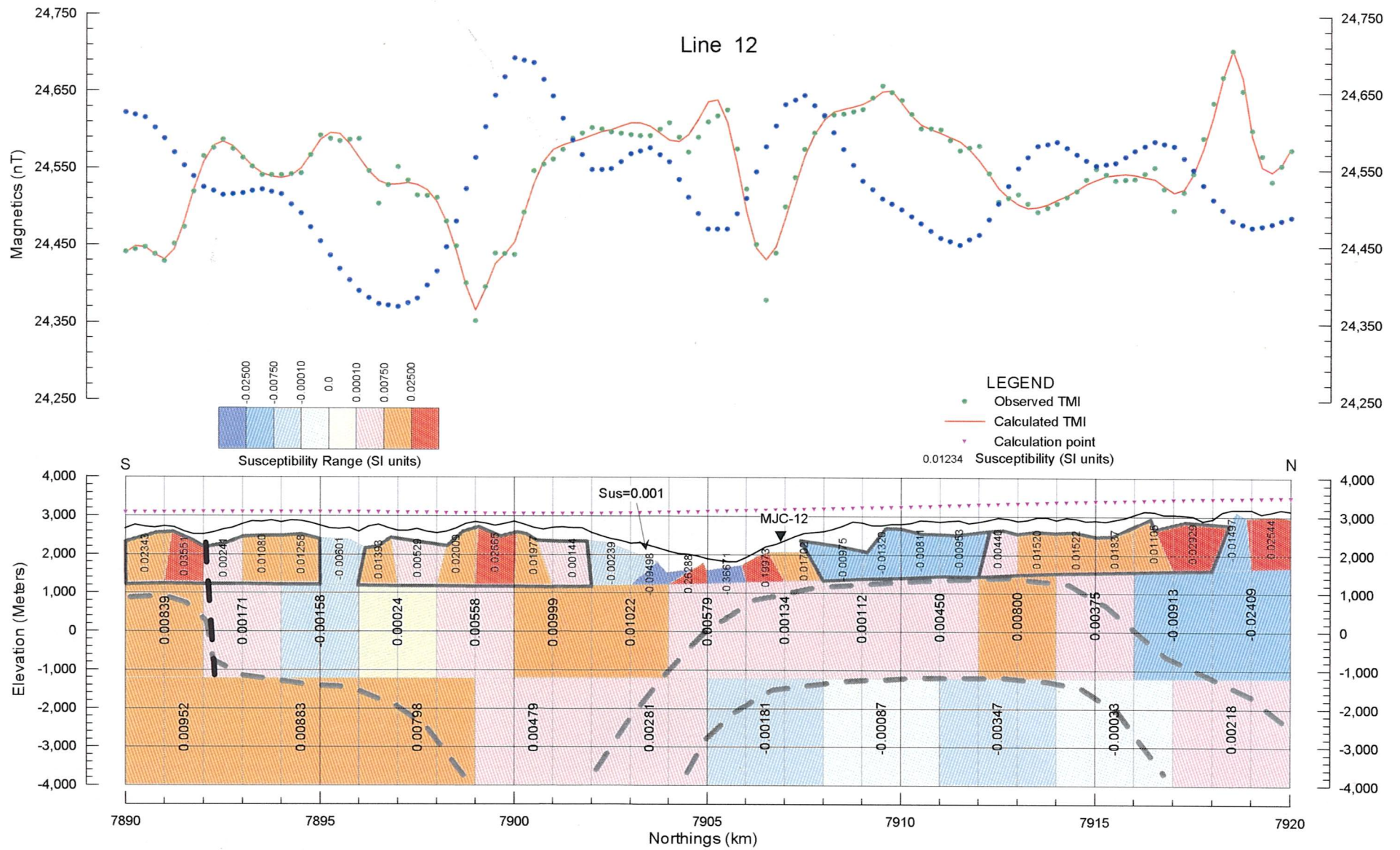
Fig. 2-6-35 Line 12 - 2D Model Profile
