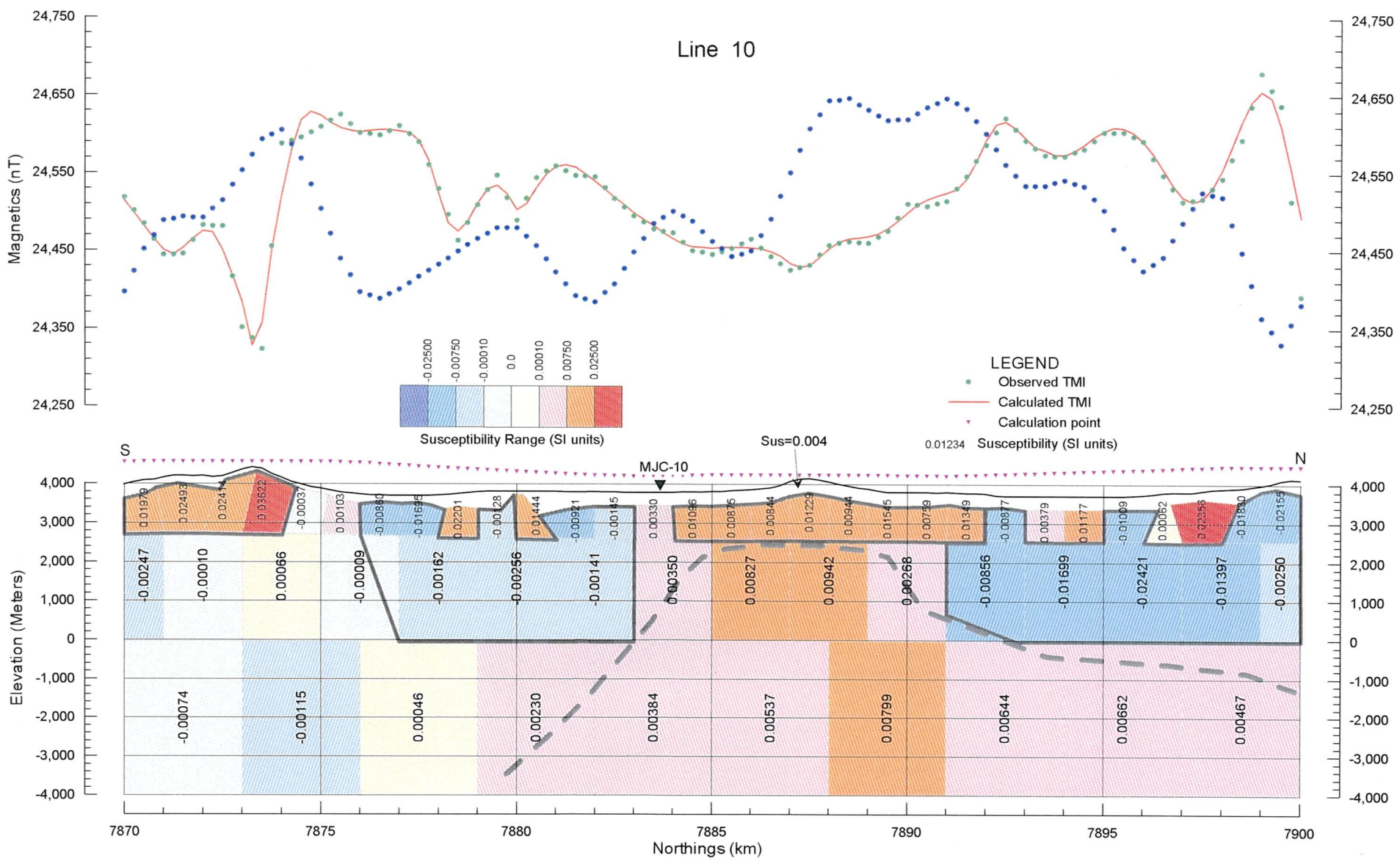
Fig. 2-6-33 Line 10 - 2D Model Profile
