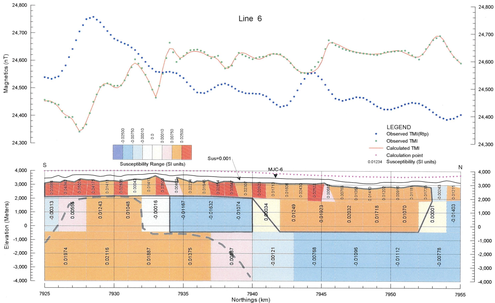
Fig. 2-6-29 Line 6 - 2D Model Profile
