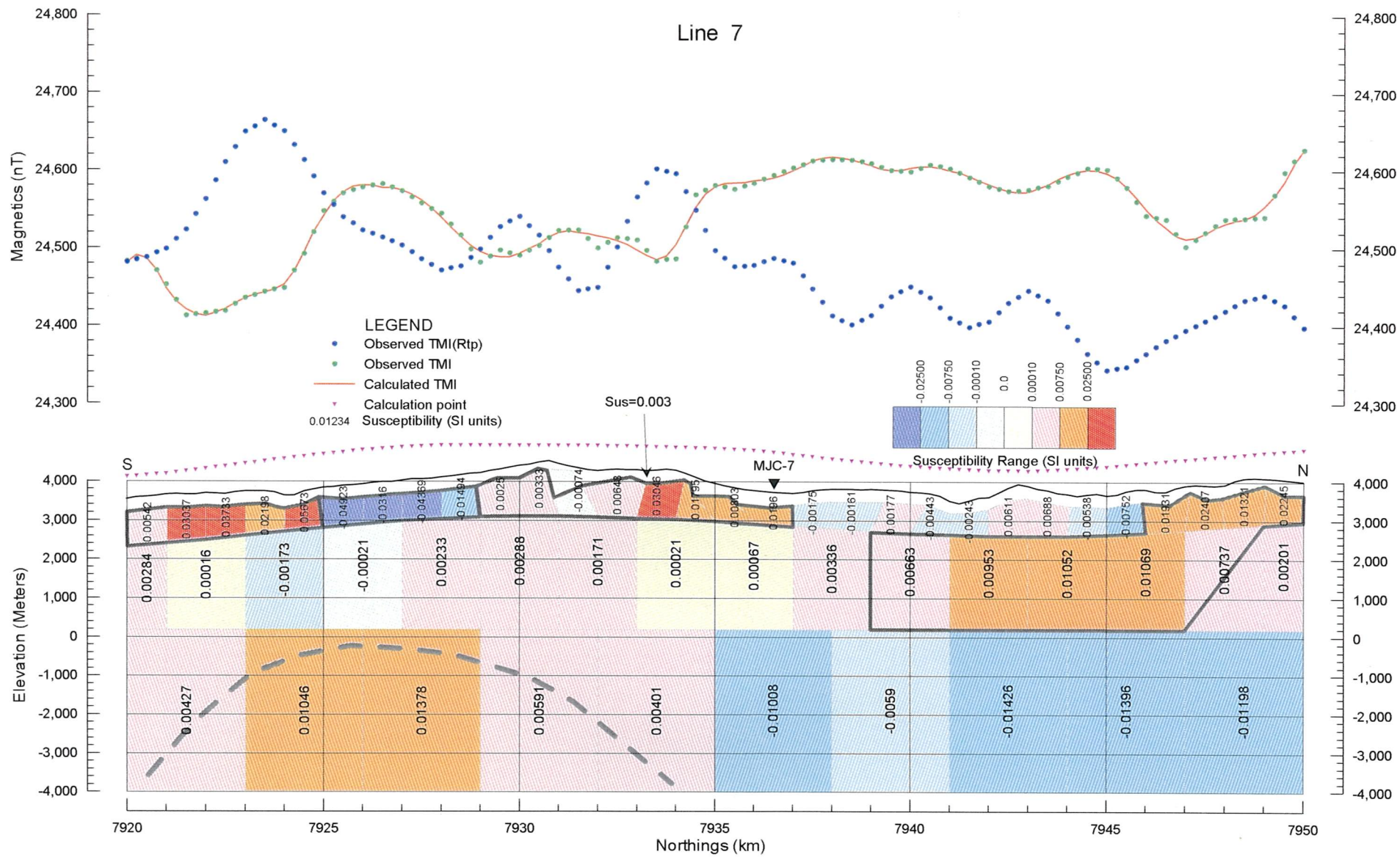
Fig. 2-6-30 Line 7 - 2D Model Profile
