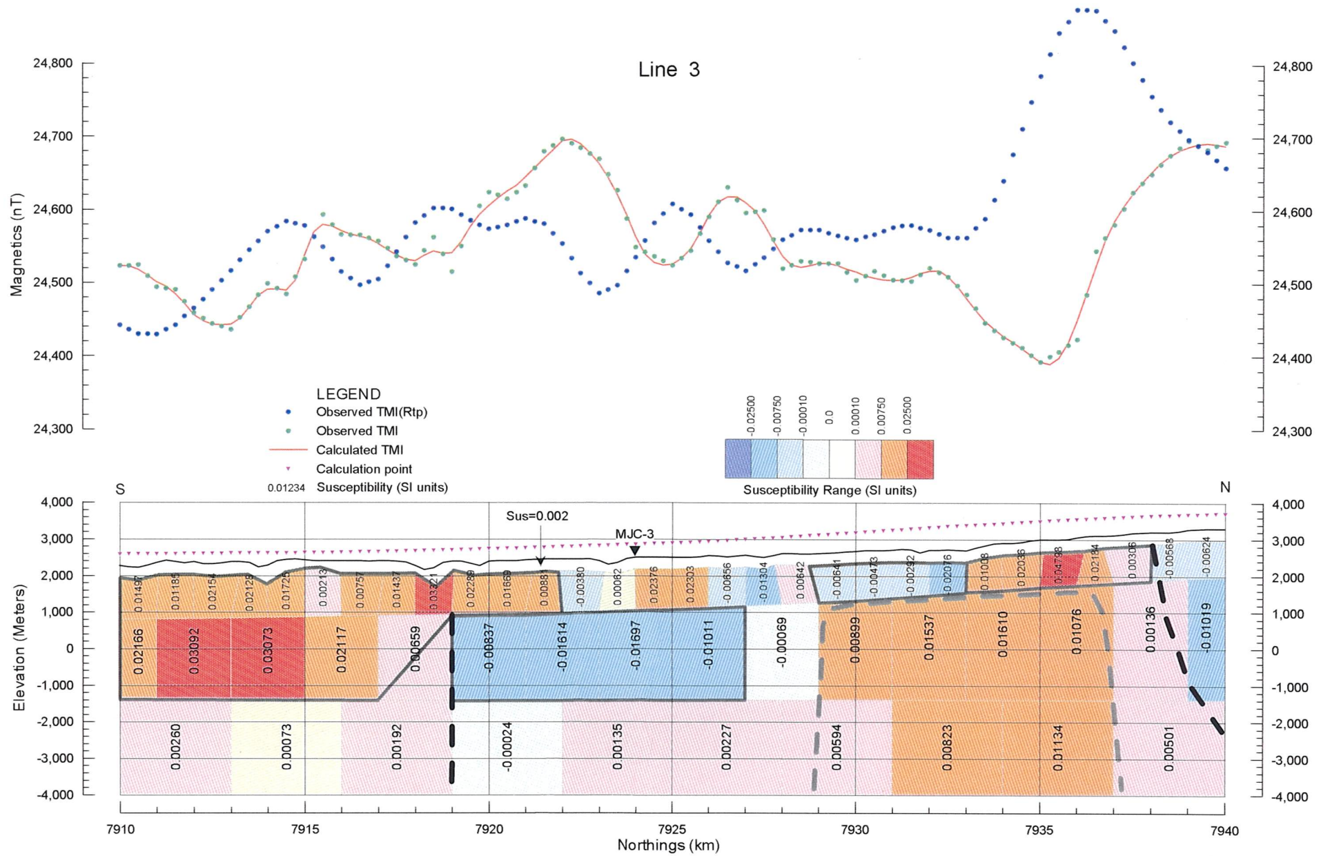
Fig. 2-6-26 Line 3 - 2D Model Profile
