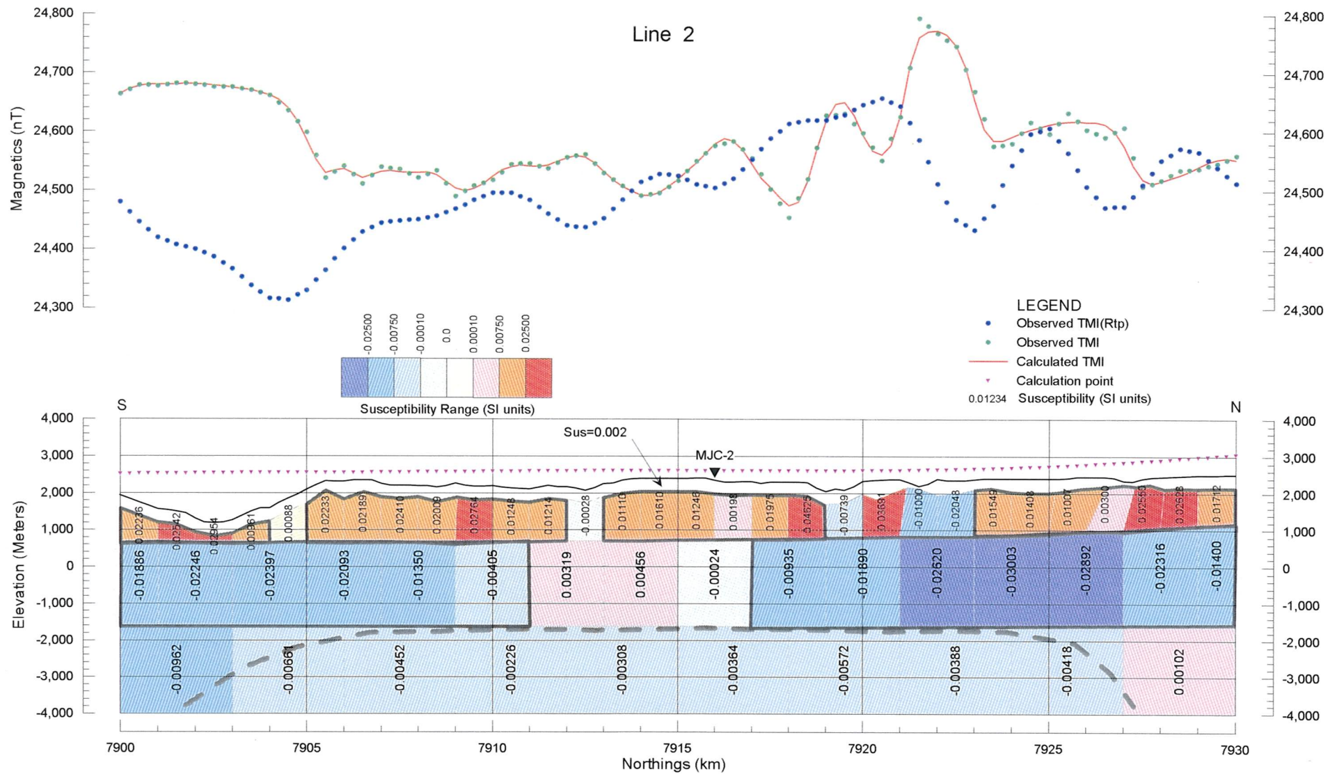
Fig. 2-6-25 Line 2 - 2D Model Profile
