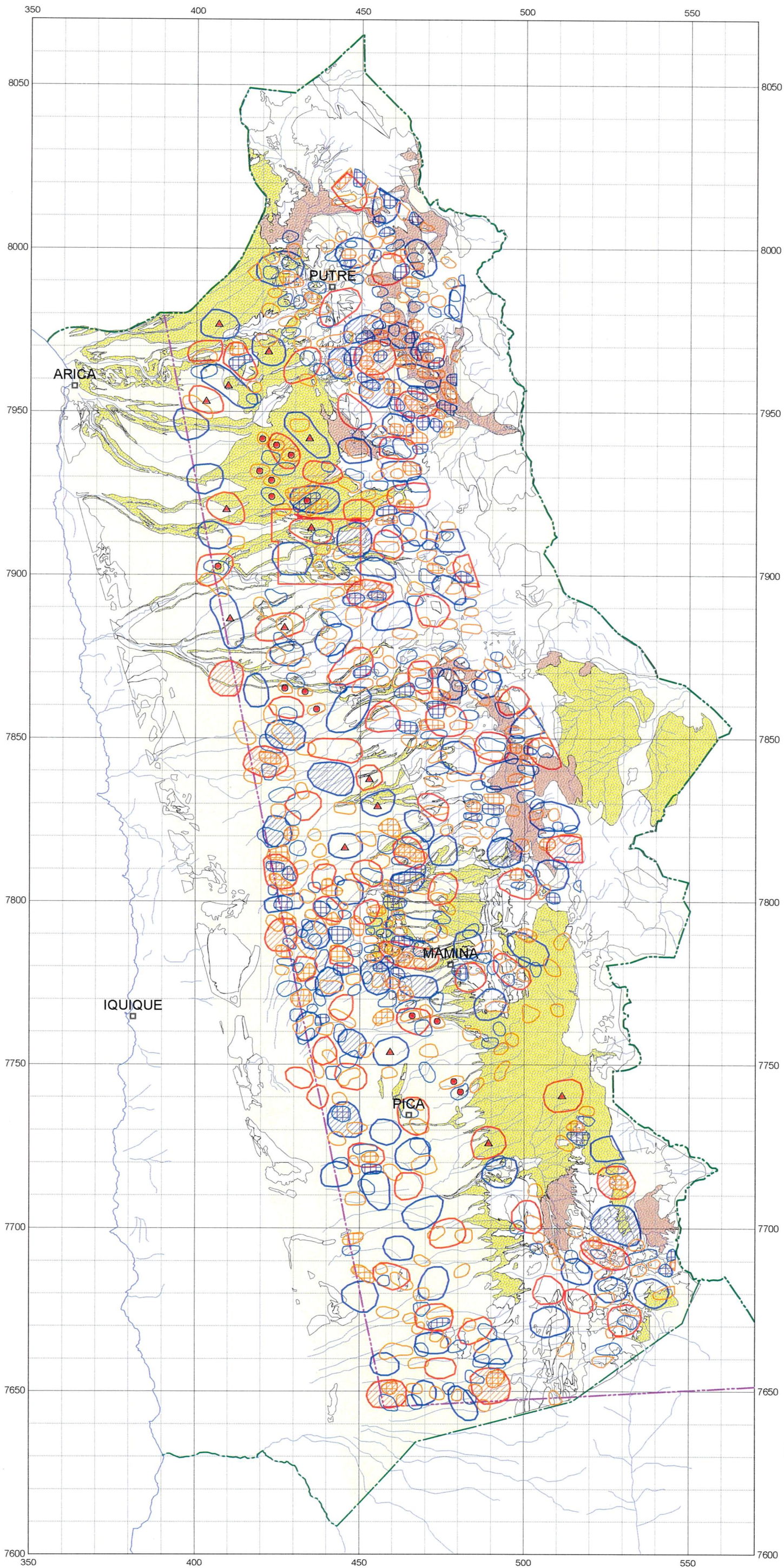
Fig.2-6-18 SW&MW Magnetic Anomalies and Tertiary-Quaternary Ignimbrites
