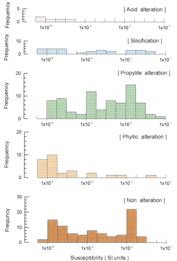
Fig. 2-6-11 Histogram of Susceptibility by Alteration Type
