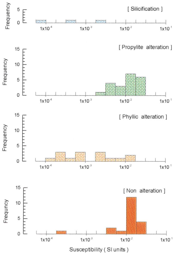
Fig. 2-6-11 Histogram of Susceptibility by Alteration Type
