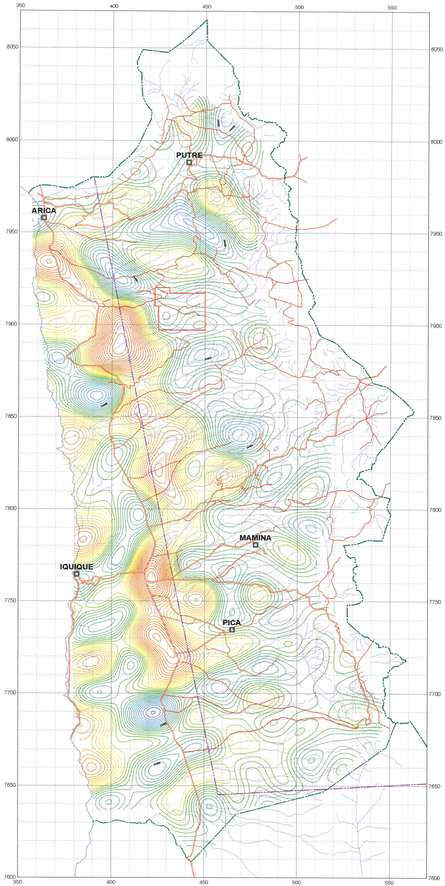
Fig.2-6-6 Long Wavelength Reduced to the Pole
