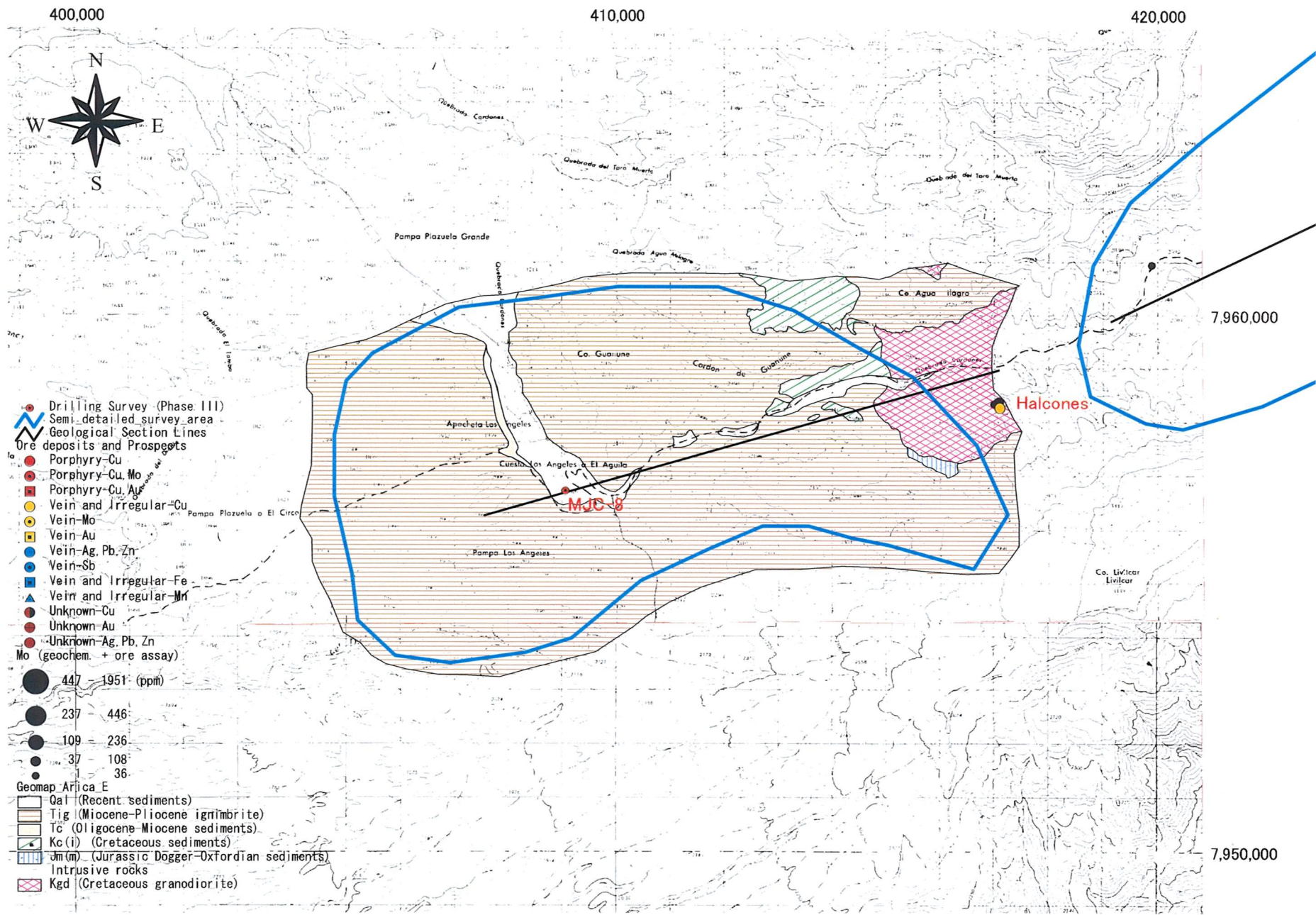
Fig. 2-2-94 (6) Geochemical Anomaly Map in the Area to the East of Arica (Mo)
