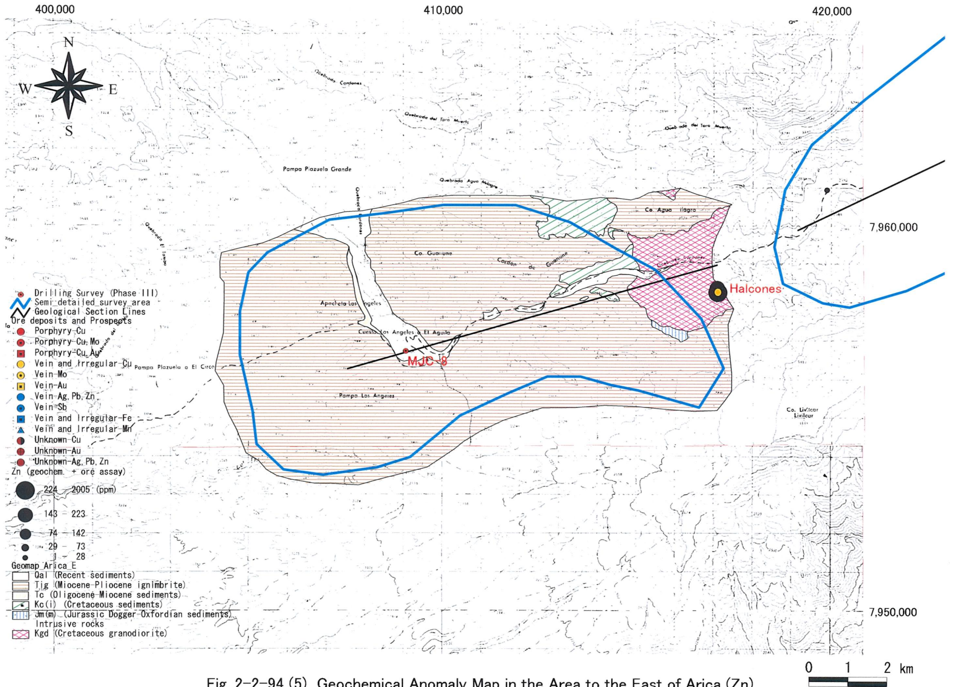
Fig. 2-2-94 (5) Geochemical Anomaly Map in the Area to the East of Arica (Zn)
