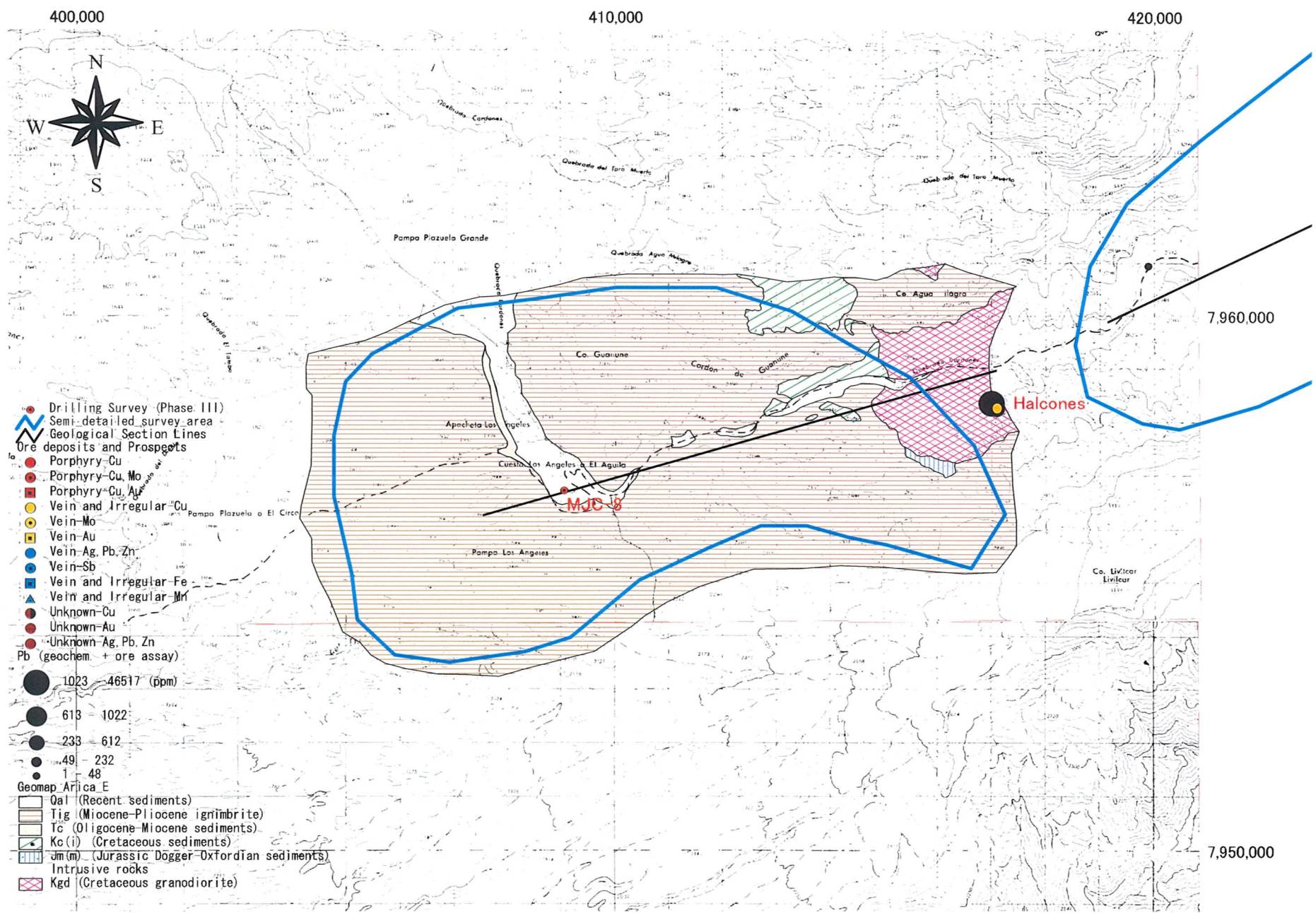
Fig. 2-2-94 (4) Geochemical Anomaly Map in the Area to the East of Arica (Pb)
