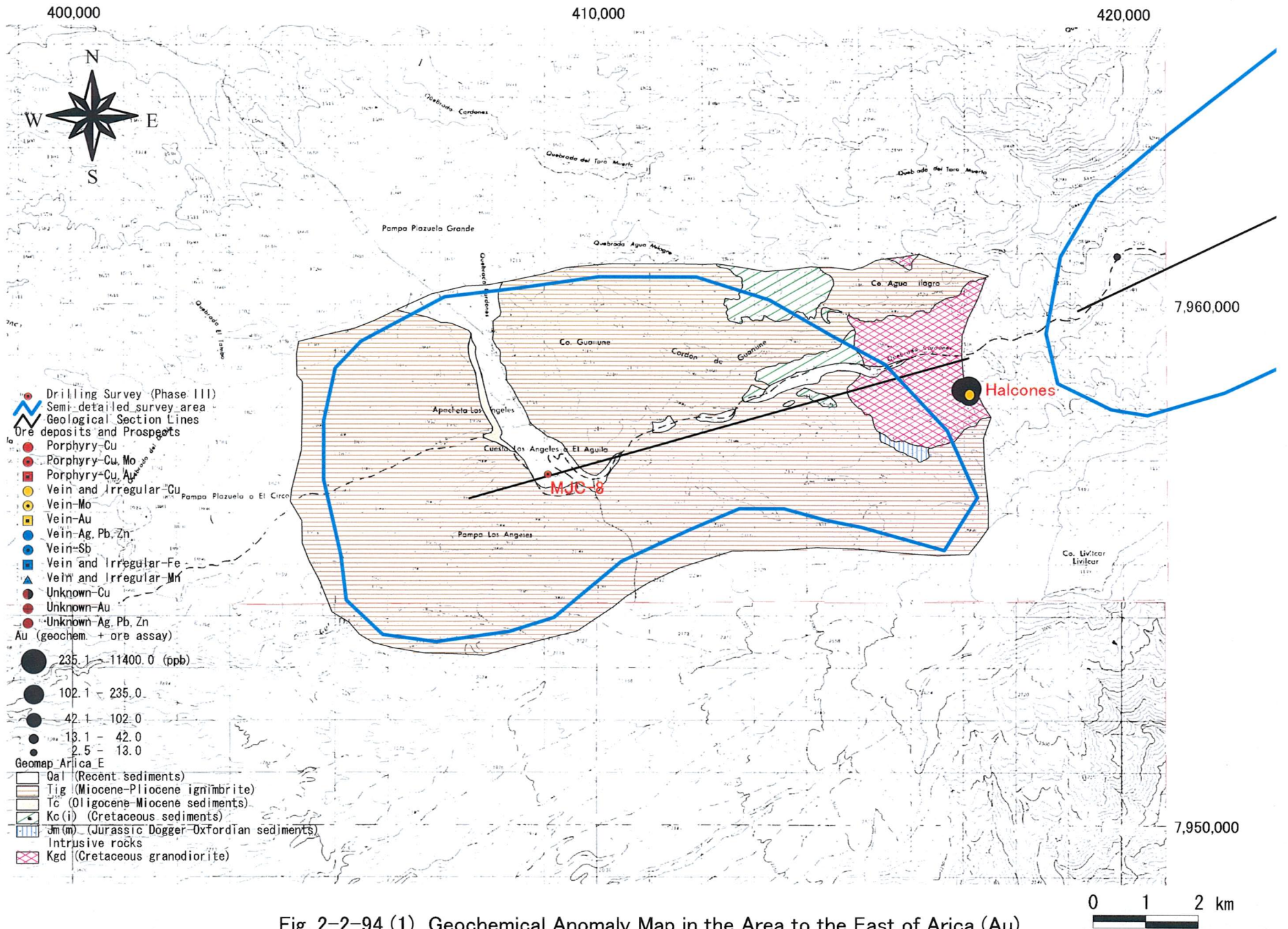
Fig. 2-2-94 (1) Geochemical Anomaly Map in the Area to the East of Arica (Au)
