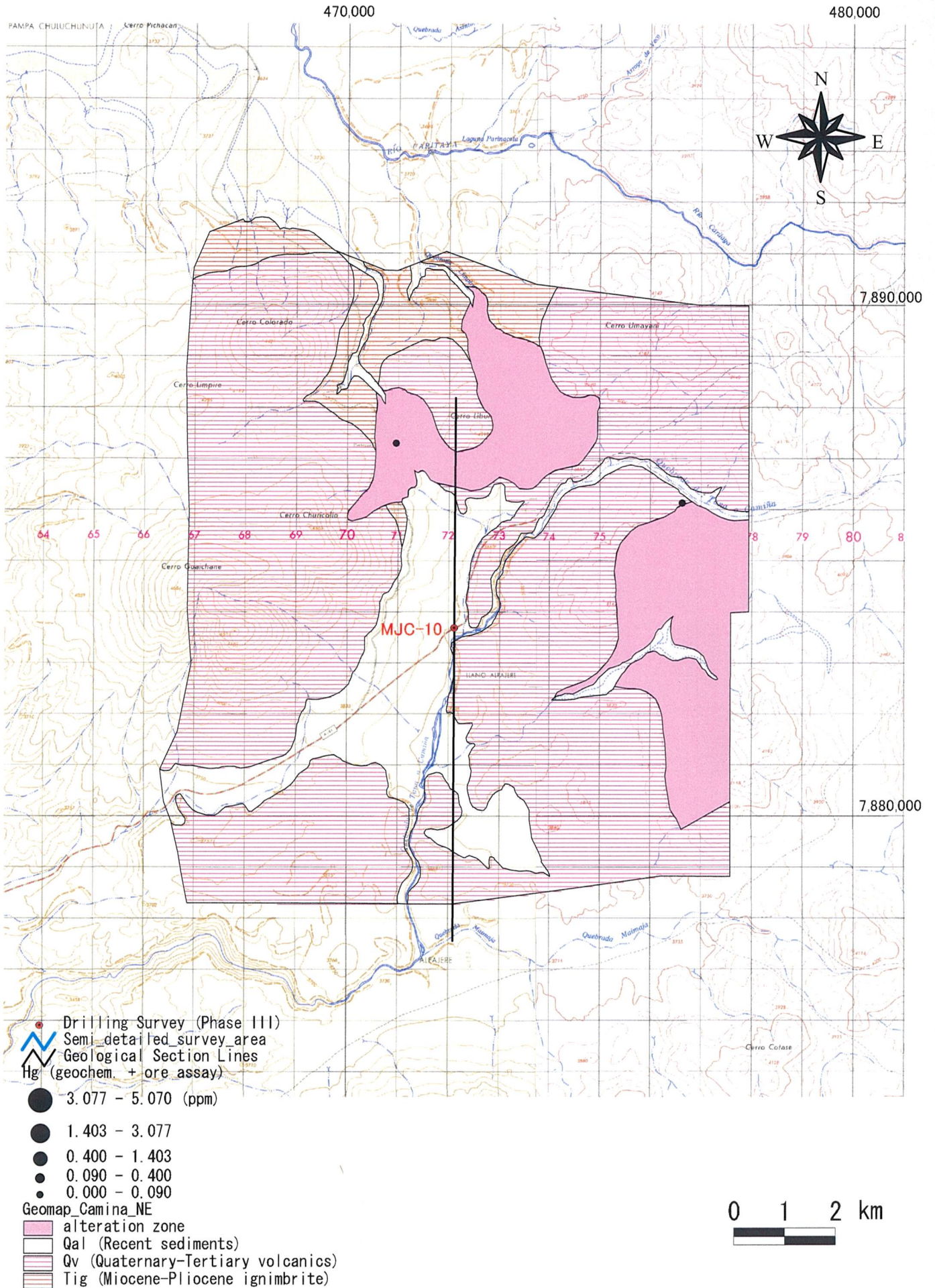
Fig. 2-2-70 (2) Geochemical Anomaly Map in the Area to the Northeast of Camina (Hg)
