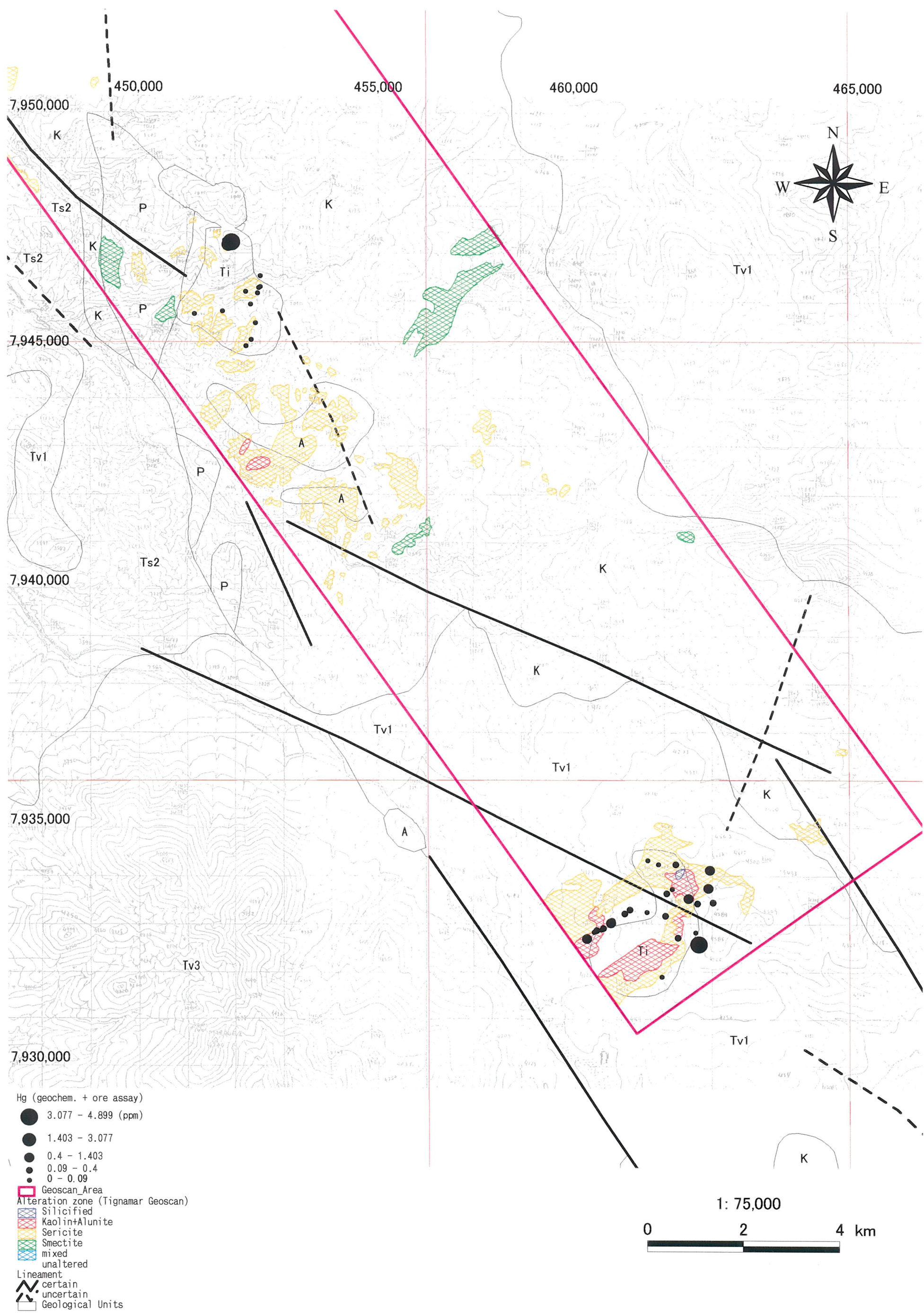
Fig. 2-2-35 (4) Geochemical Anomaly Map in the Tignamar Area (Hg)
