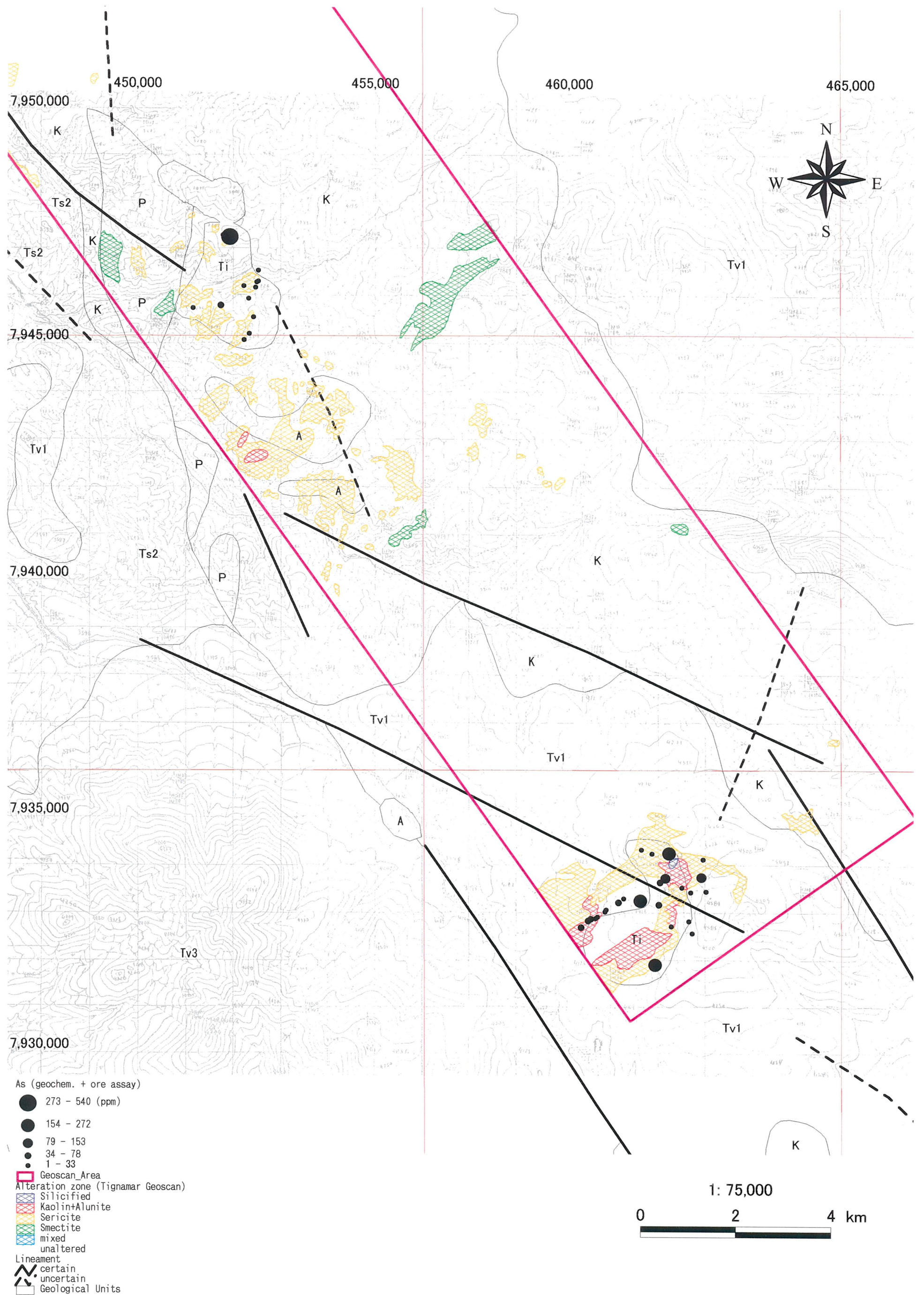
Fig. 2-2-35 (3) Geochemical Anomaly Map in the Tignamar Area (As)
