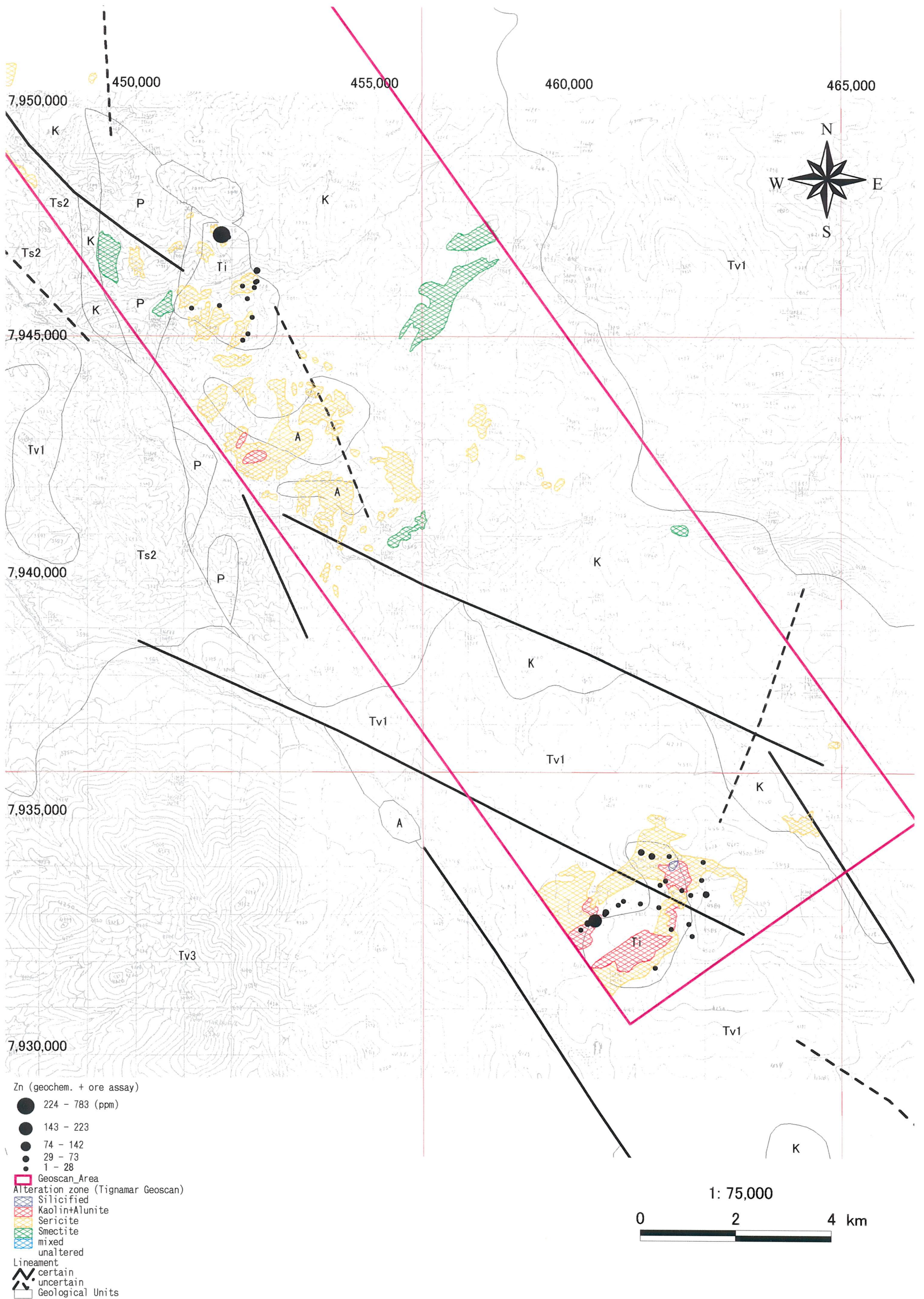
Fig. 2-2-35 (2) Geochemical Anomaly Map in the Tignamar Area (Zn)
