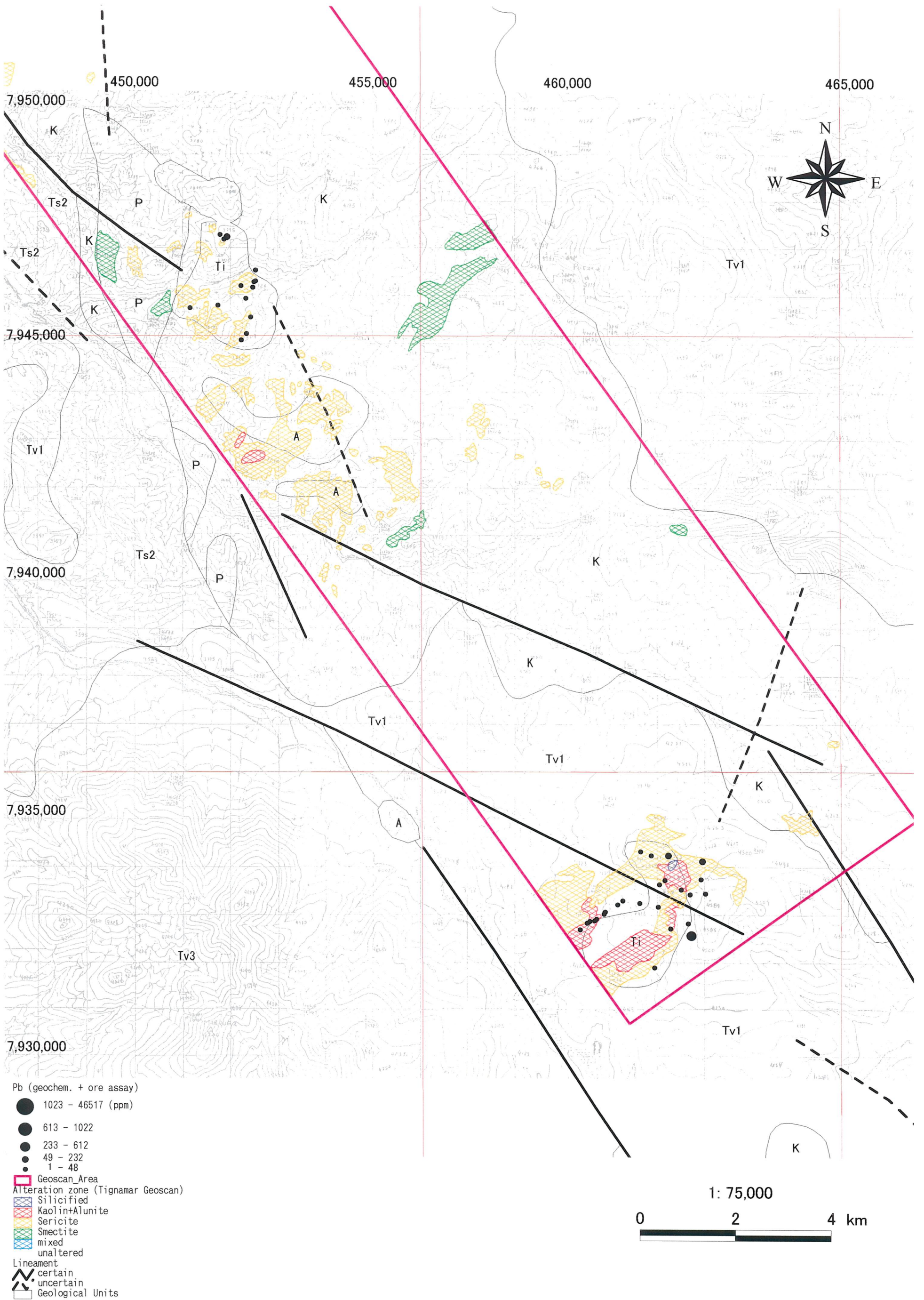
Fig. 2-2-35 (1) Geochemical Anomaly Map in the Tignamar Area (Pb)
