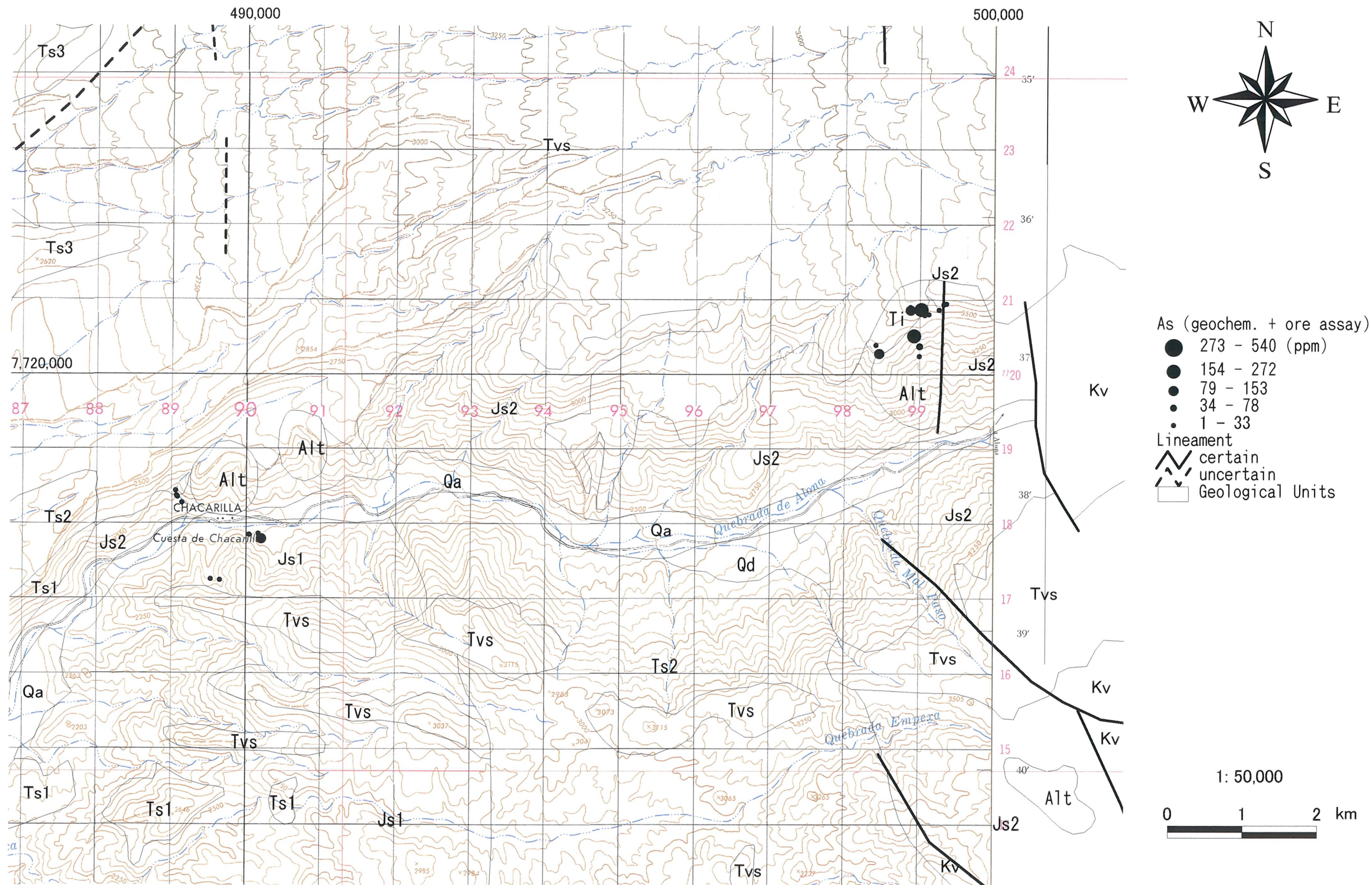
Fig. 2-2-25 (2) Geochemical Anomaly Map in the Chacarilla Area (As)
