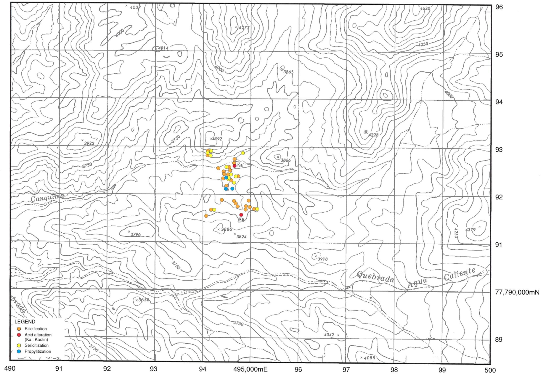
Fig. 2-2-14 Distribution Map of Alteration Minerals the Diana Area
