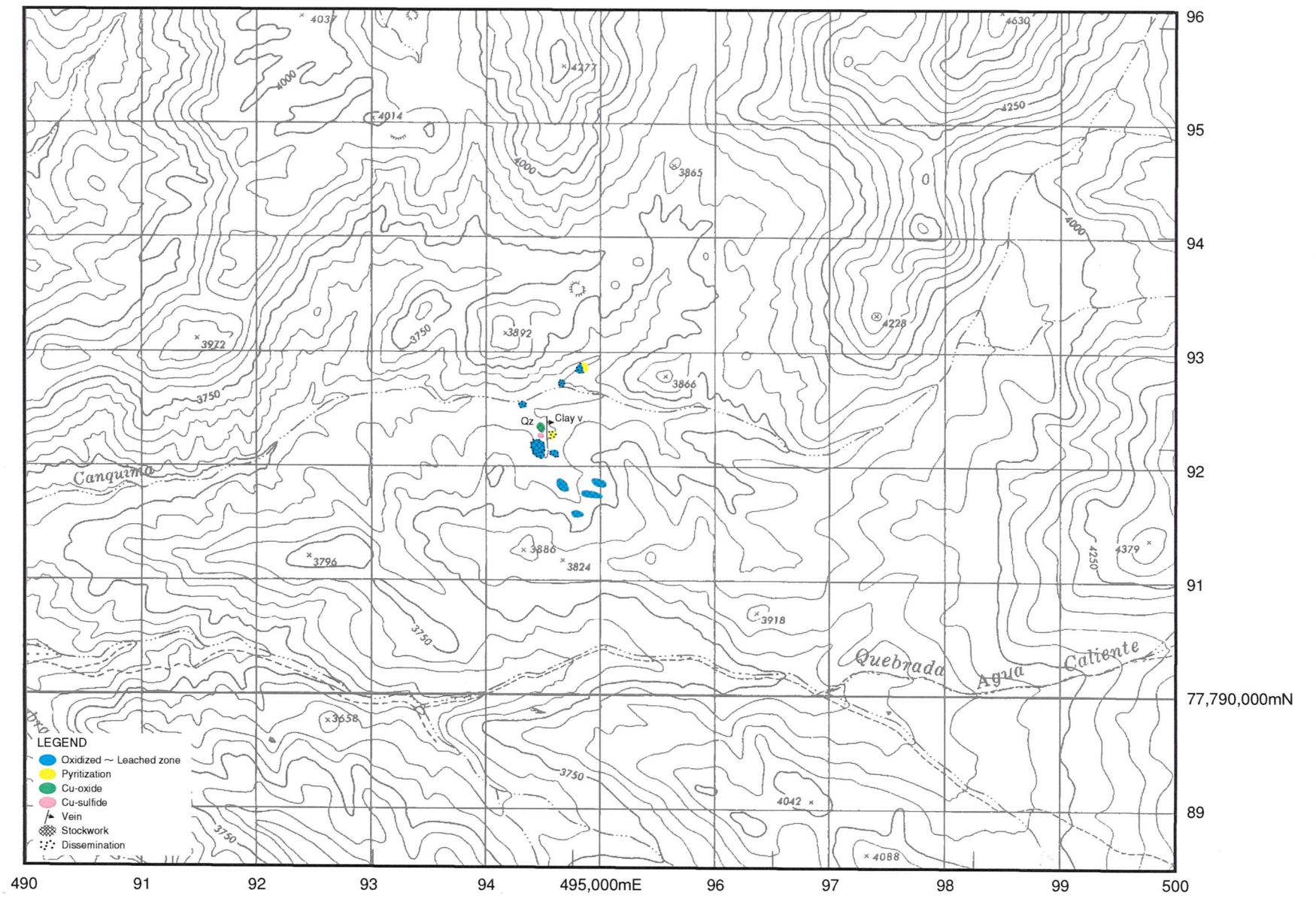
Fig. 2-2-13 Mineralization Map of the Diana Area
