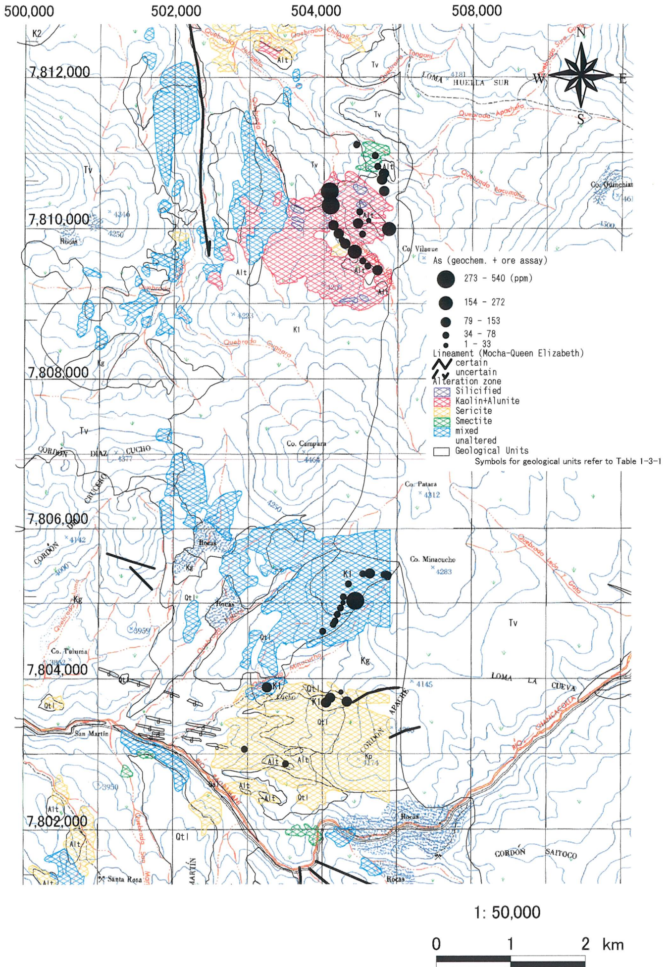
Fig. 2-2-10 (7) Geochemical Anomaly Map in the Queen Elizabeth Area (As)
