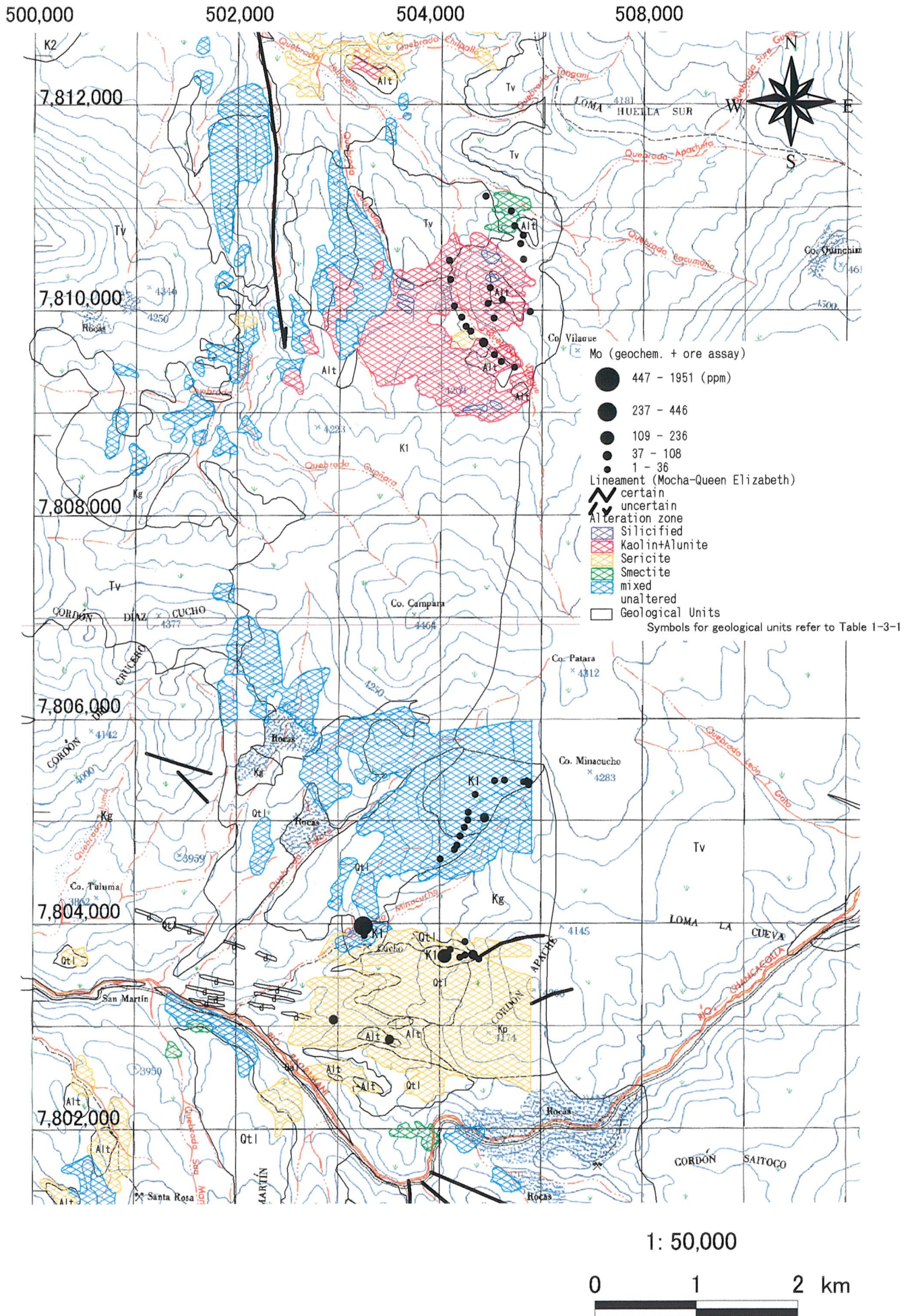
Fig. 2-2-10 (6) Geochemical Anomaly Map in the Queen Elizabeth Area (Mo)
