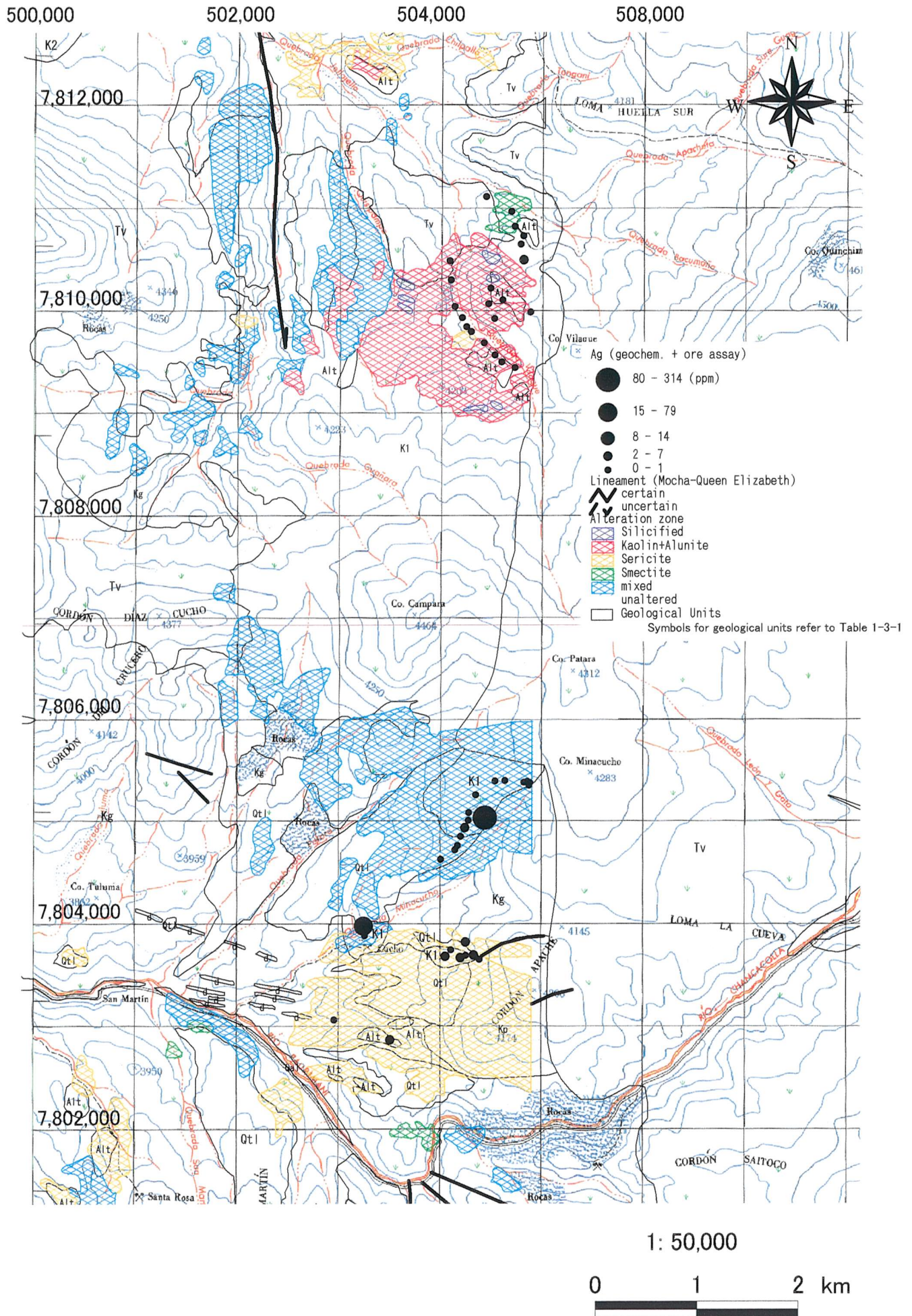
Fig. 2-2-10 (2) Geochemical Anomaly Map in the Queen Elizabeth Area (Ag)
